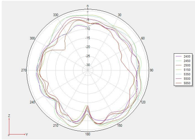
Phi =90 freq=2400MHz
