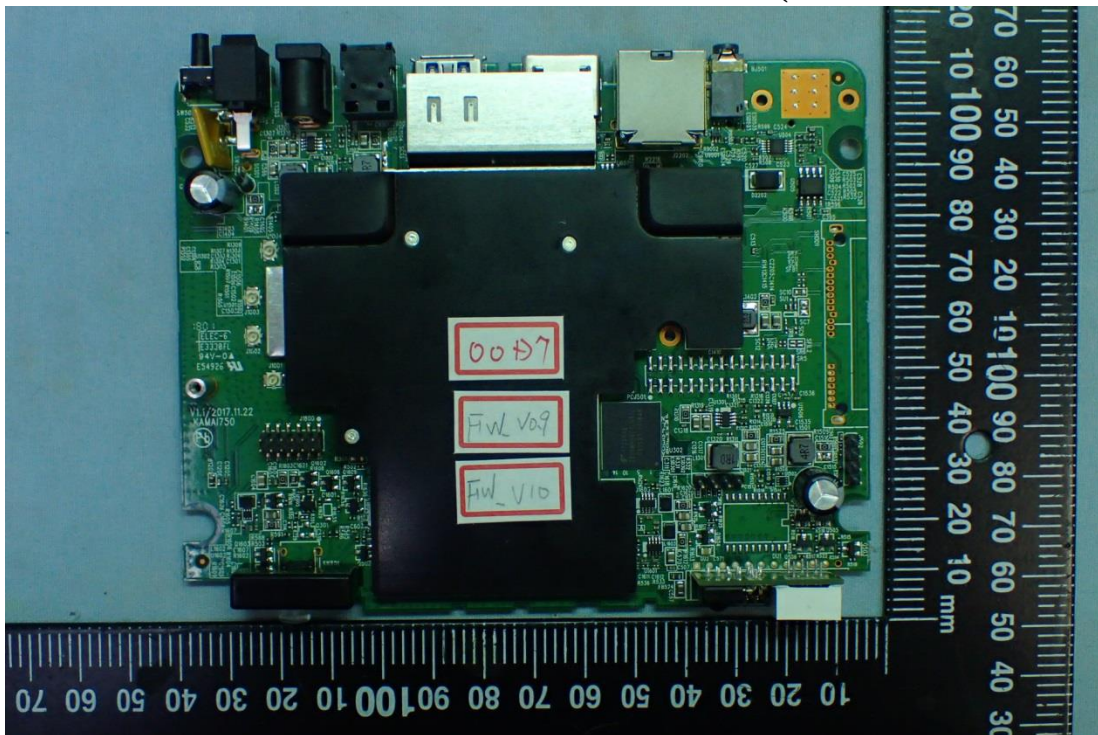
Figure 10 Internal View (Main Board, Front View)
