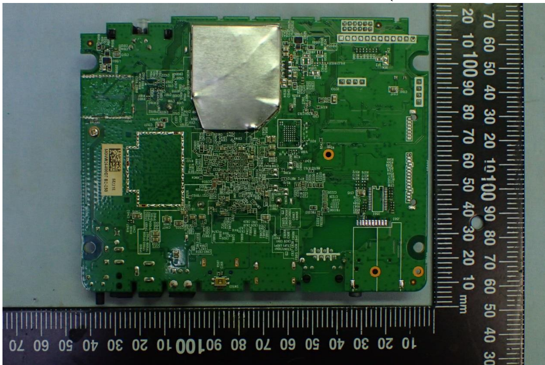
Figure 9 Internal View (Main Board, Back View)
