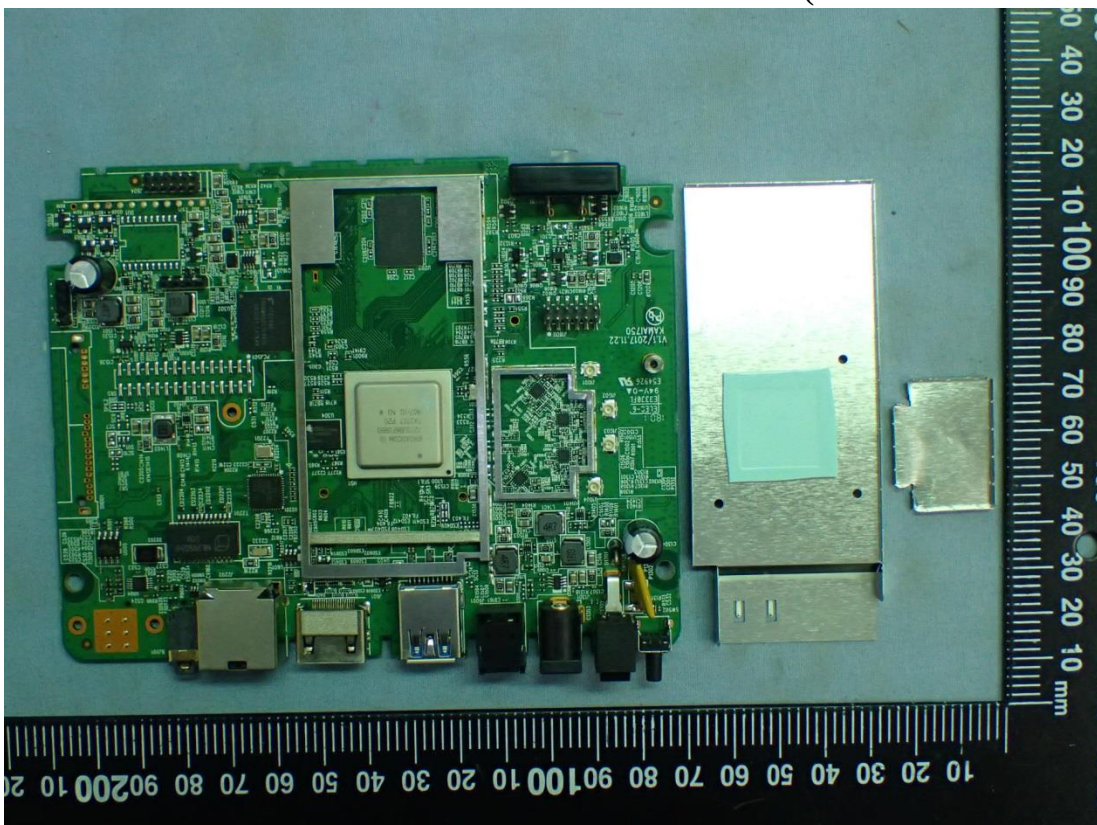
Figure 14 Internal View (Removed Metal Cover)
