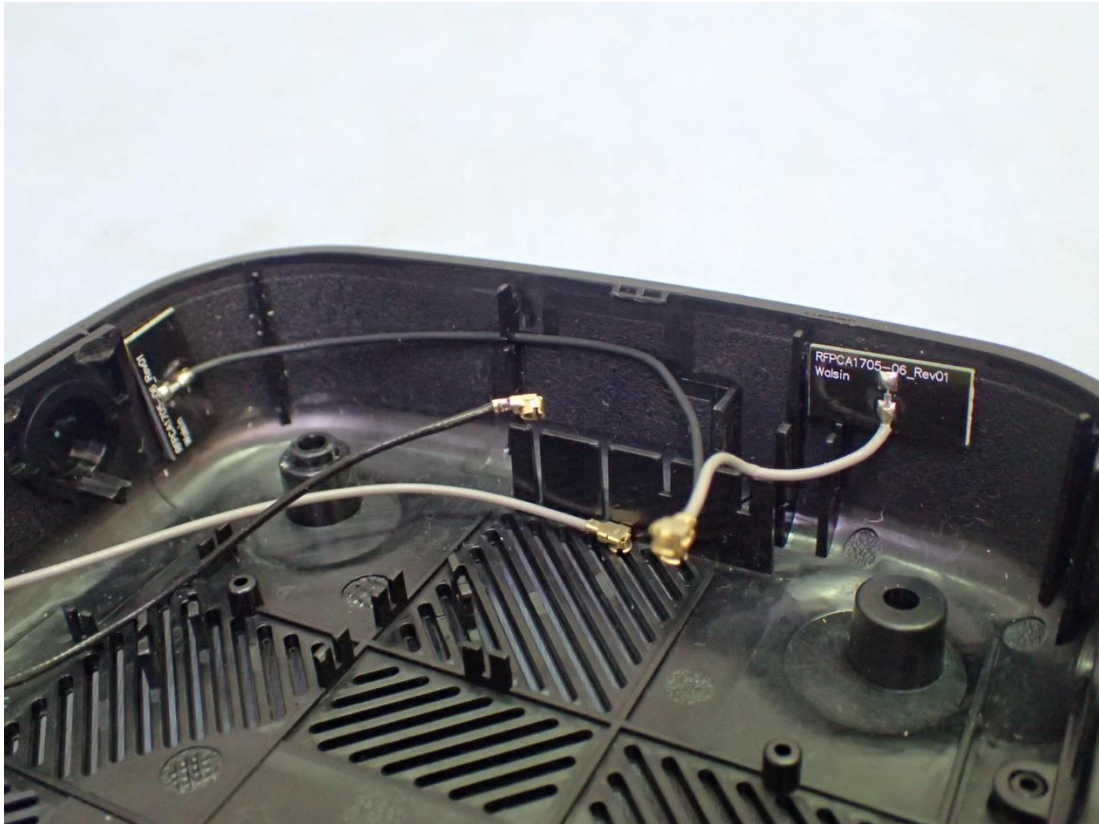
Figure 17 Internal View (WLAN Antenna View)
