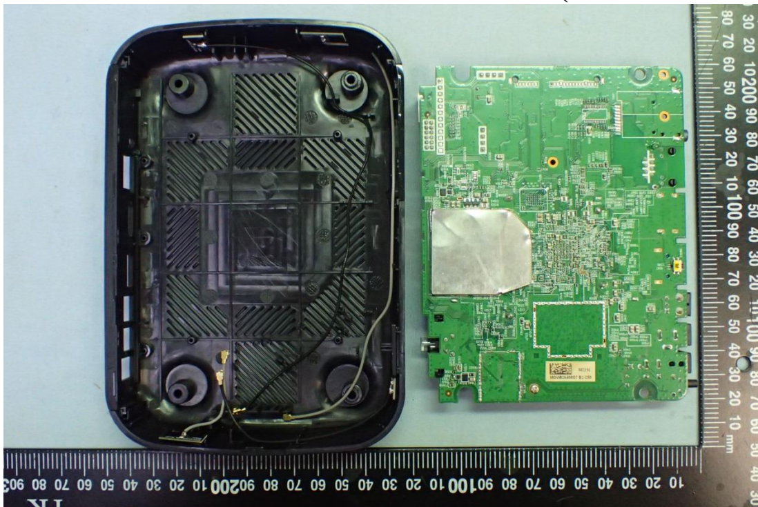
Figure 8 Internal View (Removed Main Board)
