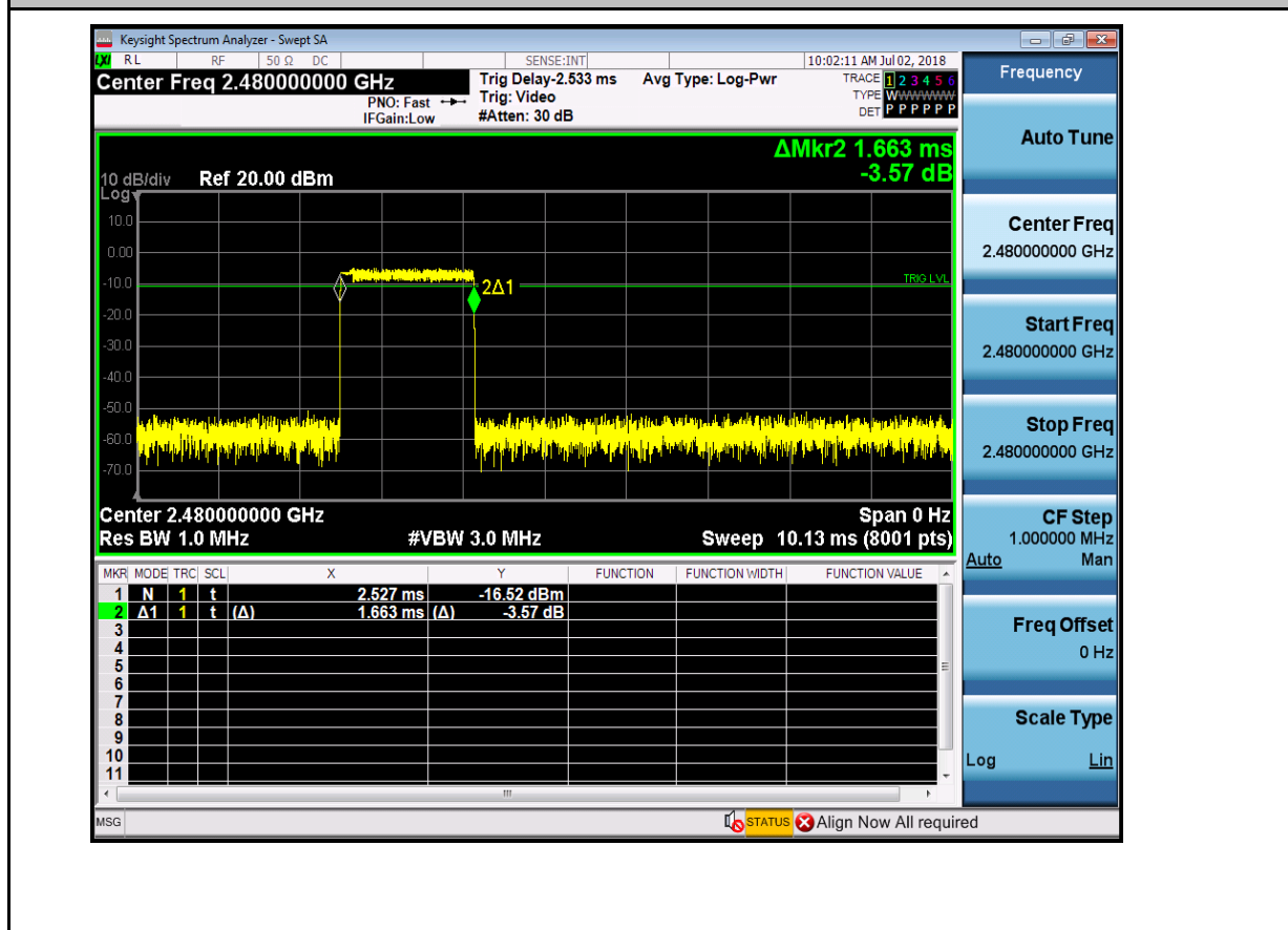
Dwell Time_2DH3_2480
