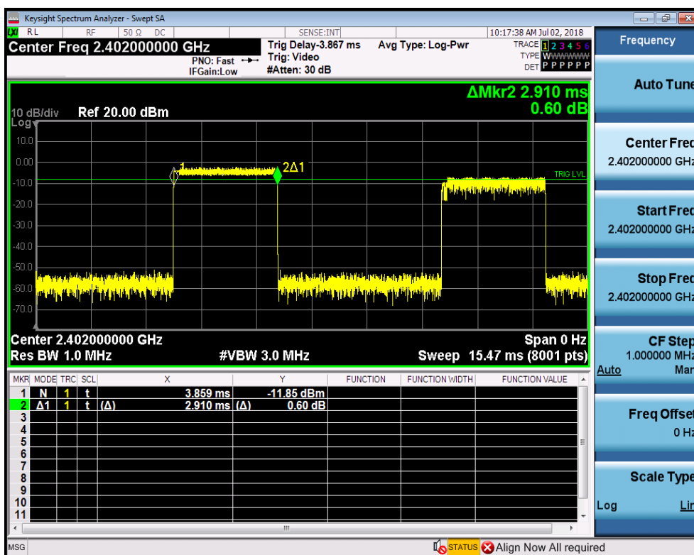
Dwell Time_3DH5_2402
