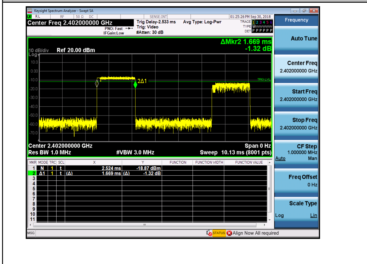
Dwell Time_3DH3_2402
