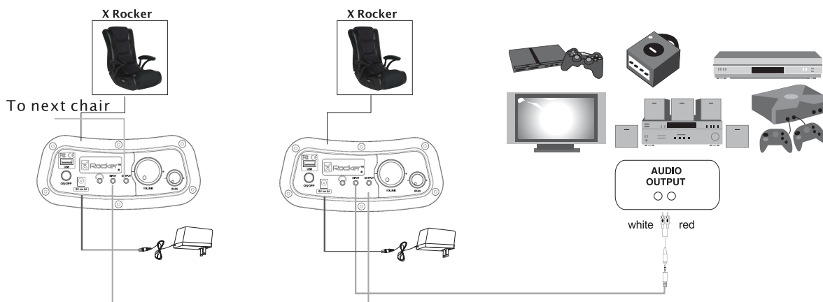
DIAGRAM 4 MULTI-USER CONNECTION
