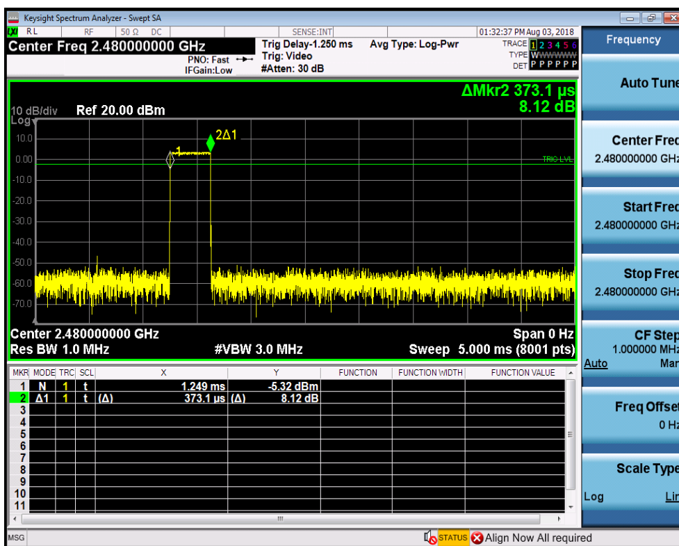
Dwell Time_DH1_2480
