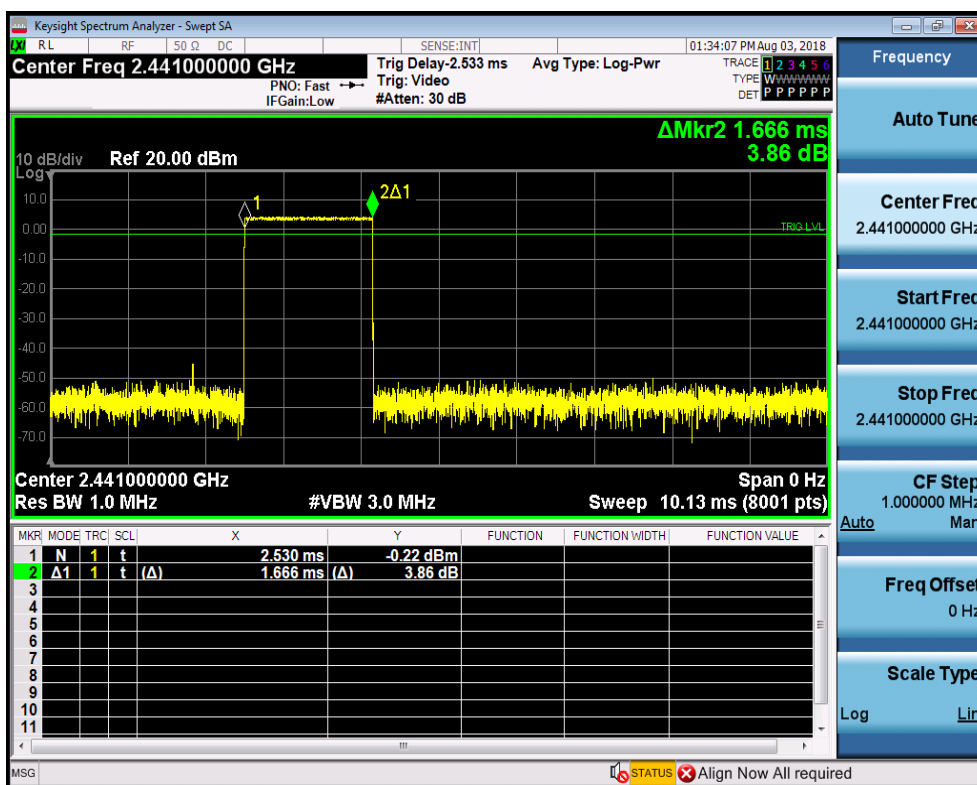
Dwell Time_DH3_2441
