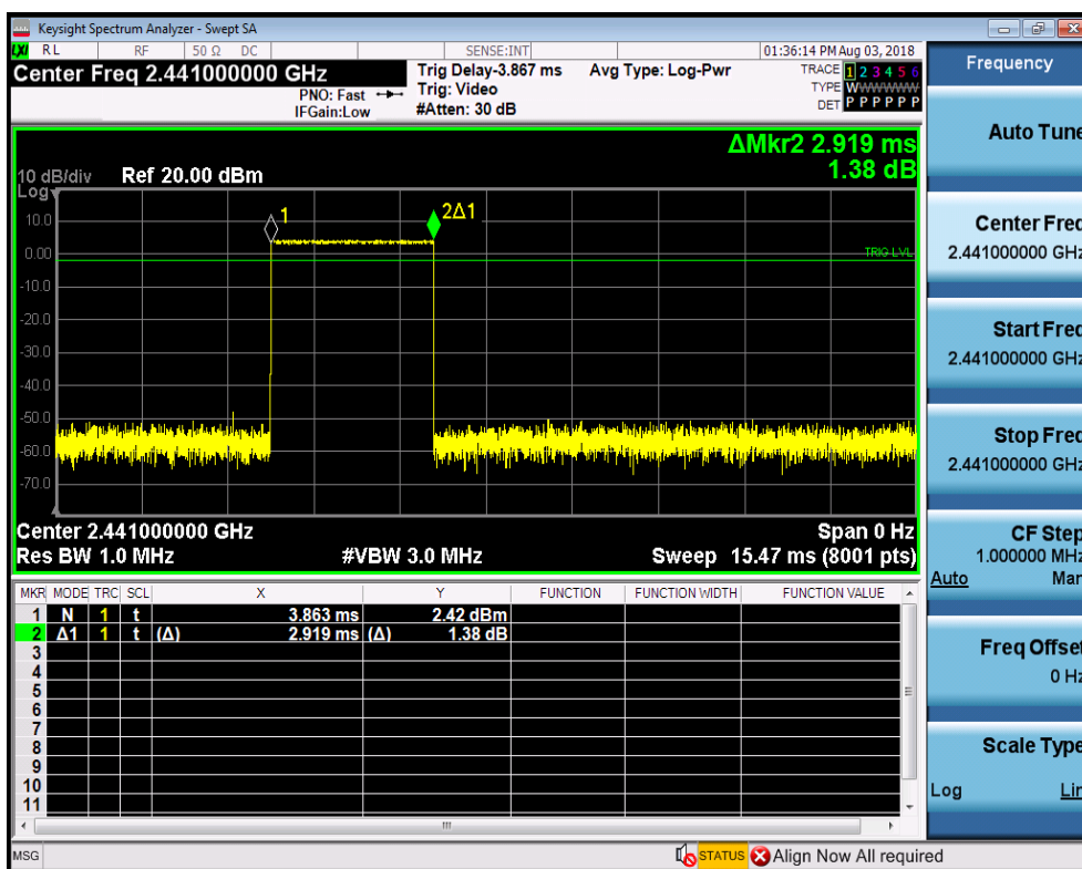
Dwell Time_DH5_2441
