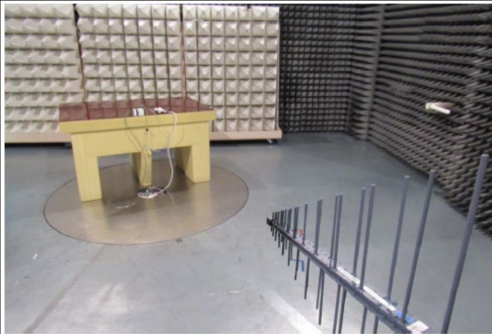
TEST SETUP 2 RADIATED EMISSION
