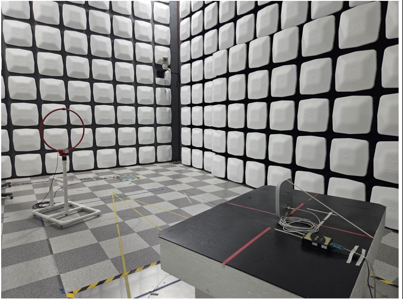
Below 30 MHz
