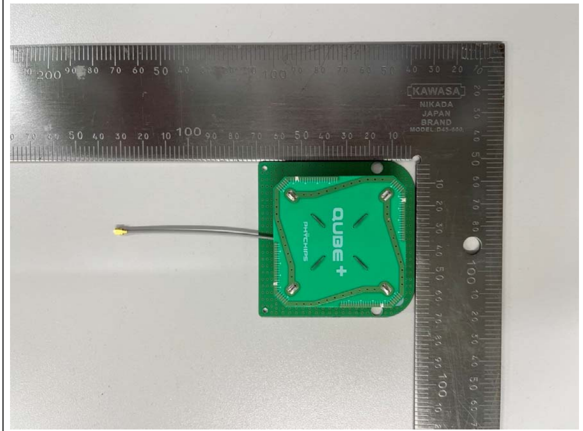
RFID Antenna (M/N: KSA-947A7015B80F)
