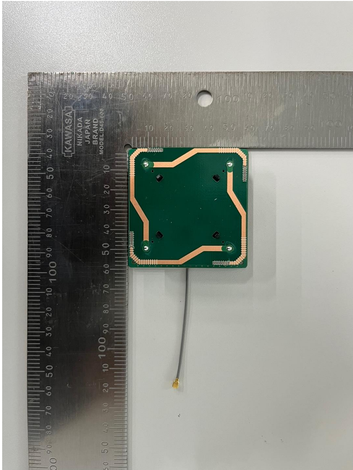
RFID Antenna (M/N: MQWA60F55SM919-A)
