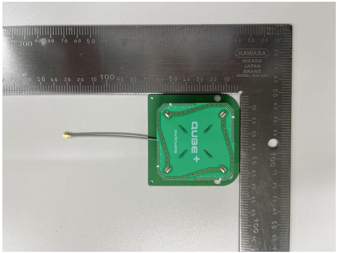
RFID Antenna (M/N: KSA-947A7015B80F)
