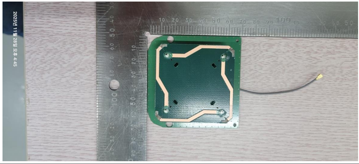
RFID Antenna (M/N: MQWA70F55SP966-A)
