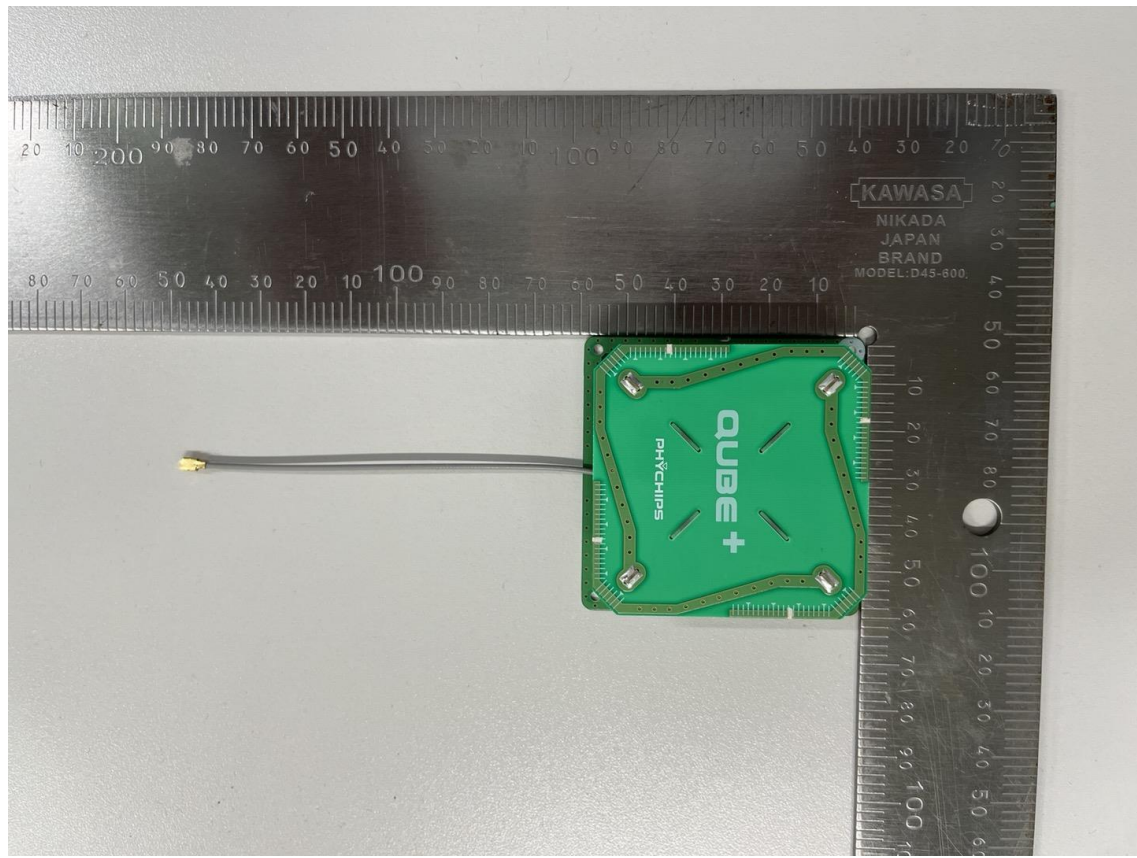
RFID Antenna (M/N: KSA-921A6015B100B)
