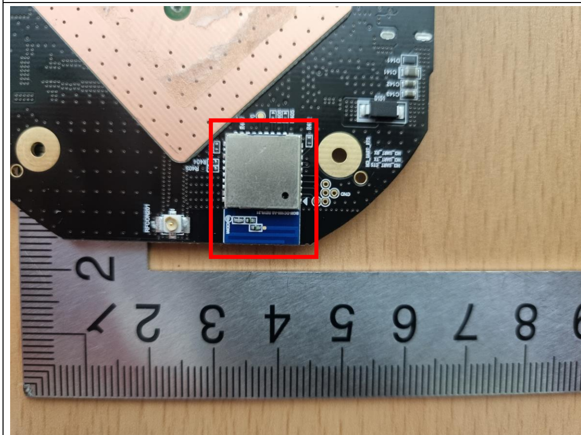
Certified BT Module (FCC ID: 2APDI-BCM-DC100-XS)
