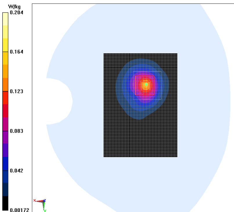
Fig3 WCDMA Band5 Ground Mode Middle
