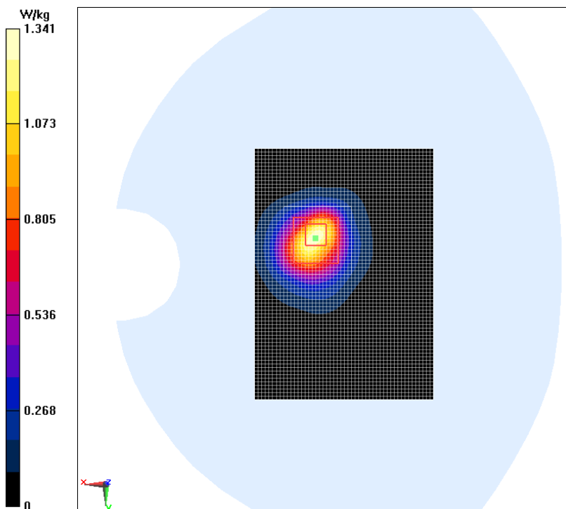
Fig1WCDMA Band2 Ground Mode Low
