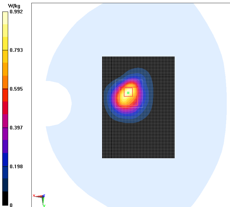
Fig2 WCDMA Band4 Ground Mode High
