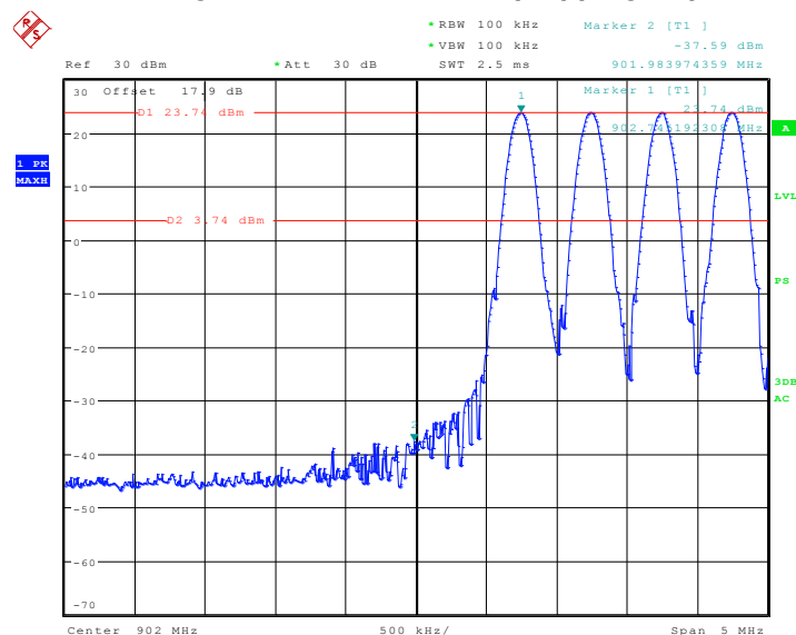
Low Band Edge Plot on Channel 00 (Hopping On)
