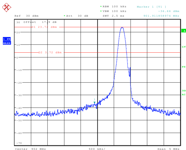
Low Band Edge Plot on Channel 00 (Hopping Off)
