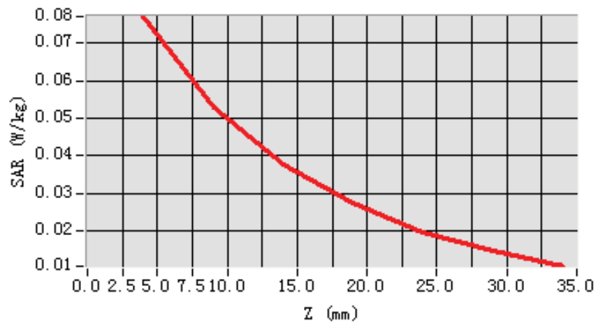
SAR, Z Axis Scan (X = -40, Y = -7)
