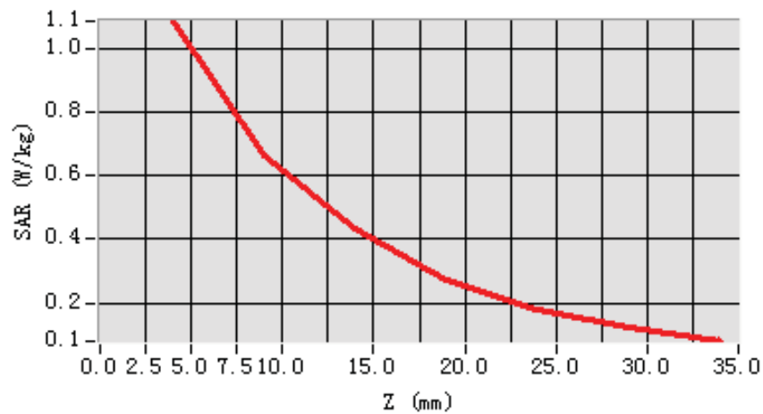
SAR, Z Axis Scan (X = -47, Y = -45)
