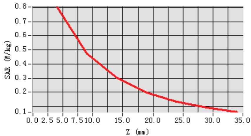
SAR, Z Axis Scan (X = -57, Y = -8)
