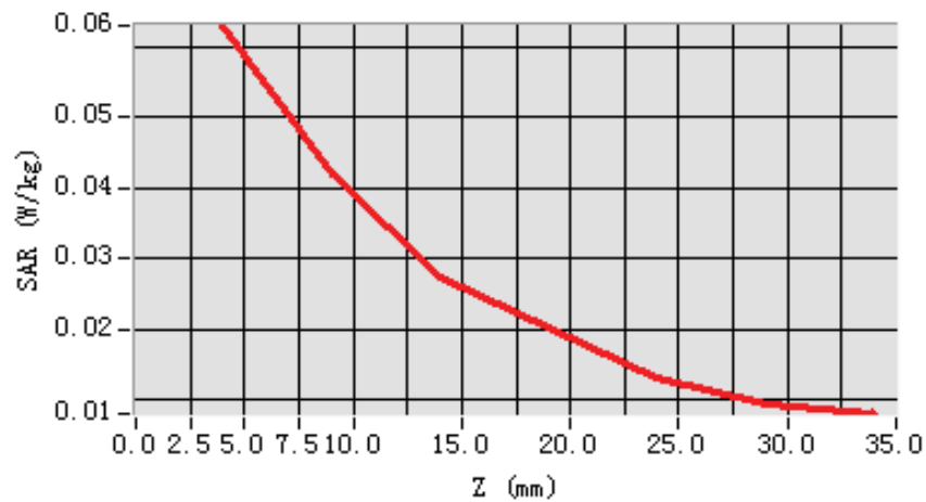
SAR, Z Axis Scan (X = -32, Y = -38)
