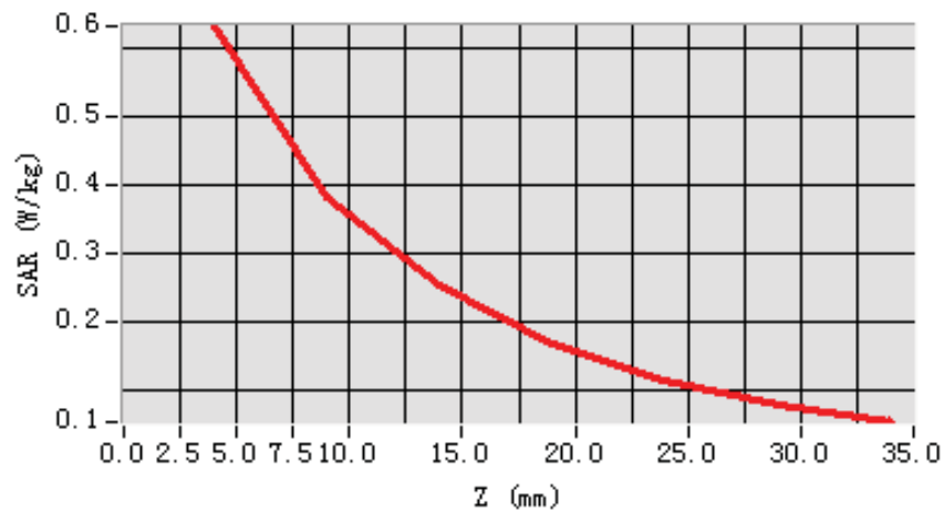
SAR, Z Axis Scan (X = -58, Y = -9)
