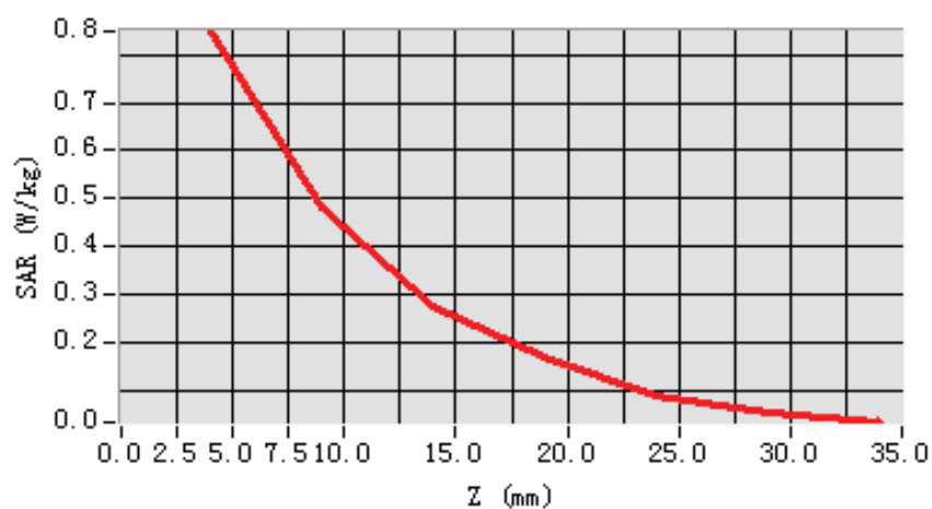
SAR, Z Axis Scan (X = -48, Y = -41)
