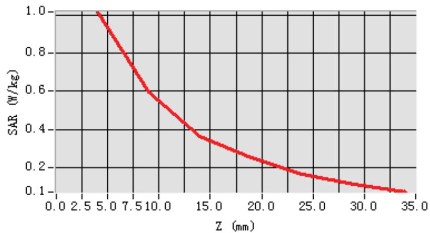
SAR, Z Axis Scan (X = -56, Y = -8)
