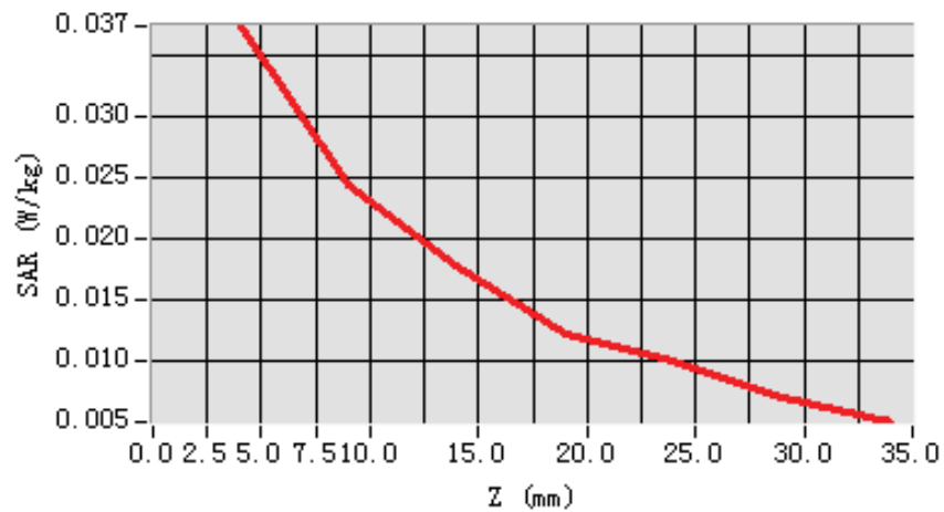
SAR, Z Axis Scan (X = -32, Y = -33)
