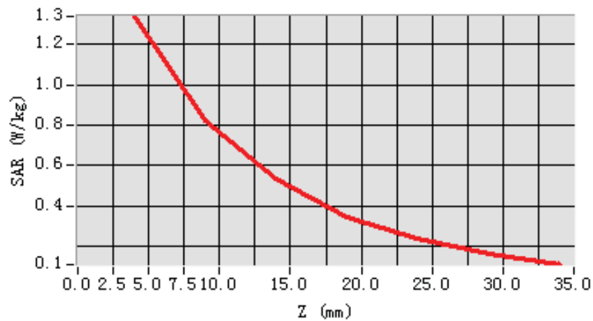
SAR, Z Axis Scan (X = -46, Y = -46)
