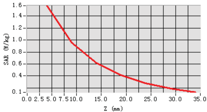
SAR, Z Axis Scan (X = -46, Y = -47)
