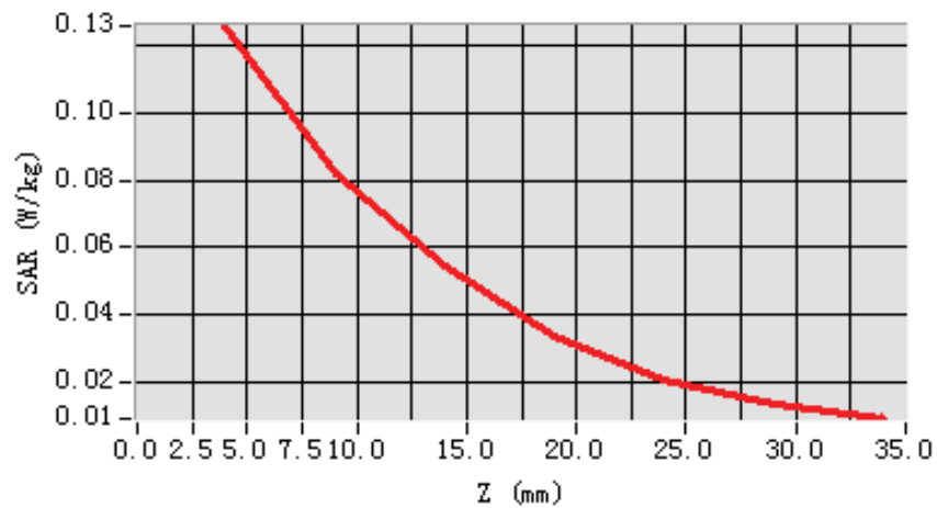
SAR, Z Axis Scan (X = -41, Y = -15)
