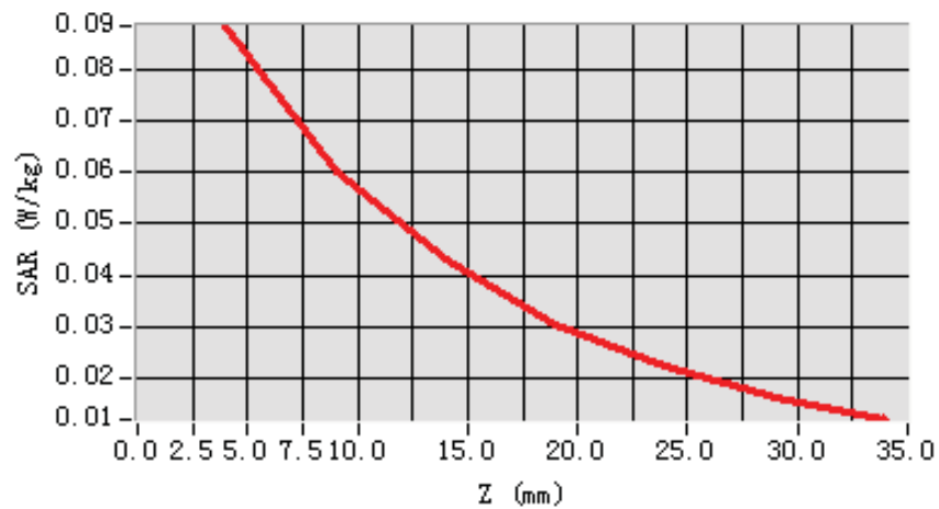
SAR, Z Axis Scan (X = -41, Y = -7)
