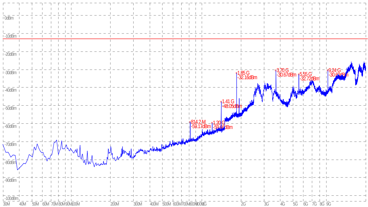
(Plot D.1: GSM 1900MHz Channel = 512, Test Antenna Horizontal)
