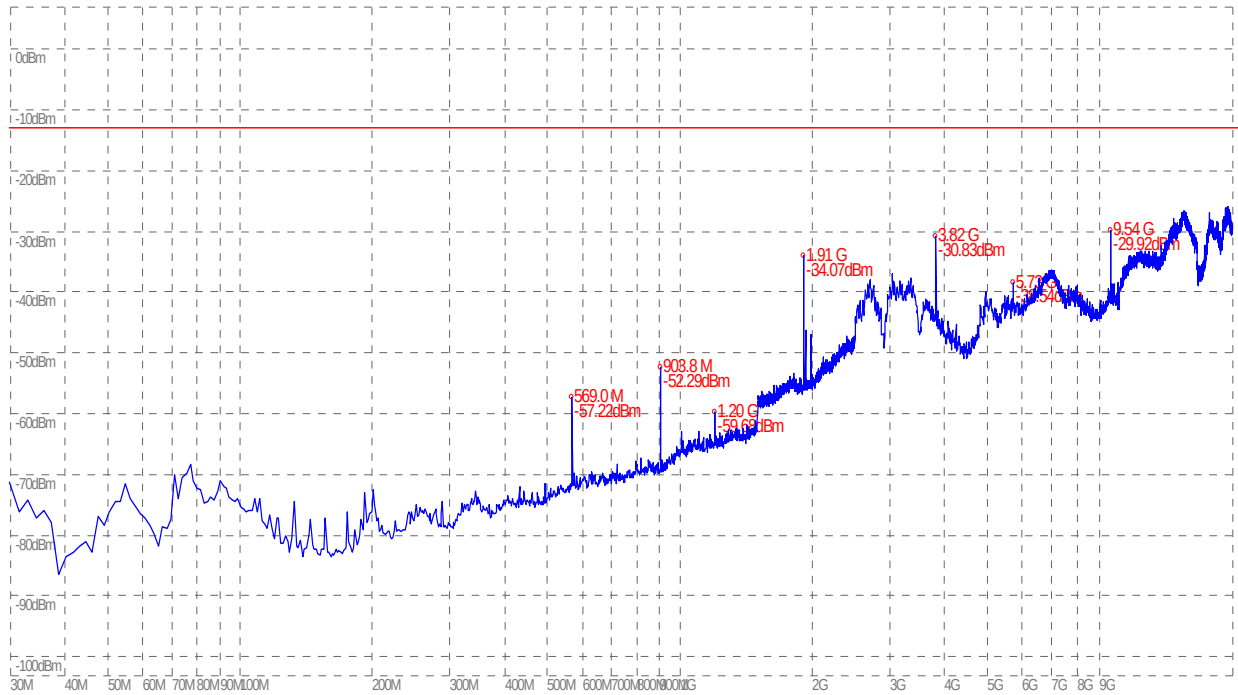
(Plot F.1: GSM 1900MHz Channel = 810, Test Antenna Horizontal)
