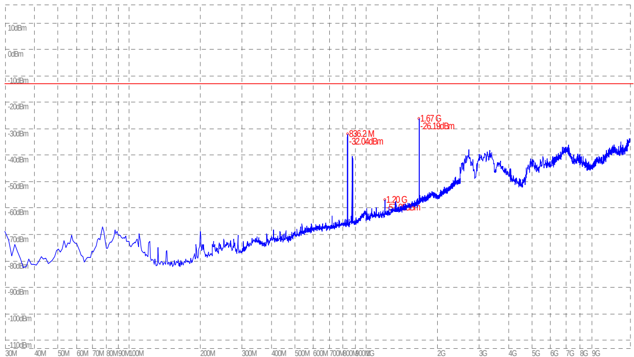
(Plot B.2: GSM 850MHz Channel = 190, Test Antenna Vertical)
