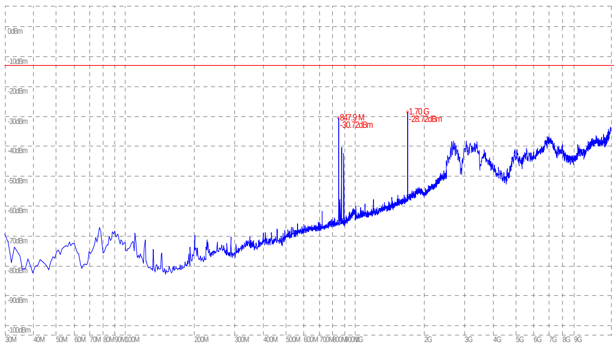
(Plot C.2: GSM 850MHz Channel = 251, Test Antenna Vertical)
