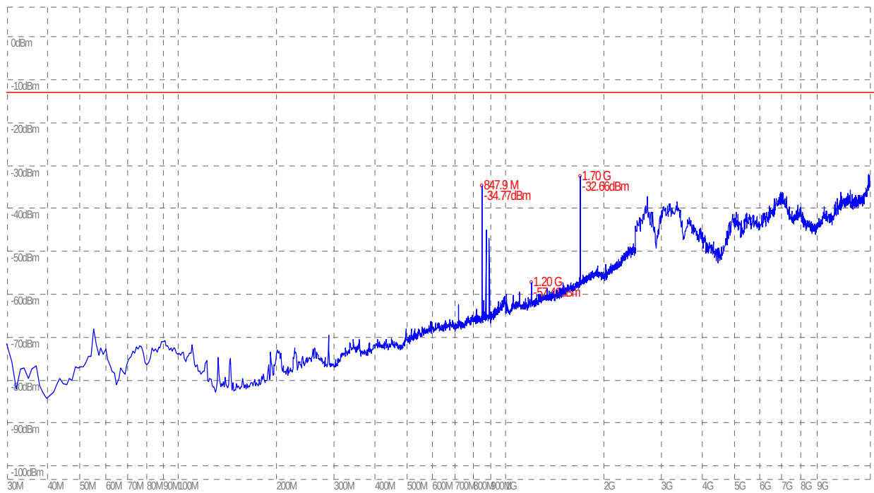
(Plot C.1: GSM 850MHz Channel = 251, Test Antenna Horizontal)
