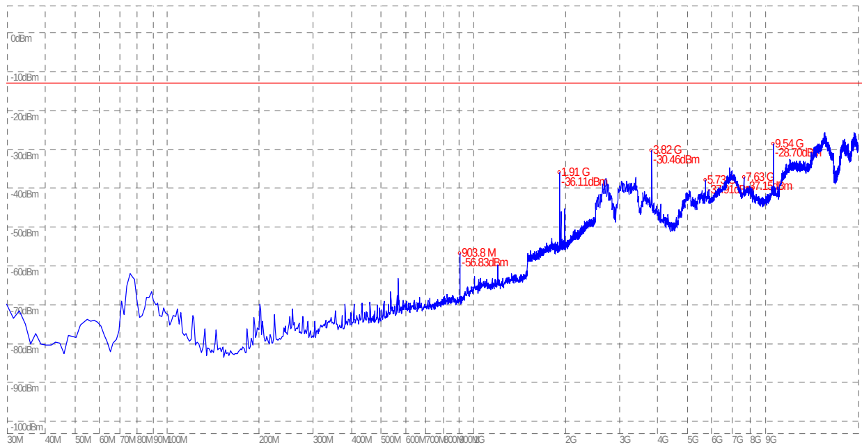
(Plot F.2: GSM 1900MHz Channel = 810, Test Antenna Vertical)
