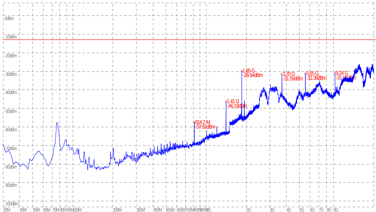
(Plot D.2: GSM 1900MHz Channel = 512, Test Antenna Vertical)
