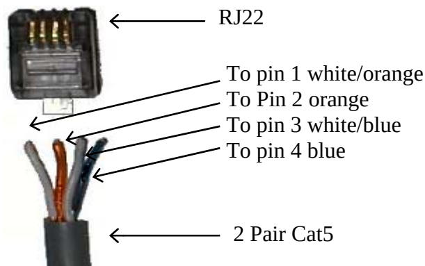
Figure 32 Timing cable wiring pin out
