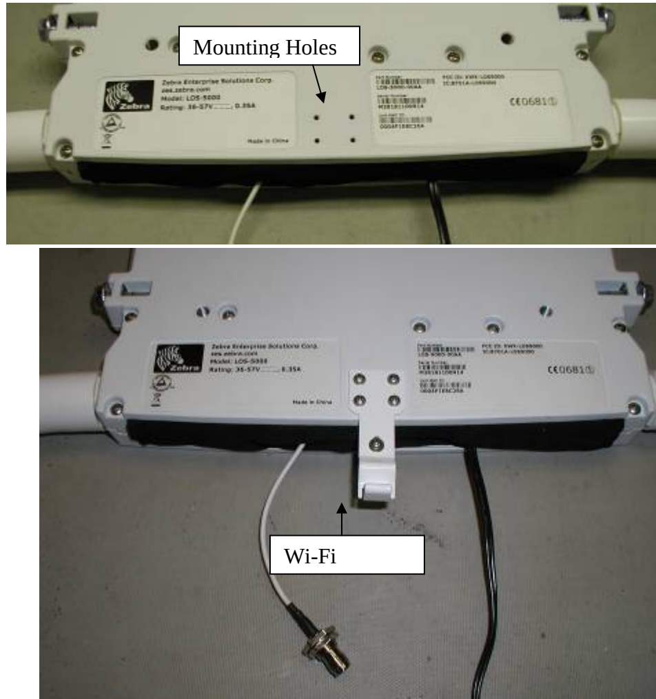
Figure 27 Wi-Fi Bracket
