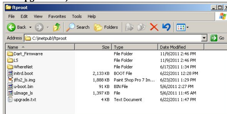
Figure 41 Ftproot Directory
