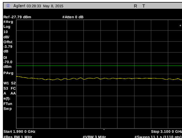
Plot 17. Radiated Emissions Above 960 MHz, 1990 MHz – 3100 MHz, Average, 2mbps IC Limit
