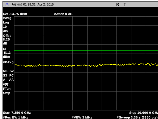
Plot 30. Radiated Emissions Above 960 MHz, 7250 MHz – 10600 MHz, Average, 2mbps
