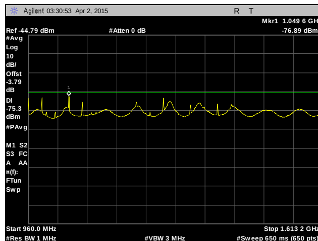
Plot 25. Radiated Emissions Above 960 MHz, 960 MHz – 1610 MHz, Average, 2mbps
