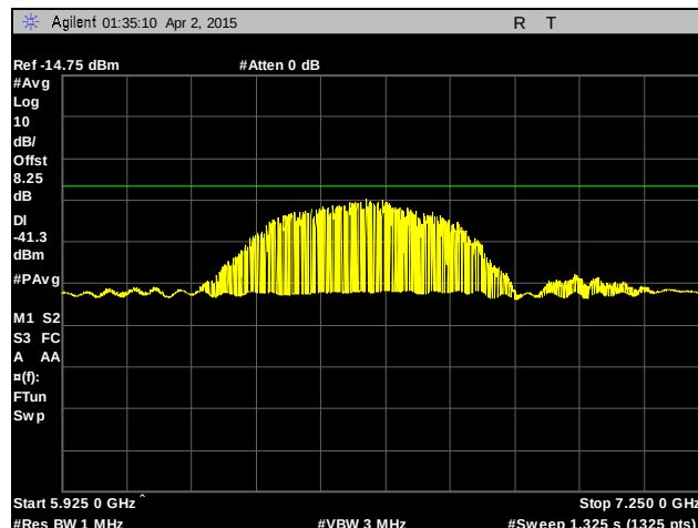
Plot 29. Radiated Emissions Above 960 MHz, 5925 MHz – 7250 MHz, Average, 2mbps
