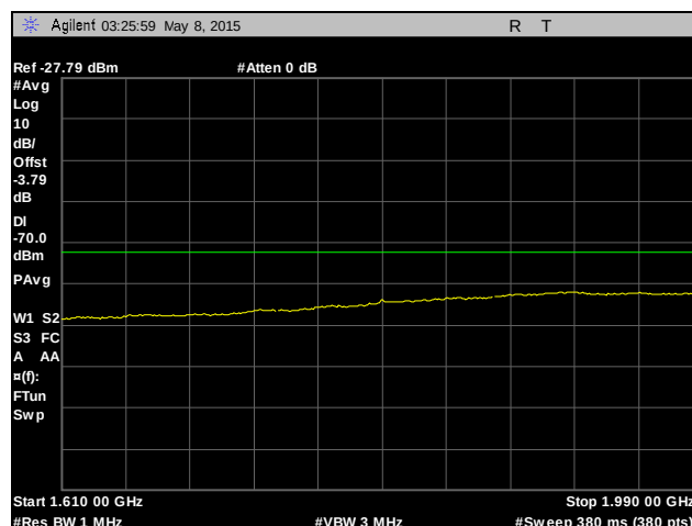
Plot 14. Radiated Emissions Above 960 MHz, 1610 MHz – 1990 MHz, Average, 1mbps IC Limit
