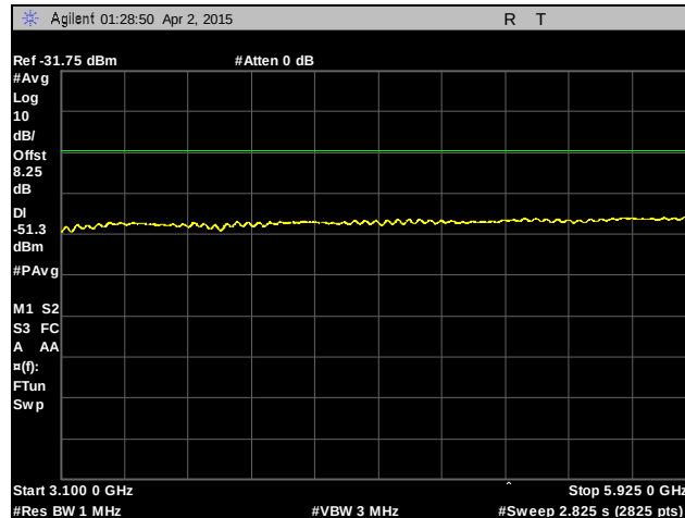
Plot 21. Radiated Emissions Above 960 MHz, 3100 MHz – 5925 MHz, Average, 1mbps
