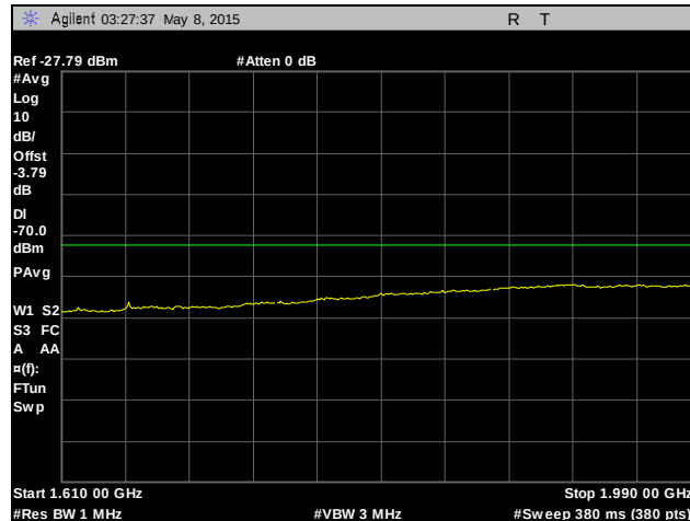
Plot 15. Radiated Emissions Above 960 MHz, 1610 MHz – 1990 MHz, Average, 2mbps IC Limit
