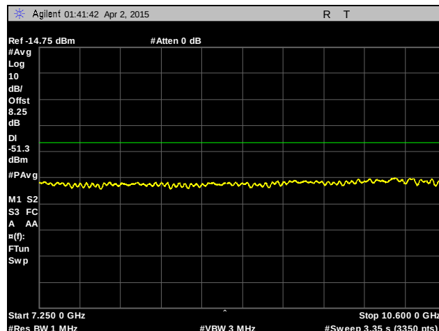
Plot 23. Radiated Emissions Above 960 MHz, 7250 MHz – 10600 MHz, Average, 1mbps
