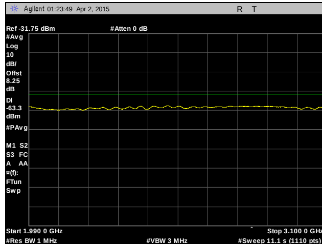
Plot 27. Radiated Emissions Above 960 MHz, 1990 MHz – 3100 MHz, Average, 2mbps
