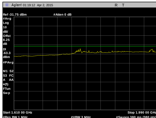
Plot 26. Radiated Emissions Above 960 MHz, 1610 MHz – 1990 MHz, Average, 2mbps
