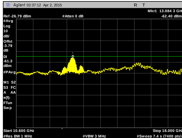
Plot 24. Radiated Emissions Above 960 MHz, 10600 MHz – 18000 MHz, Average, 1mbps
