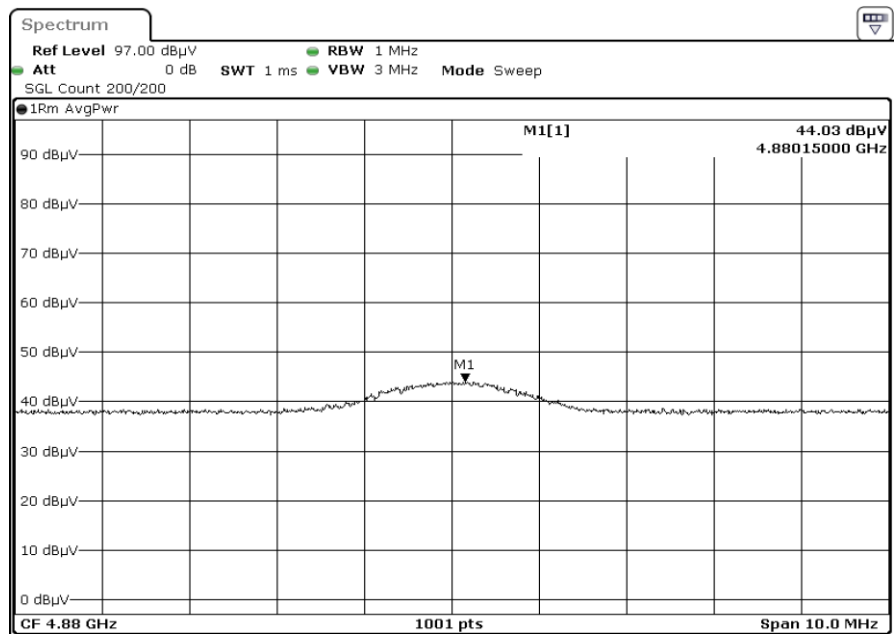
F2 X2 4880.0 Harmonic Vertical AVG
