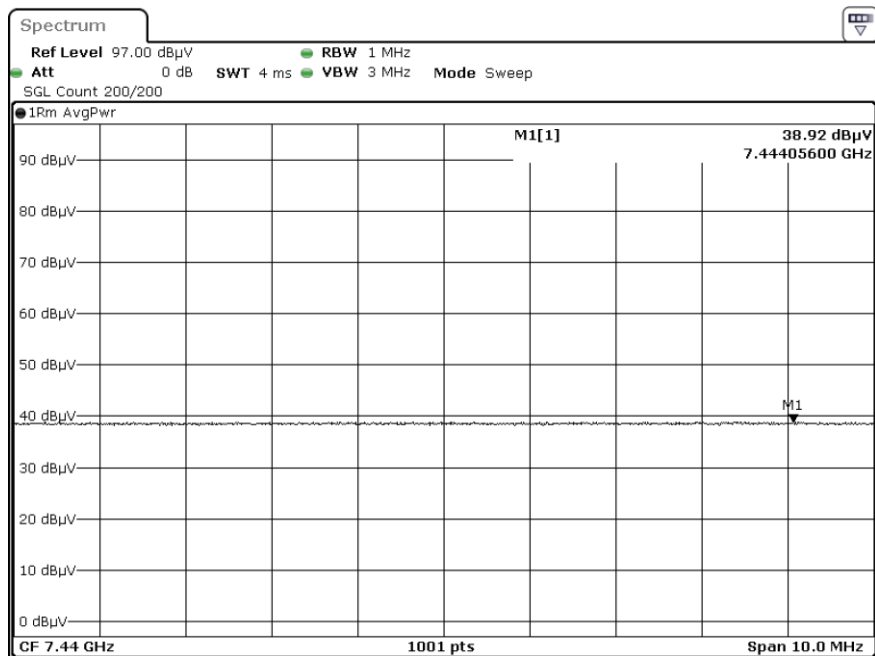
F3 X3 7440.0 Harmonic Horizontal AVG
