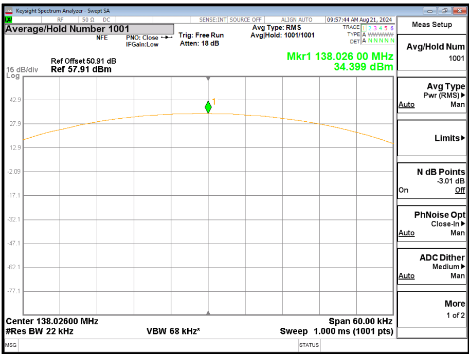
Figure 49 - 138.025 MHz
