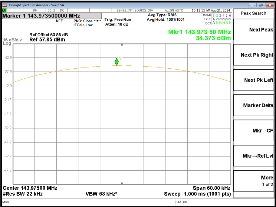
Figure 50 143.975 MHz
