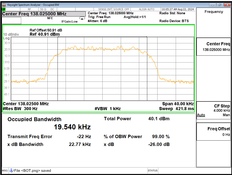
Figure 56 - 138.025 MHz
