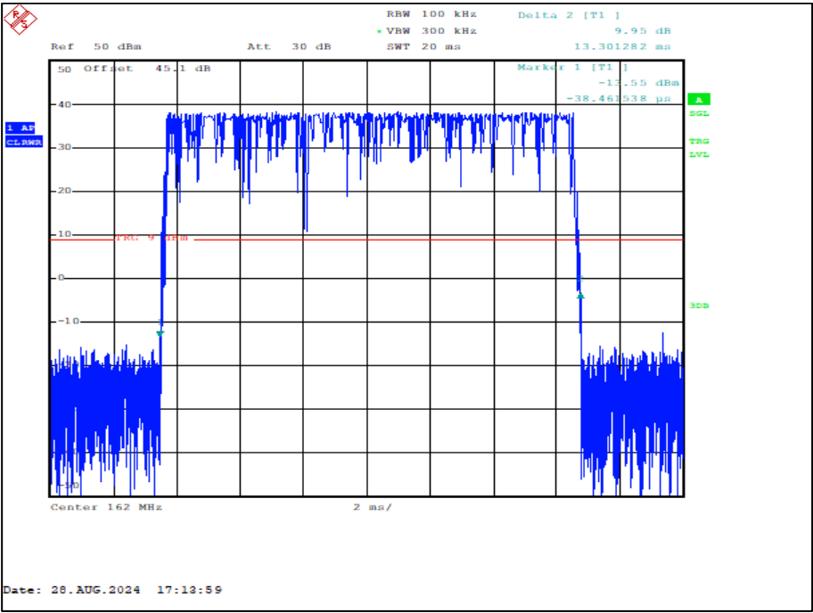
Figure 115-Burst Length
