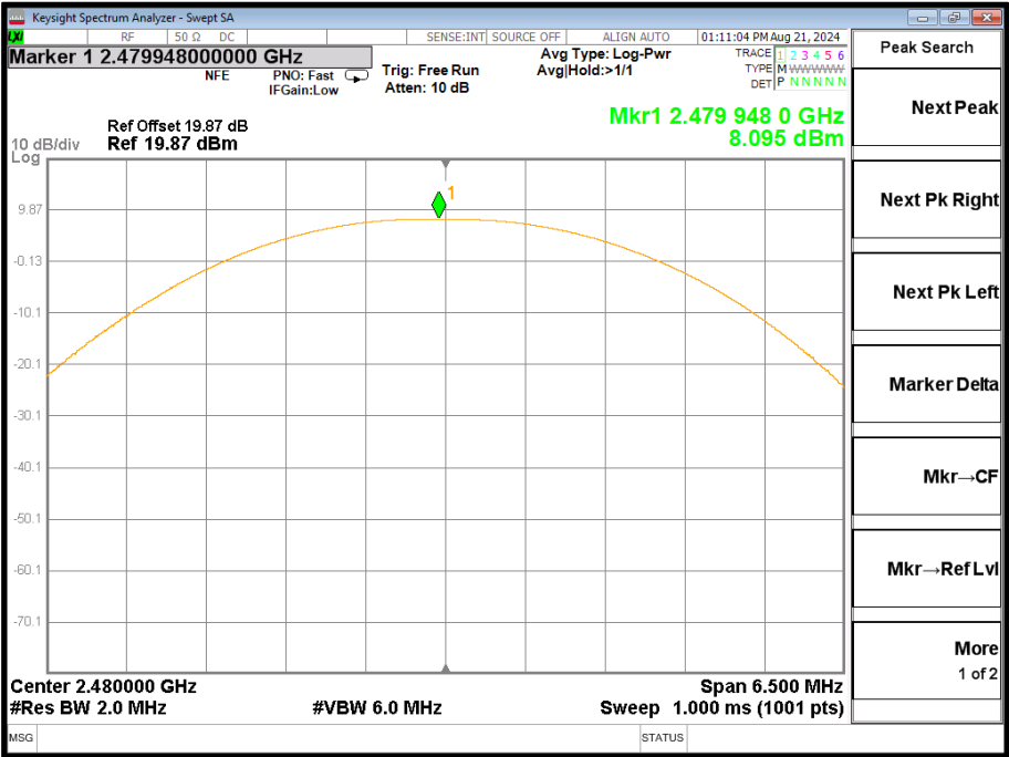
Figure 3 - 2480 MHz, GFSK
