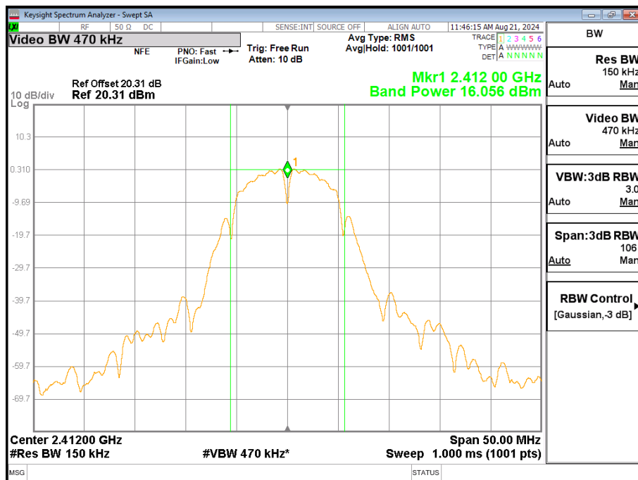
Figure 4 - 2412 MHz (CH1)
