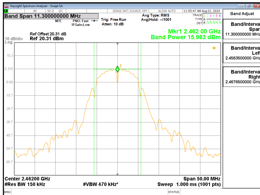
Figure 6 - 2462 MHz (CH11)
