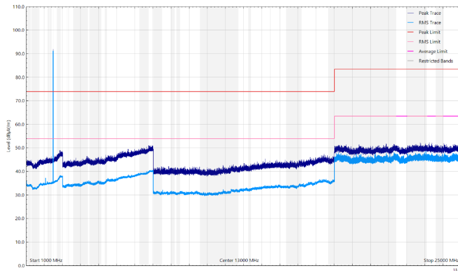
Figure 20 - CH78_3DH5_EDR_3MBPS, 2480 MHz, 1 to 25 GHz, Horizontal, Z Orientation - Peak / Average
