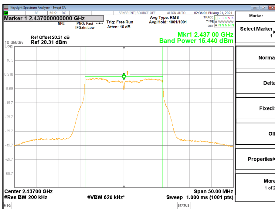
Figure 11 - 2437 MHz (CH6)
