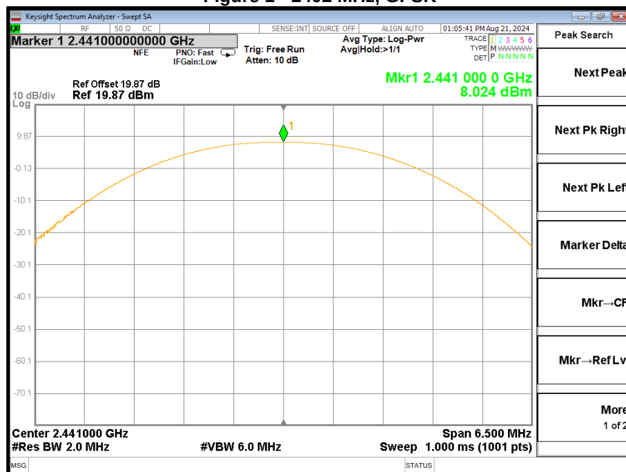
Figure 2 - 2441 MHz, GFSK
