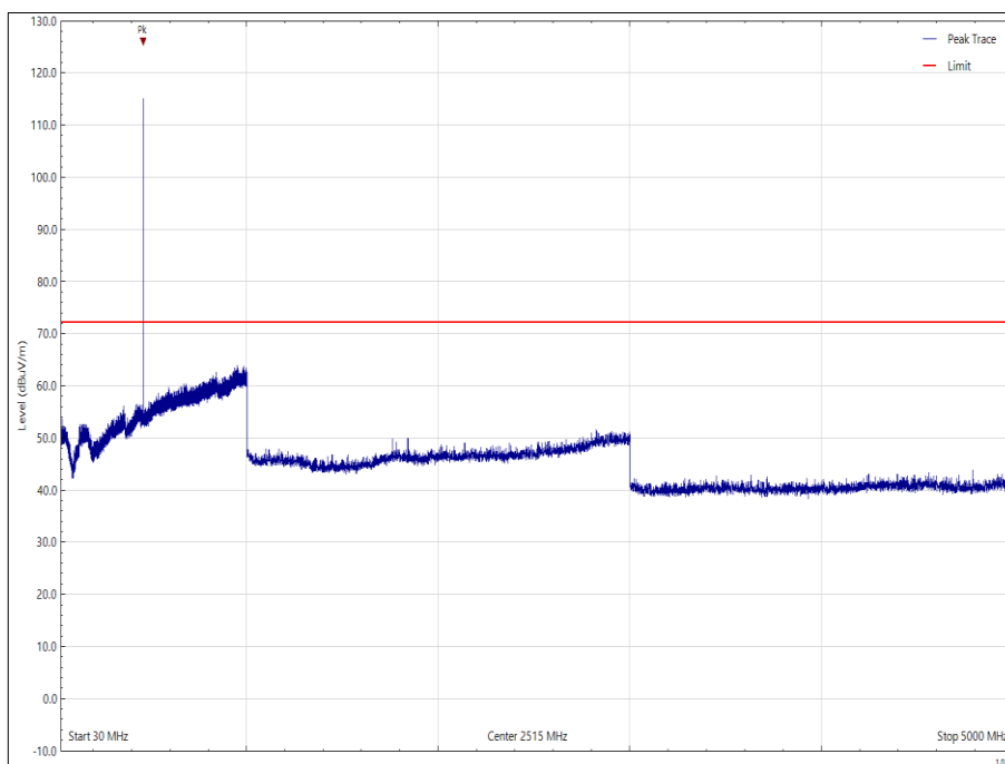
Figure 83 – 460.025 MHz - 30 MHz to 5 GHz, Horizontal, EUT Orientation X
