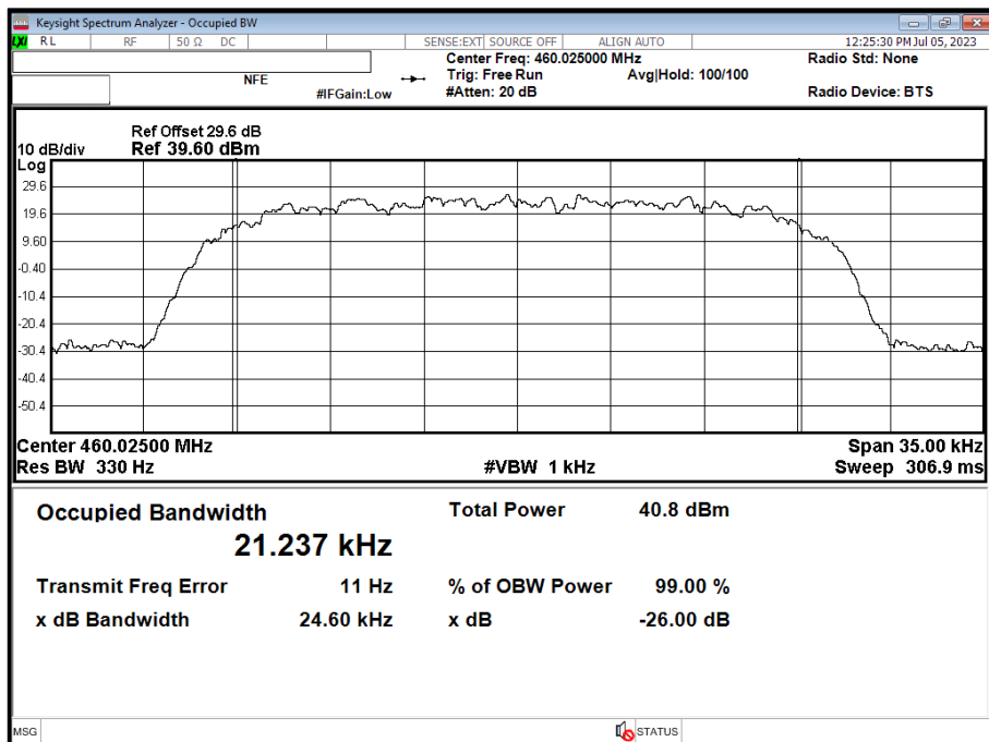
Figure 17 - 460.025 MHz
