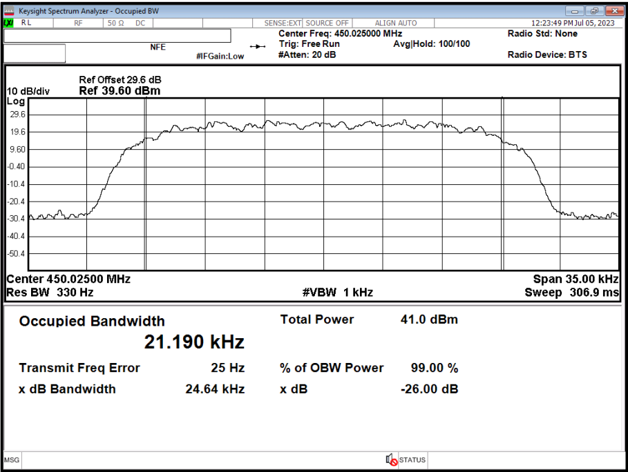
Figure 16 - 450.025 MHz
