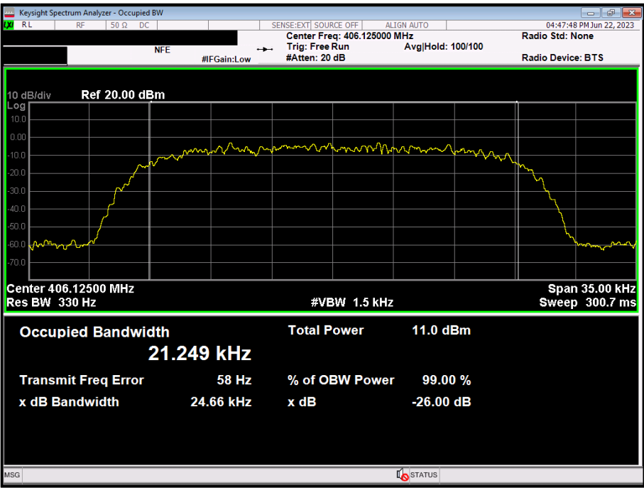
Figure 13 - 406.125 MHz
