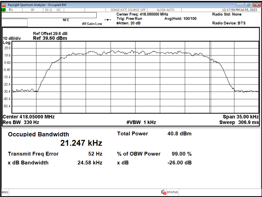
Figure 14 - 418.050 MHz
