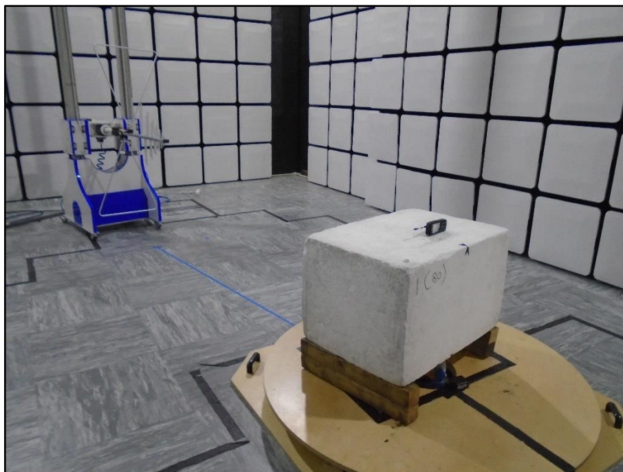
Figure 110 – Test Setup, 30 MHz to 1 GHz X Orientation
