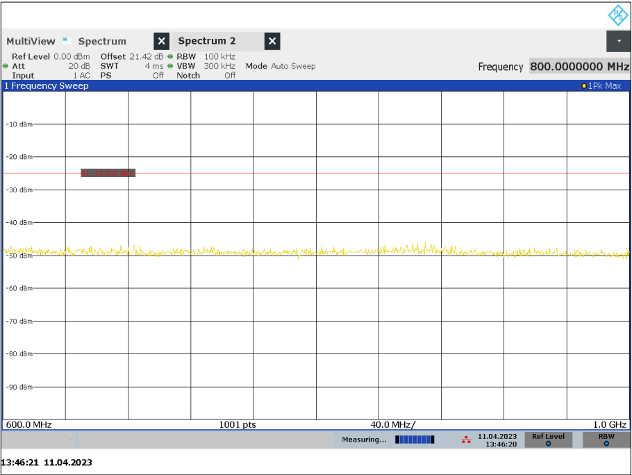
Figure 32 - 418.050 MHz, 600 MHz to 1 GHz Mask Y
