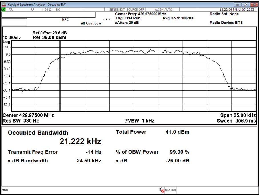
Figure 15 - 429.975 MHz
