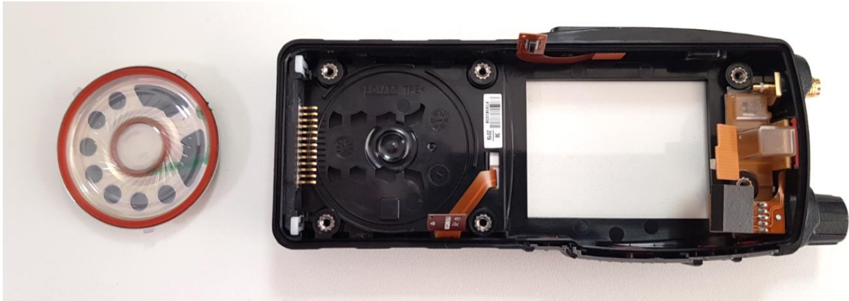
Figure 28. SC2028 Front Cover with Speaker Removed New Version
