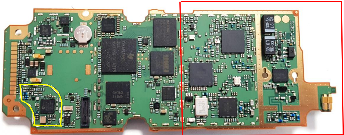
Figure 17. SC2028 Main PCB Bottom View With Cans Removed Old Version
