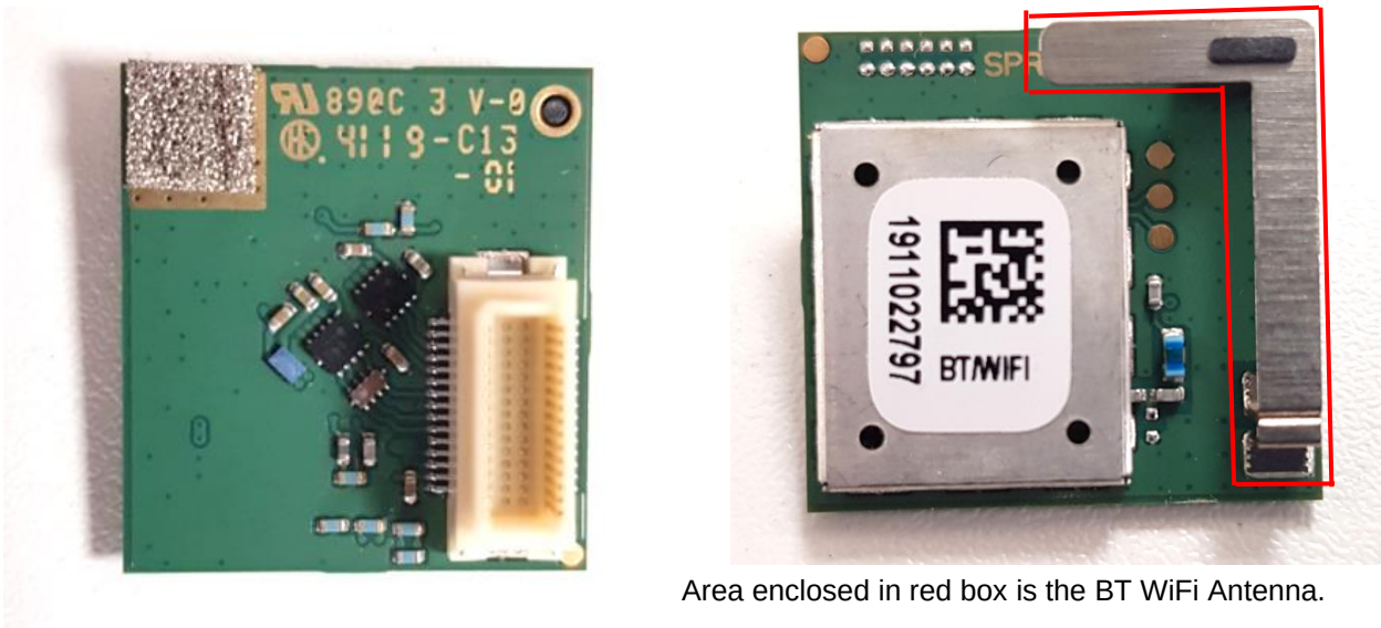
Figure 29. SC2028 Bluetooth Module Old Version
