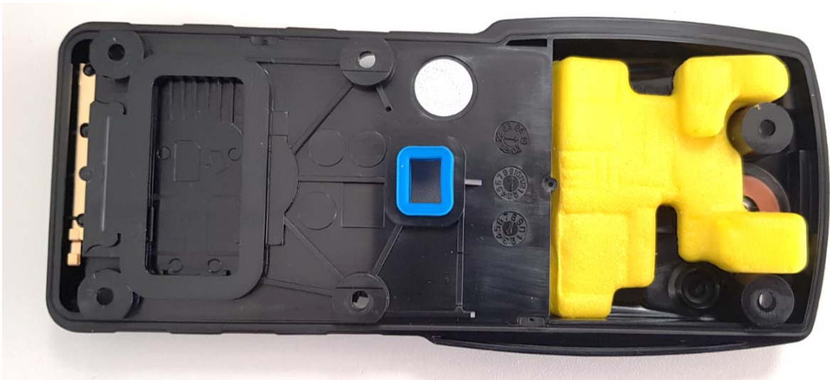
Figure 8. SC2028 Main Rear Cover New Version
