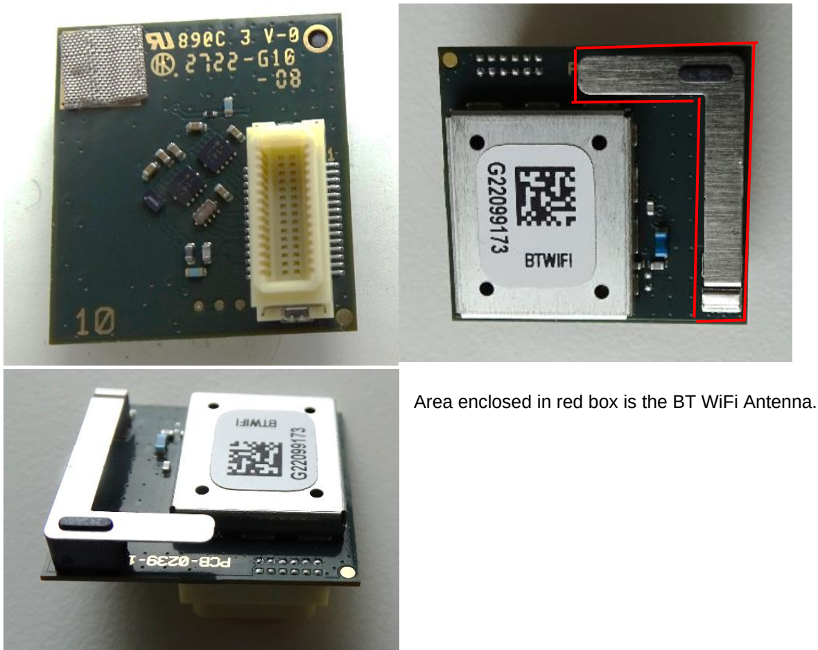
Figure 30. SC2028 Bluetooth Module New Version
