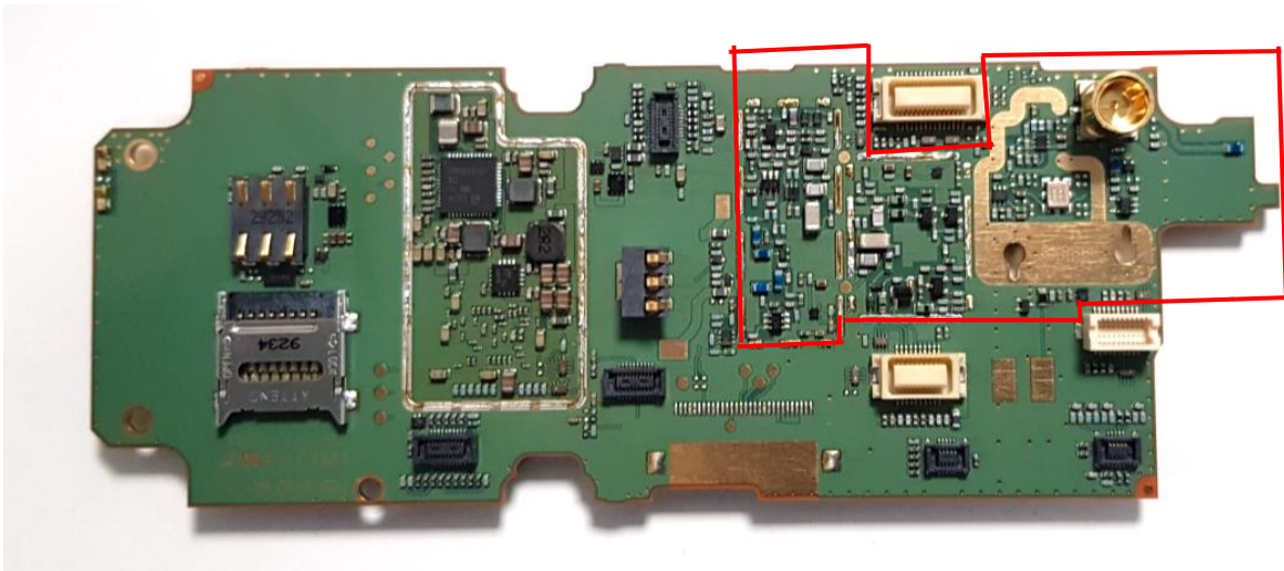
Figure 15. SC2028 Main PCB Top View With Cans Removed Old Version
