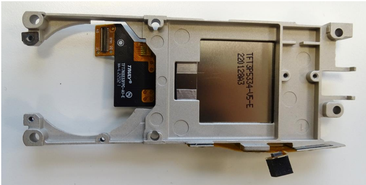
Figure 22. SC2028 LCD Side Rear View New Version
