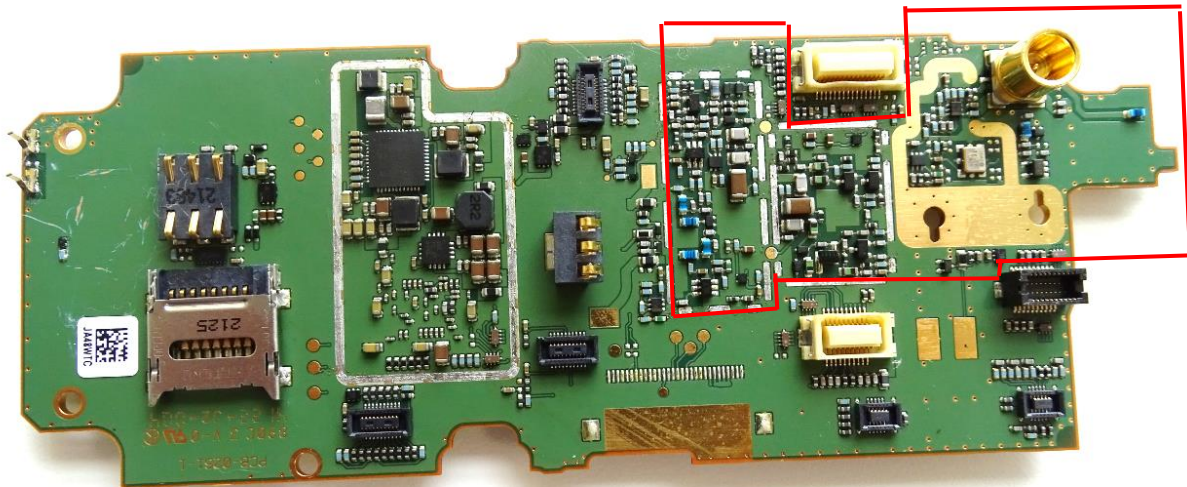
Figure 16. SC2028 Main PCB Top View With Cans Removed New Version
