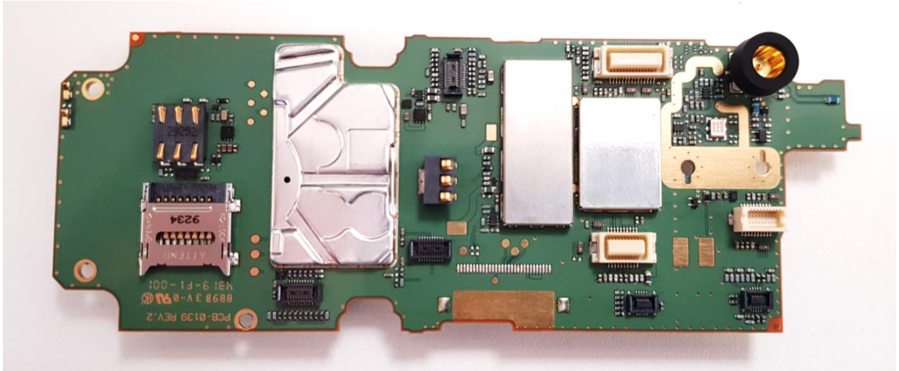
Figure 12. SC2028 Main PCB Top View New Version
