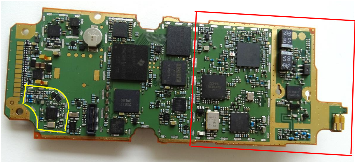
Figure 18. SC2028 Main PCB Bottom View With Cans Removed New Version
