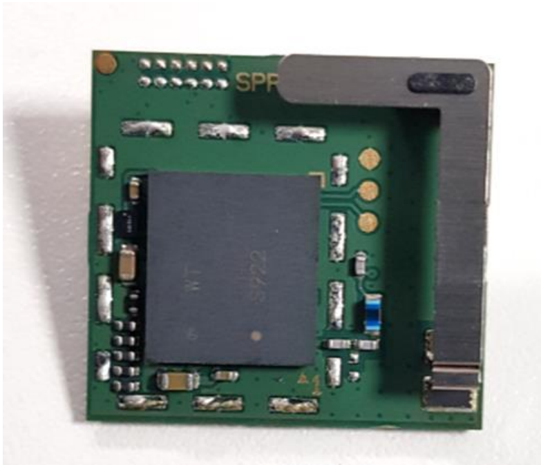
Figure 31. SC2028 Bluetooth Module with Can Removed
