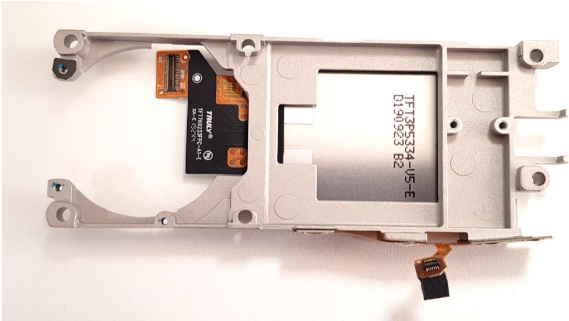
Figure 22. SC2028 LCD Side Rear View New Version
