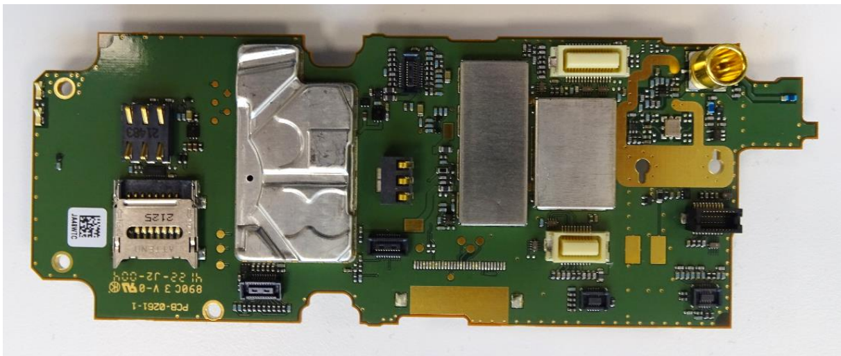
Figure 12. SC2028 Main PCB Top View New Version
