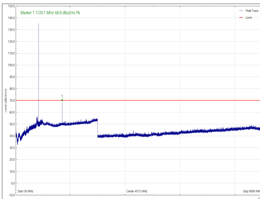
Figure 96 - 860.000 MHz, 30 MHz to 9 GHz, EUT Orientation: Z, Horizontal (Peak)
