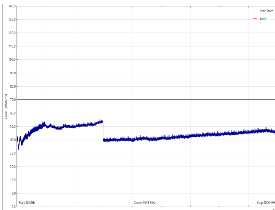
Figure 97 - 860.000 MHz, 30 MHz to 9 GHz, EUT Orientation: Z, Vertical (Peak)
