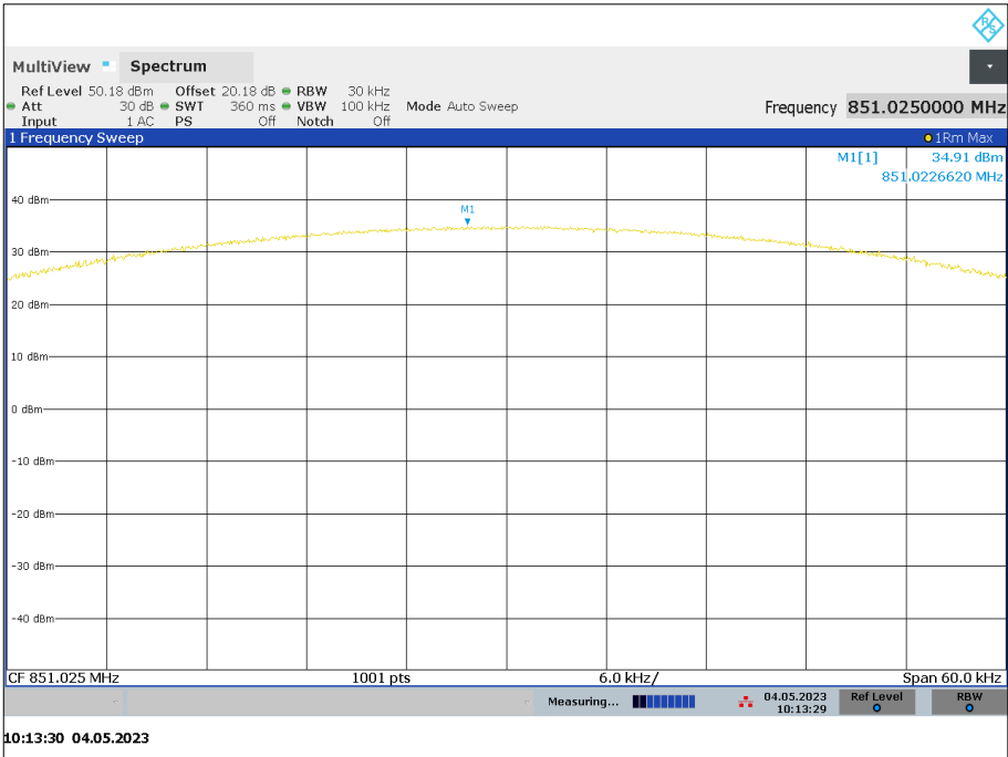
Figure 4 - 851.025 MHz
