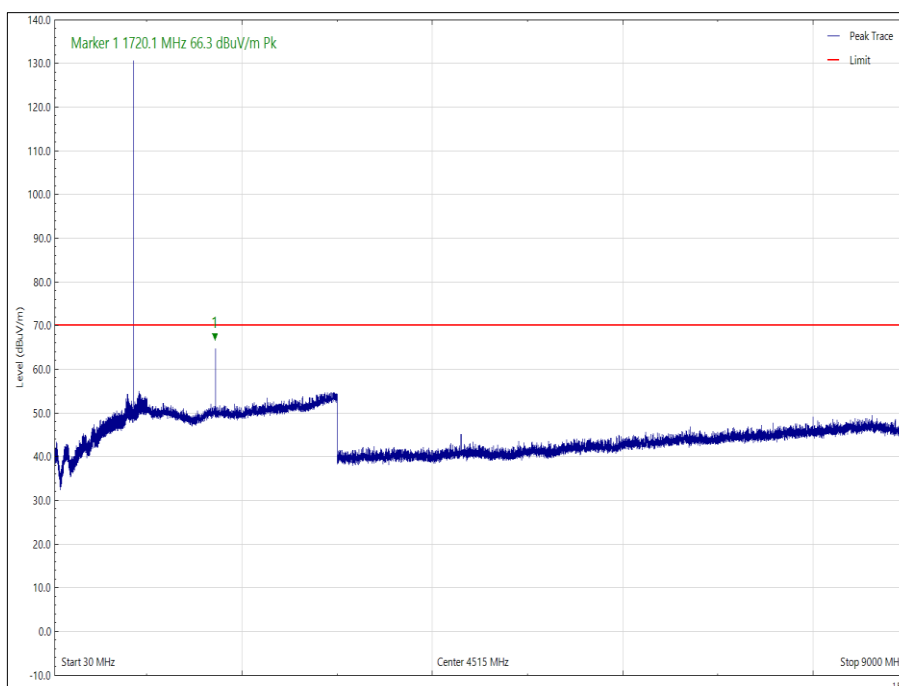
Figure 95 - 860.000 MHz, 30 MHz to 9 GHz, EUT Orientation: Y, Vertical (Peak)
