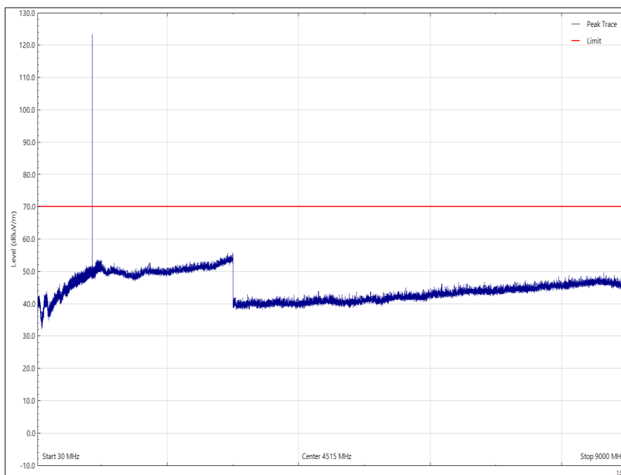
Figure 94 - 860.000 MHz, 30 MHz to 9 GHz, EUT Orientation: Y, Horizontal (Peak)
