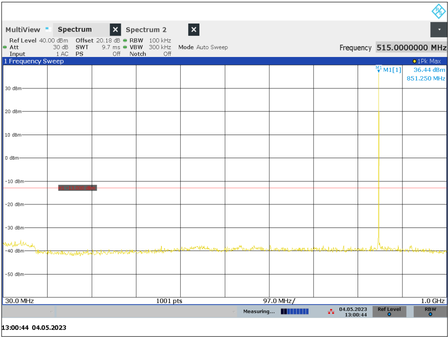
Figure 49 - 851.025 MHz, 30 MHz to 1 GHz Mask B
