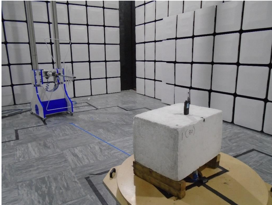
Figure 106 – Test Setup – 30 MHz to 1 GHz Z Orientation
