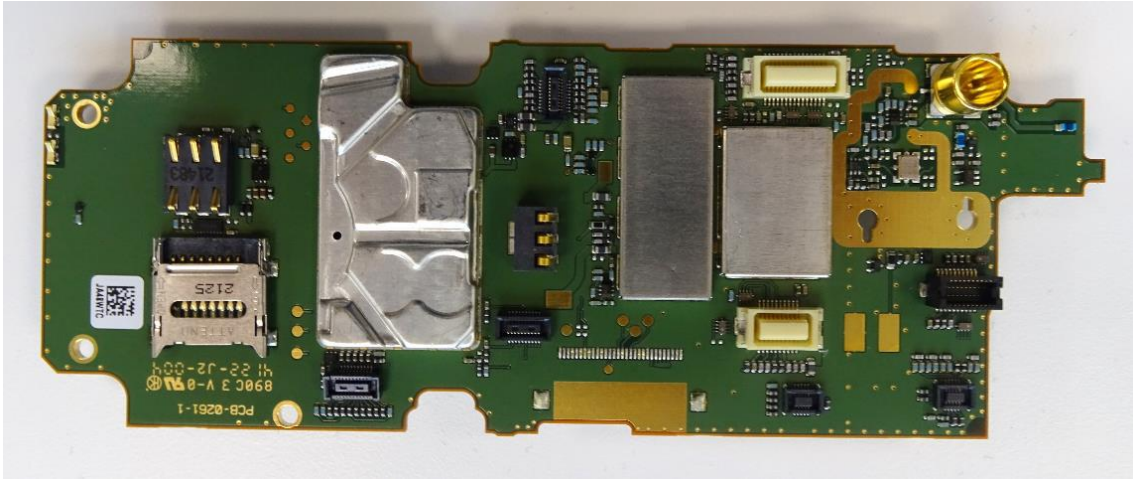
Figure 14 SC2328 MAIN PCB TOP VIEW
