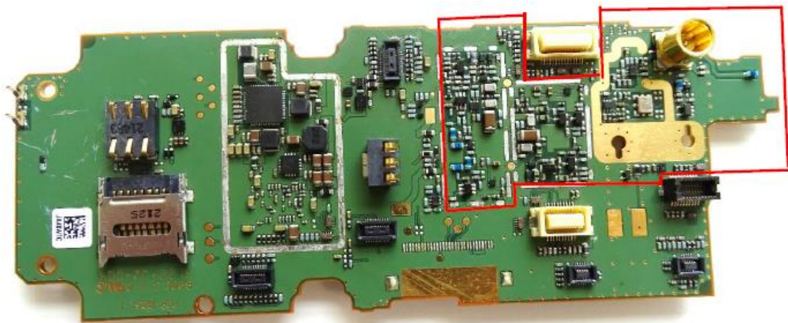
Figure 17 SC2028 MAIN PCB TOP VIEW WITHOUT CANS
