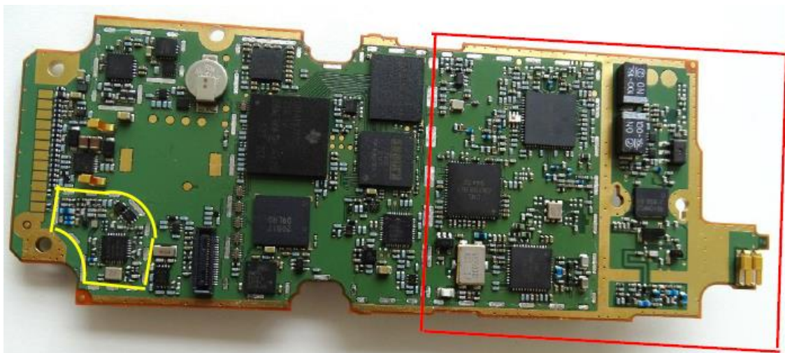
Figure 19 SC2028 MAIN PCB BOTTOM VIEW WITHOUT CANS
