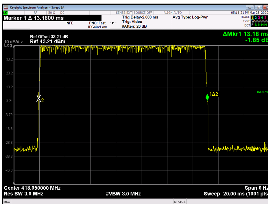
Figure 2 - Burst Length
