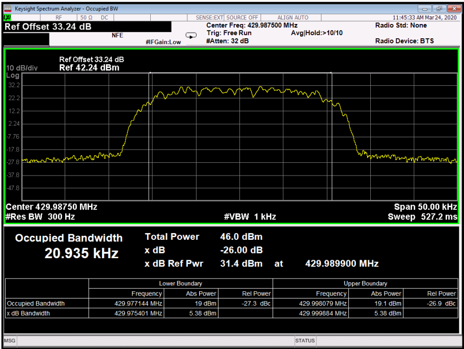
Figure 10 - 429.9875 MHz
