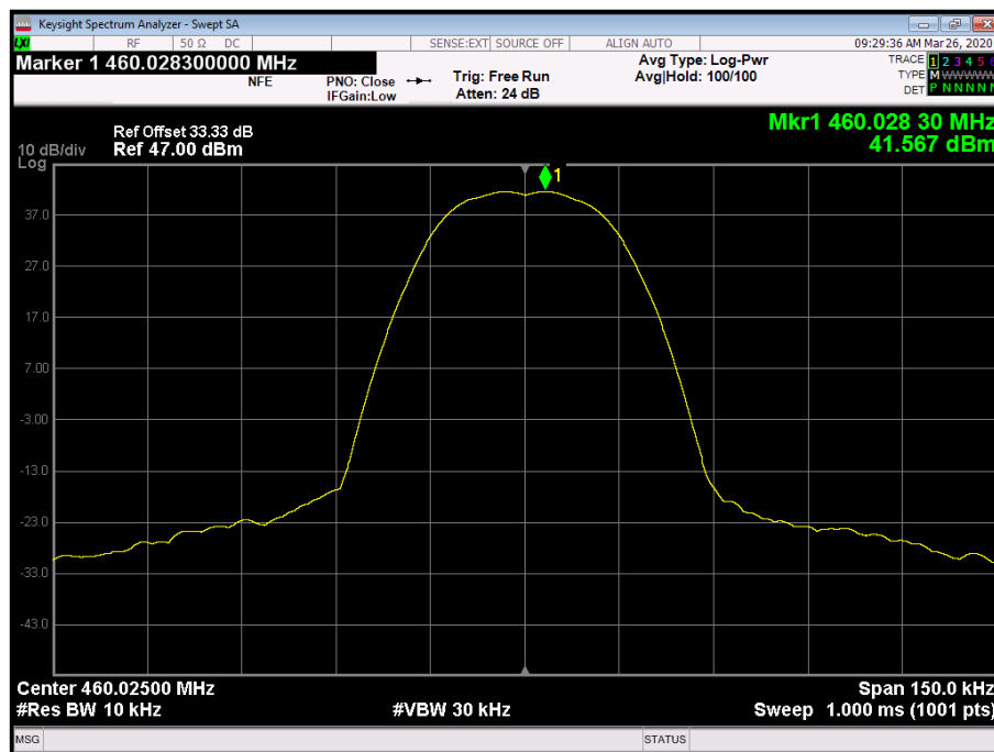
Figure 7 - Frequency Spectrum
