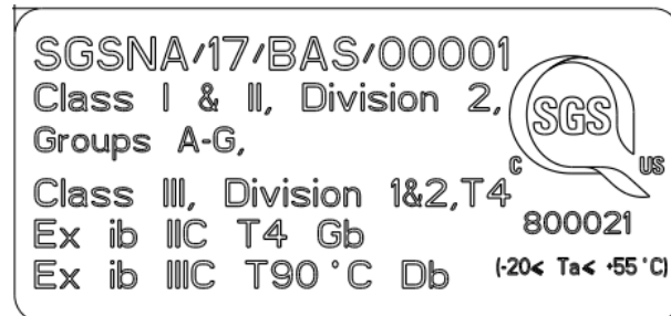
Figure 7. STP8X SGS North America label
