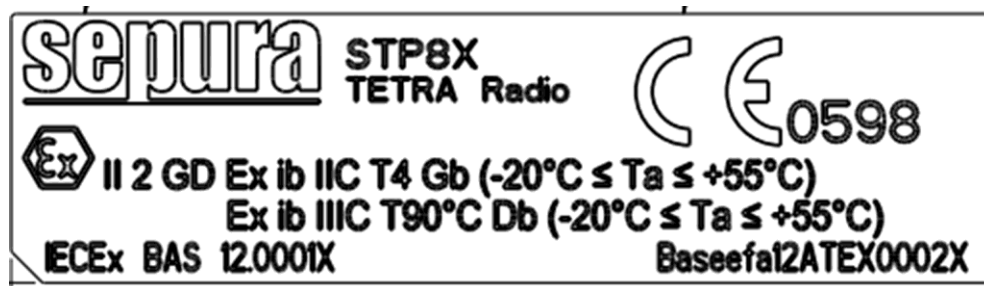
Figure 8. STP8X Lower label
