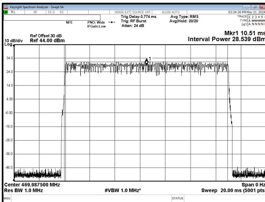
Figure 6 - 469.9875 MHz
