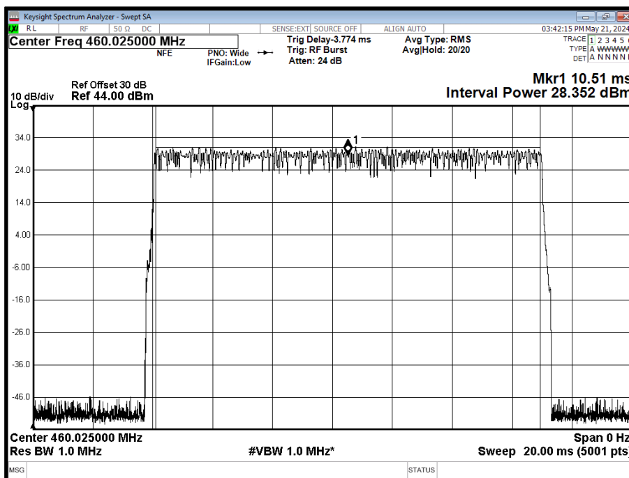
Figure 5 - 460.025 MHz
