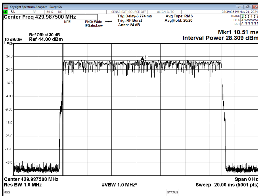
Figure 3 - 429.9875 MHz
