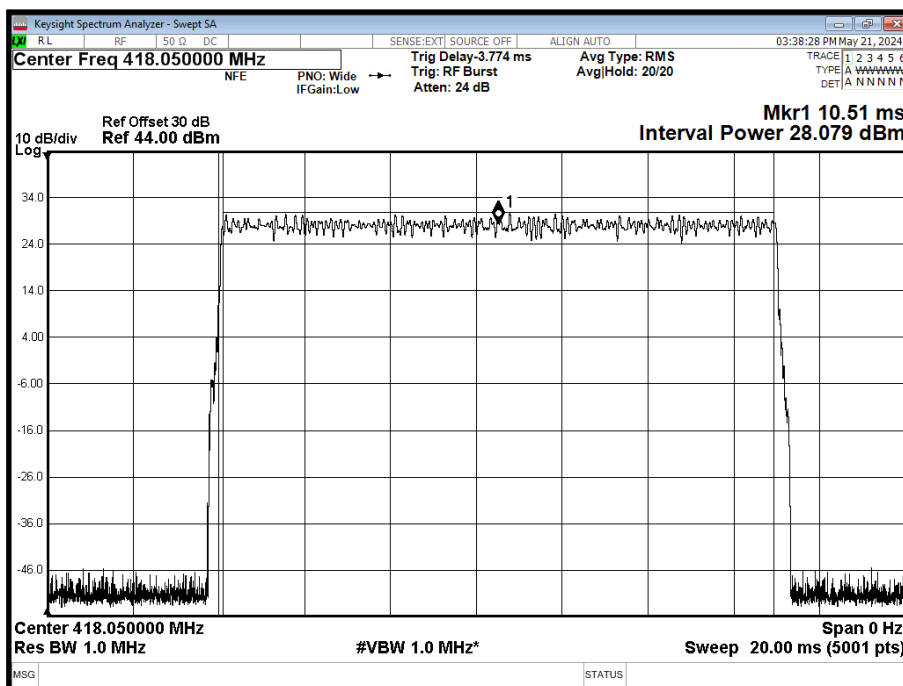
Figure 2 - 418.05 MHz
