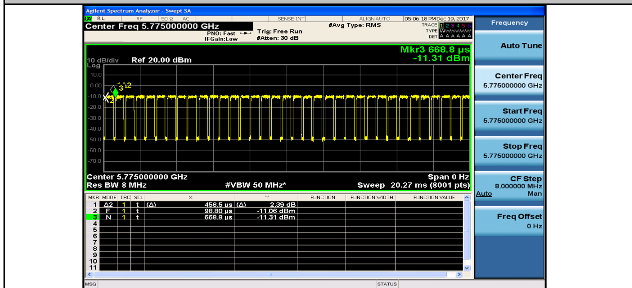
Duty Cycle_11AC80_5775_Ant1
