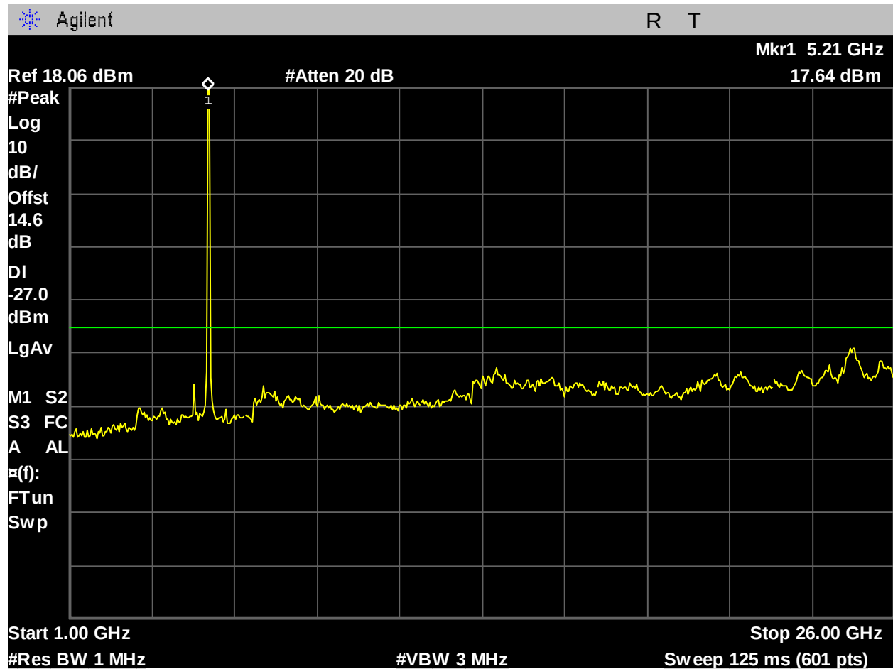
Figure 556: U-NII-1_5230MHz_high_Mid Ch_46_40MHz BW_n-mode_-27dBm_1-26GHz_Port 2.
