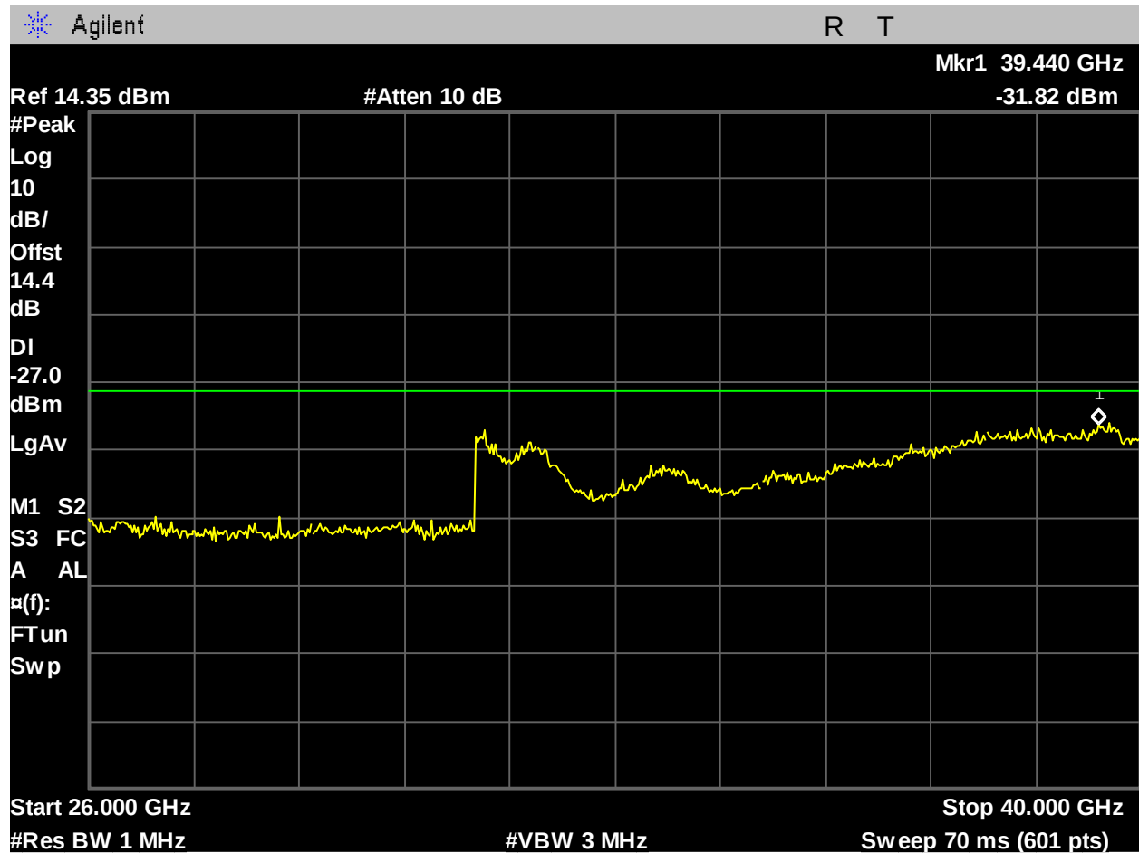
Figure 345: U-NII-3_5745MHz_Low Ch_149_20MHz BW_ax-mode_-27dBm_26-40GHz_Port 1.
