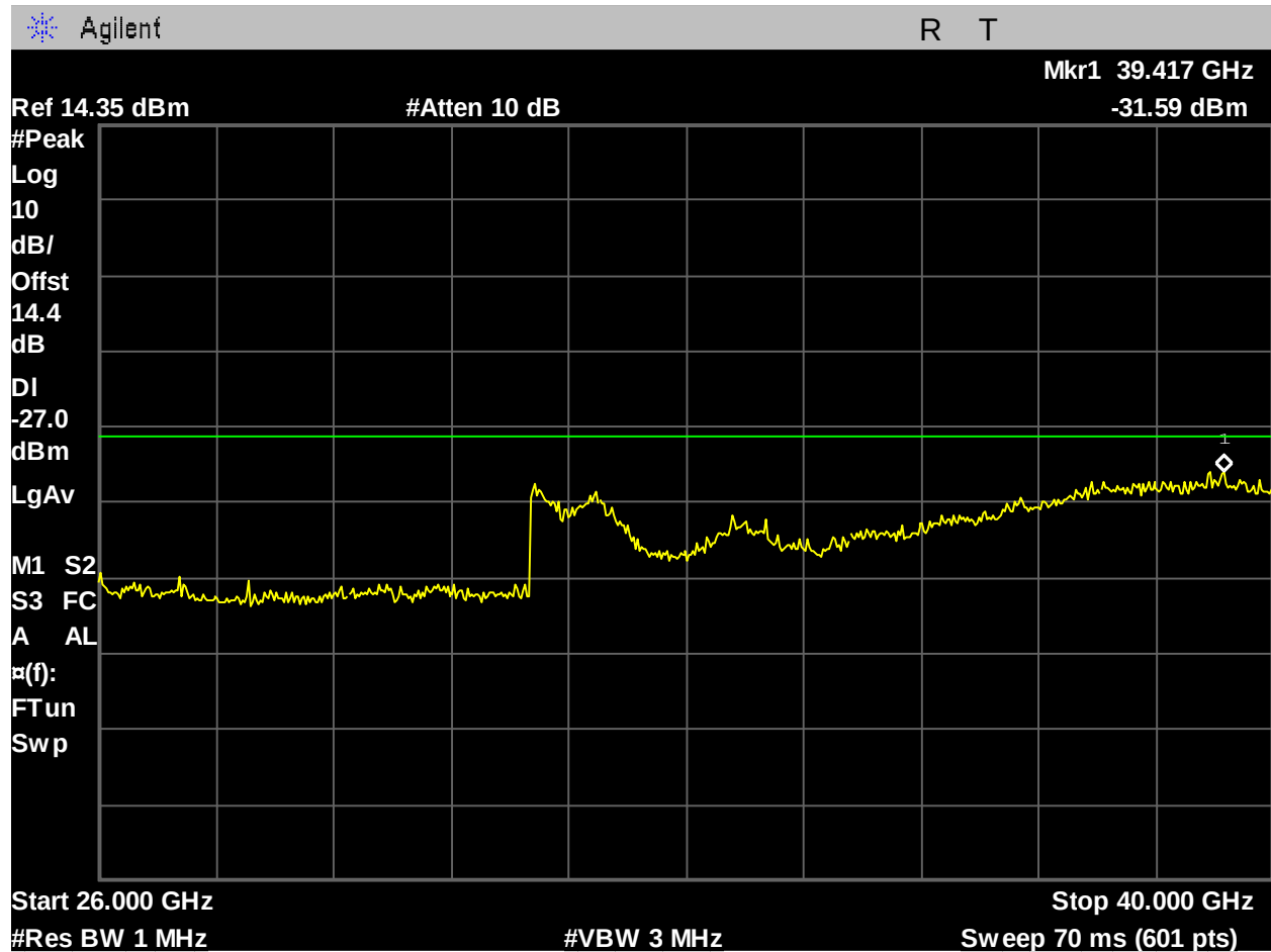
Figure 333: U-NII-3_5745MHz_Low Ch_149_20MHz BW_a-mode_-27dBm_26-40GHz_Port 1.
