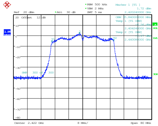
802.11n40_2422MHz_Chain 0 35.840MHz
