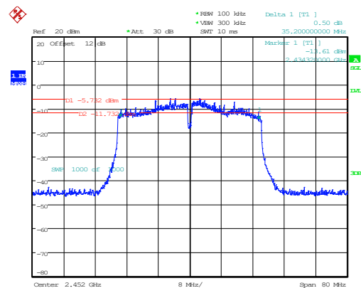
802.11n40_2452MHz_Chain 1 35.200MHz
