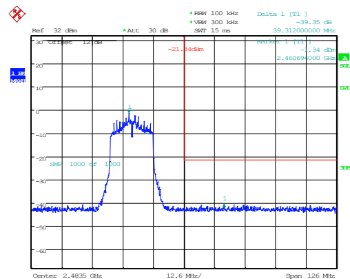
802.11n20_2462MHz_Chain 1 39.35dB
