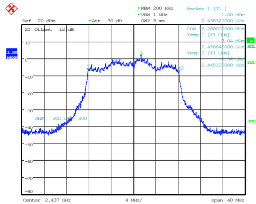
802.11g_2437MHz_Chain 0 16.280MHz
