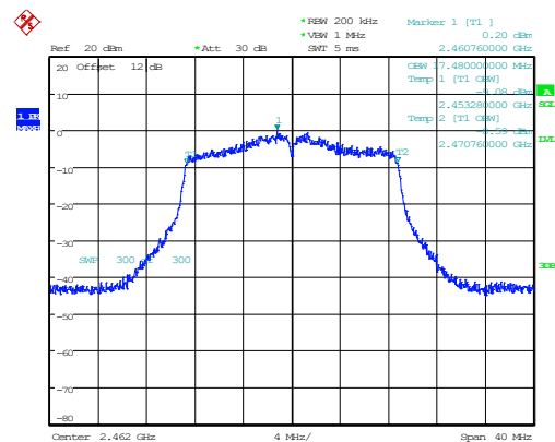
802.11n20_2462MHz_Chain 1 17.480MHz
