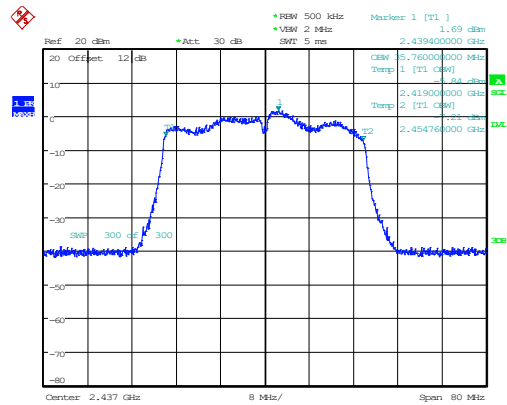
802.11n40_2437MHz_Chain 0 35.760MHz
