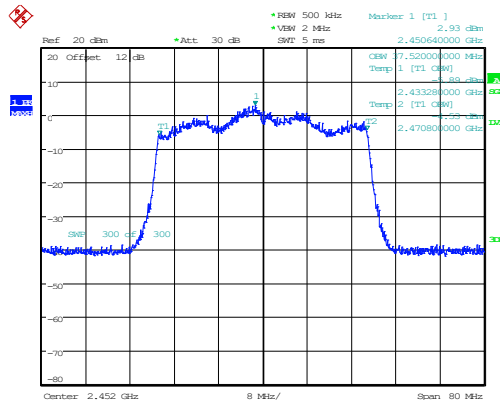
802.11ax40_2452MHz_RU_484/65_Chain 0 37.520MHz
