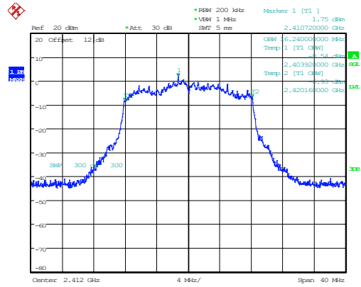
802.11g_2412MHz_Chain 0 16.240MHz
