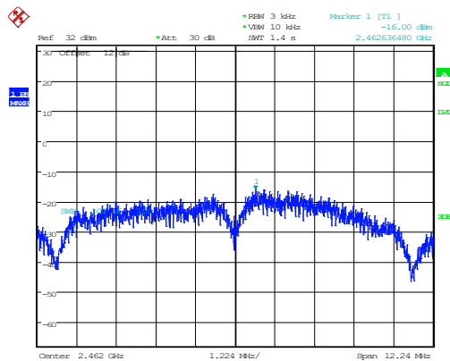
802.11b_2462MHz_Chain 0 -16.00dBm/3kHz
