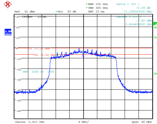
802.11ax20_2412MHz_RU_242/61_Chain 1 15.160MHz
