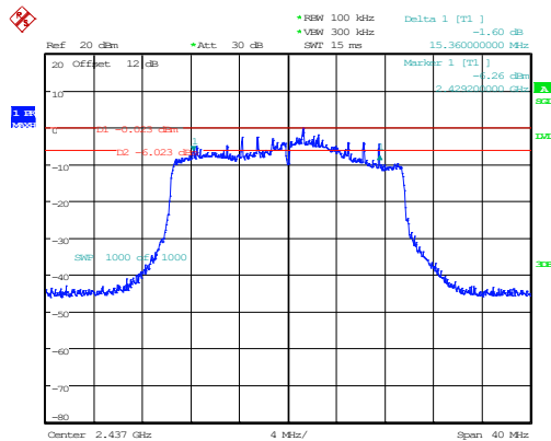
802.11ax20_2437MHz_RU_242/61_Chain 0 15.360MHz
