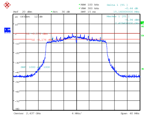
802.11ax20_2437MHz_RU_242/61_Chain 1 15.160MHz
