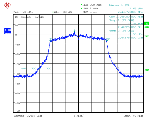
802.11n20_2437MHz_Chain 1 17.480MHz
