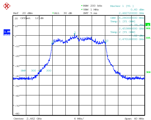
802.11g_2462MHz_Chain 0 16.280MHz
