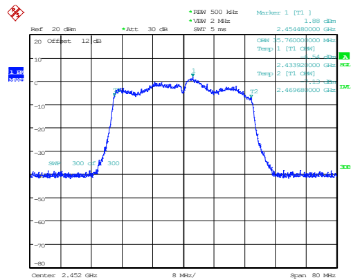
802.11n40_2452MHz_Chain 0 35.760MHz
