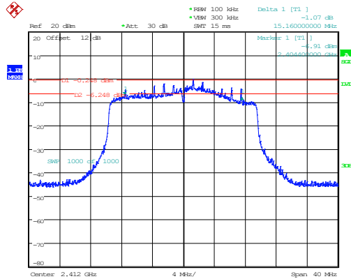
802.11ax20_2412MHz_RU_242/61_Chain 0 15.160MHz
