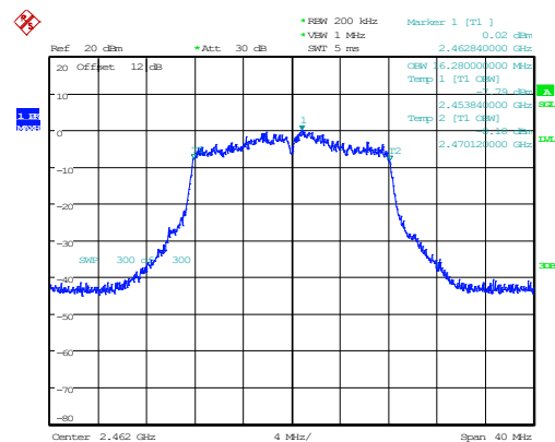
802.11g_2462MHz_Chain 1 16.280MHz
