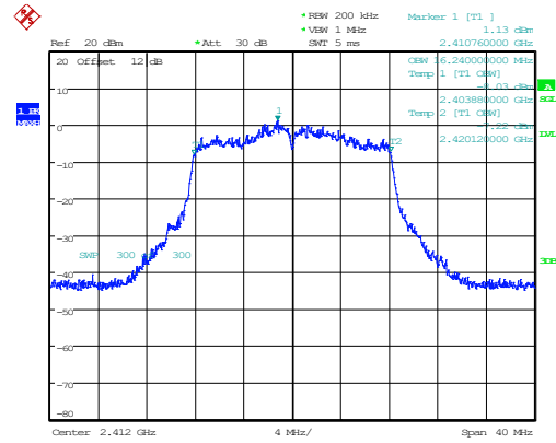
802.11g_2412MHz_Chain 1 16.240MHz
