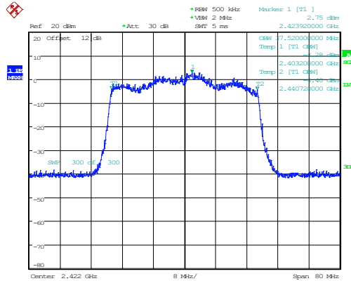
802.11ax40_2422MHz_RU_484/65_Chain 0 37.520MHz
