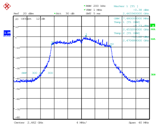
802.11n20_2462MHz_Chain 0 17.480MHz
