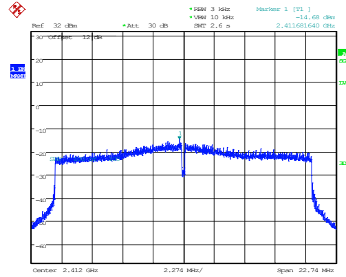
802.11ax20_2412MHz_RU_242/61_Chain 1 -14.68dBm/3kHz
