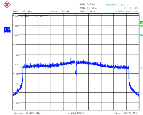
802.11ax20_2462MHz_RU_242/61_Chain 1 -16.02dBm/3kHz
