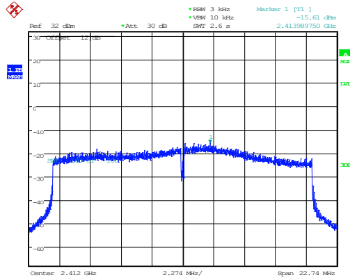
802.11ax20_2412MHz_RU_242/61_Chain 0 -15.61dBm/3kHz
