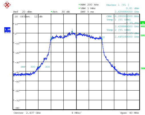
802.11g_2437MHz_Chain 1 16.280MHz
