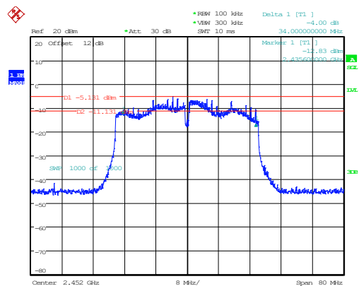
802.11n40_2452MHz_Chain 0 34MHz
