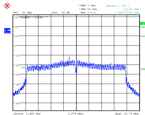
802.11n20_2462MHz_Chain 1 -13.91dBm/3kHz
