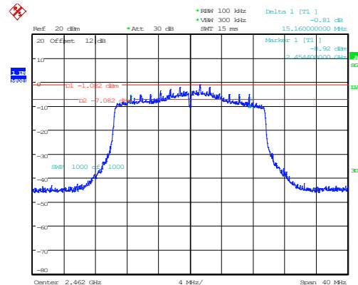
802.11ax20_2462MHz_RU_242/61_Chain 1 15.160MHz
