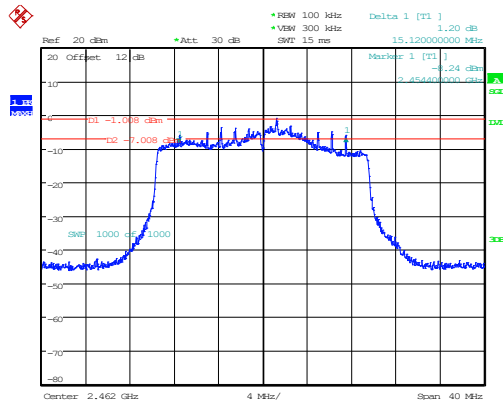
802.11ax20_2462MHz_RU_242/61_Chain 0 15.120MHz
