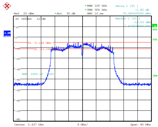
802.11n40_2437MHz_Chain 0 35.280MHz
