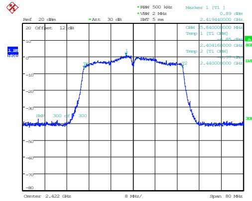
802.11n40_2422MHz_Chain 1 35.840MHz
