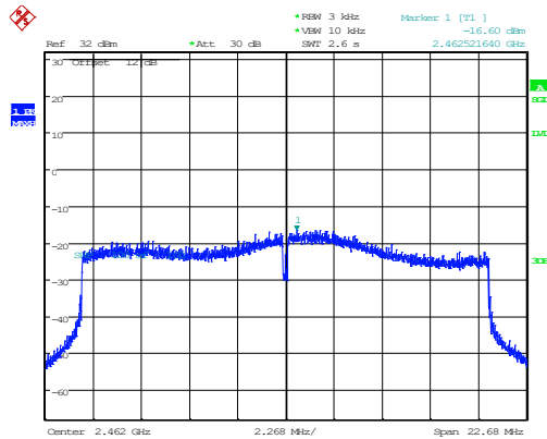
802.11ax20_2462MHz_RU_242/61_Chain 0 -16.60dBm/3kHz
