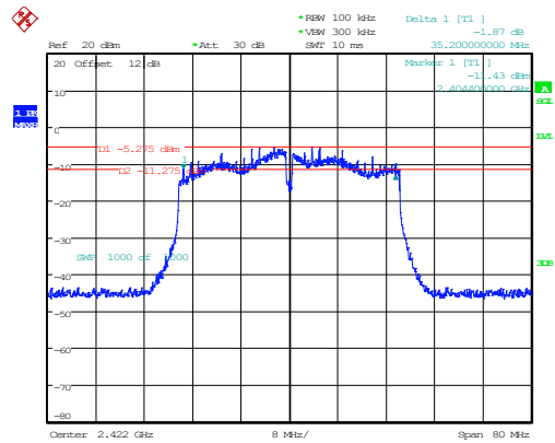
802.11n40_2422MHz_Chain 0 35.200MHz
