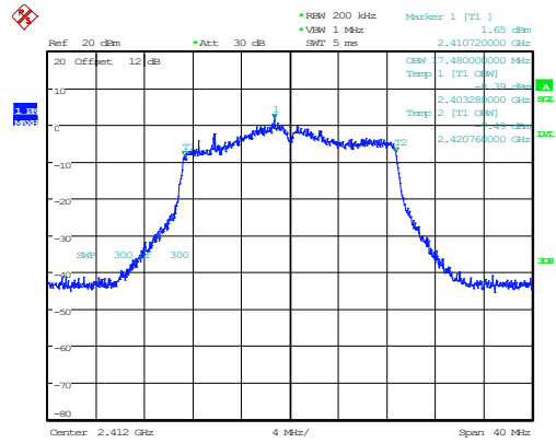
802.11n20_2412MHz_Chain 0 17.480MHz
