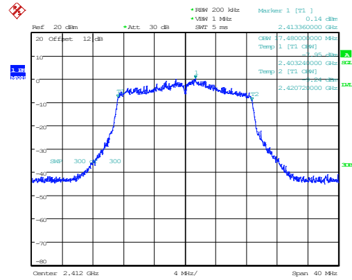
802.11n20_2412MHz_Chain 1 17.480MHz
