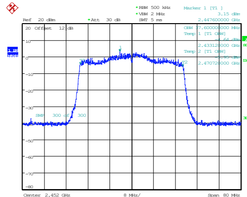
802.11ax40_2452MHz_RU_484/65_Chain 1 37.600MHz
