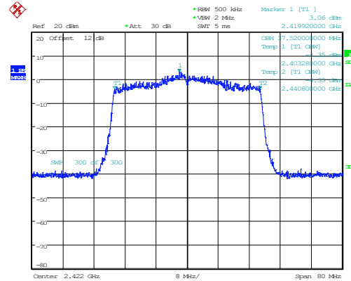
802.11ax40_2422MHz_RU_484/65_Chain 1 37.520MHz
