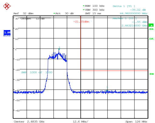
802.11n20_2462MHz_Chain 0 39.02dB
