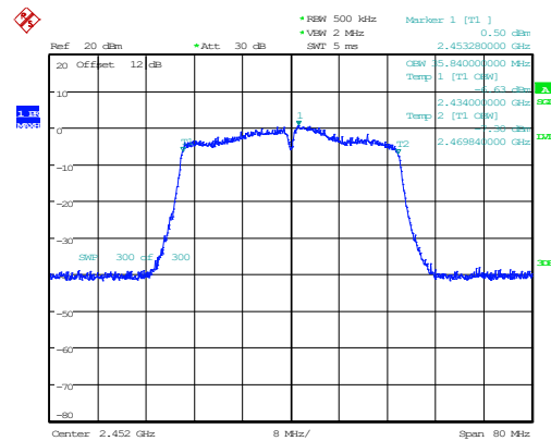
802.11n40_2452MHz_Chain 1 35.840MHz
