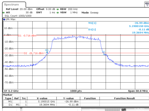
802.11a_5200MHz_Chain 0 19.369MHz
