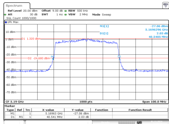
802.11ax40_5190MHz_RU_484/65_Chain 1 40.541MHz
