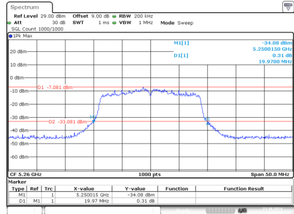
802.11n20_5260MHz_Chain 1 19.970MHz
