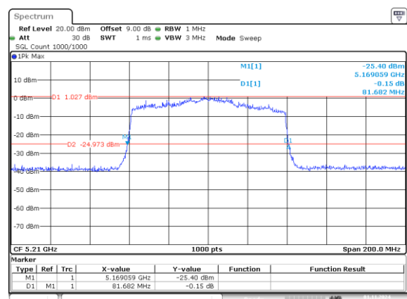
802.11ax80_5210MHz_RU_996/67_Chain 1 81.682MHz
