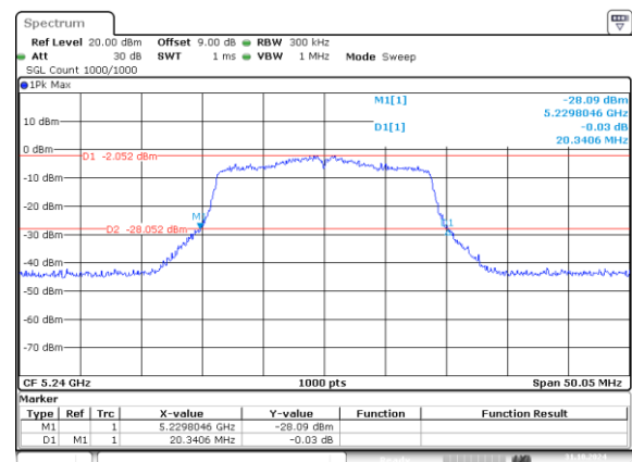
802.11n20_5240MHz_Chain 1 20.341MHz
