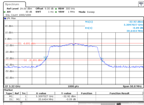
802.11n20_5320MHz_Chain 1 20.645MHz
