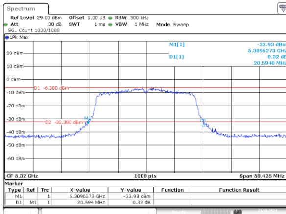
802.11n20_5320MHz_Chain 0 20.594MHz
