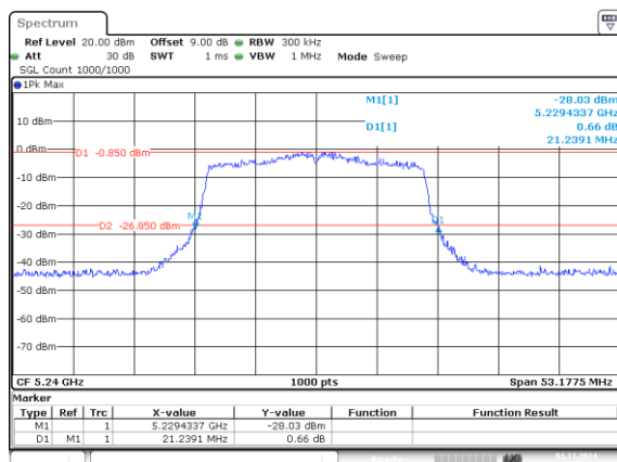
802.11ax20_5240MHz_RU_242/61_Chain 0 21.239MHz
