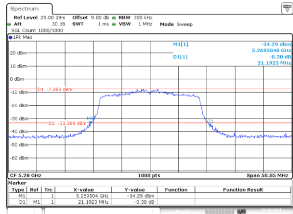
802.11n20_5280MHz_Chain 1 21.192MHz
