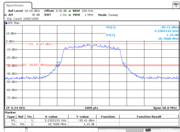
802.11a_5240MHz_Chain 1 18.769MHz
