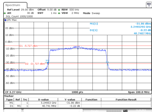
802.11ax40_5270MHz_RU_484/65_Chain 1 40.741MHz
