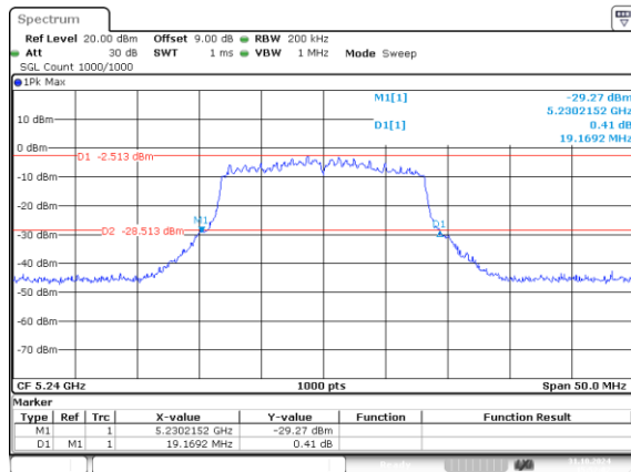
802.11a_5240MHz_Chain 0 19.169MHz
