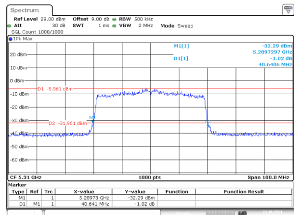
802.11ax40_5310MHz_RU_484/65_Chain 1 40.641MHz
