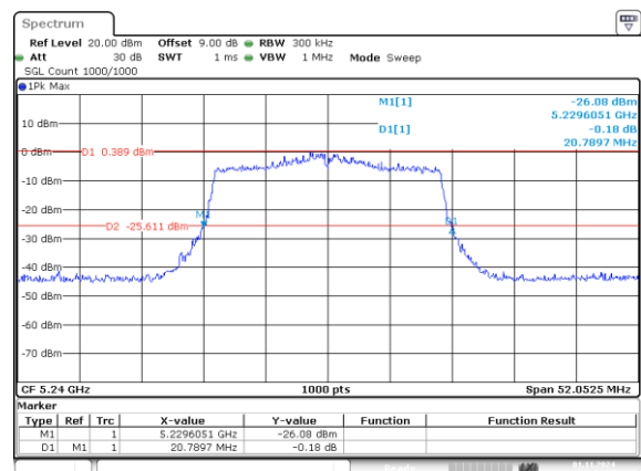
802.11ax20_5240MHz_RU_242/61_Chain 1 20.790MHz
