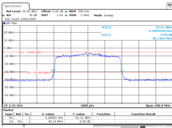
802.11ax40_5310MHz_RU_484/65_Chain 0 40.140MHz
