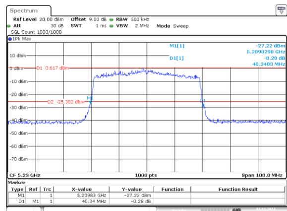
802.11ax40_5230MHz_RU_484/65_Chain 1 40.340MHz
