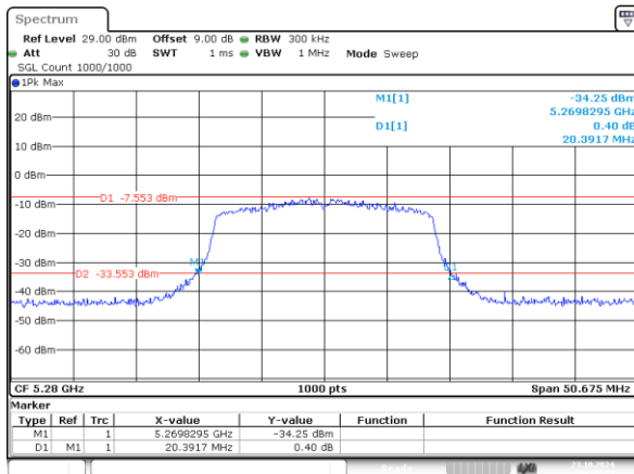
802.11n20_5280MHz_Chain 0 20.392MHz
