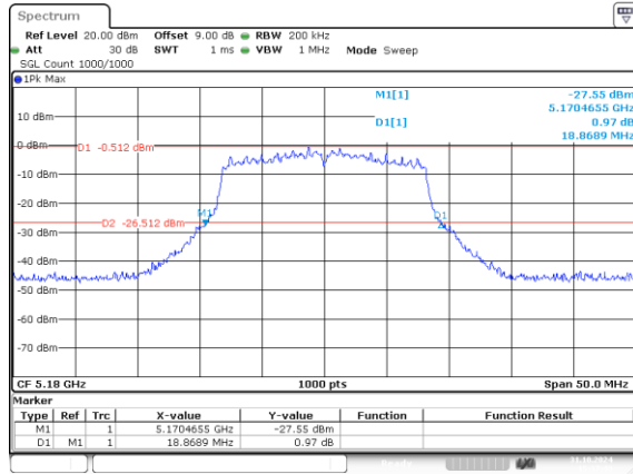
802.11a_5180MHz_Chain 0 18.869MHz
