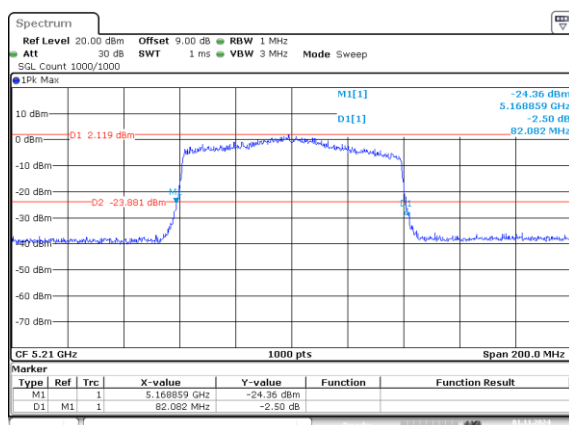
802.11ax80_5210MHz_RU_996/67_Chain 0 82.082MHz
