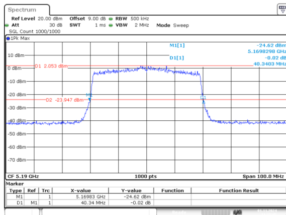
802.11ax40_5190MHz_RU_484/65_Chain 0 40.340MHz
