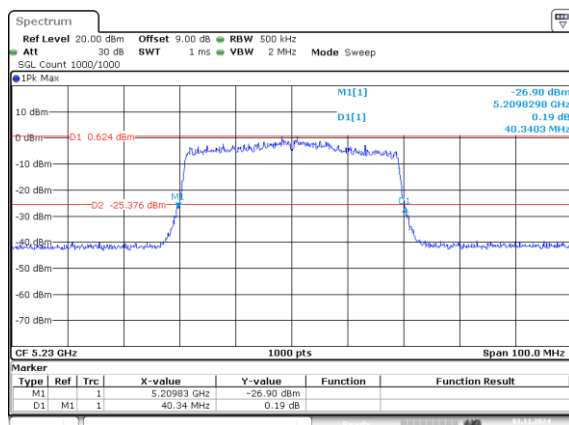
802.11ax40_5230MHz_RU_484/65_Chain 0 40.340MHz
