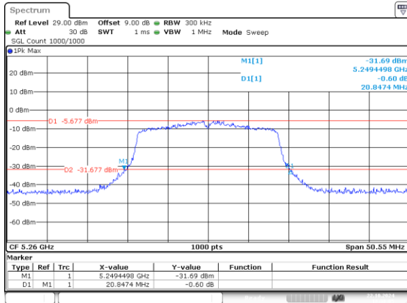
802.11n20_5260MHz_Chain 0 20.847MHz
