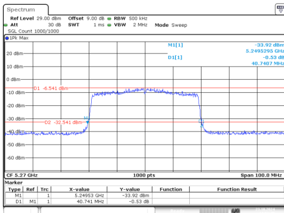
802.11ax40_5270MHz_RU_484/65_Chain 0 40.741MHz
