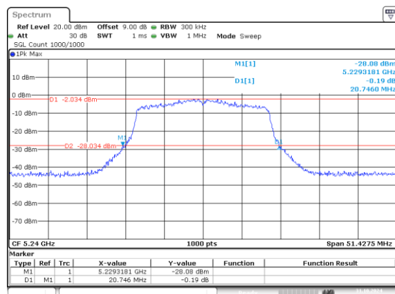
802.11n20_5240MHz_Chain 0 20.746MHz
