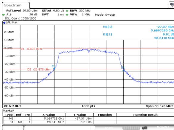
802.11n20_5700MHz_Chain 0 20.341MHz
