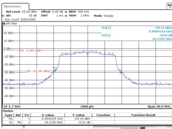
802.11a_5700MHz_Chain 0 19.219MHz
