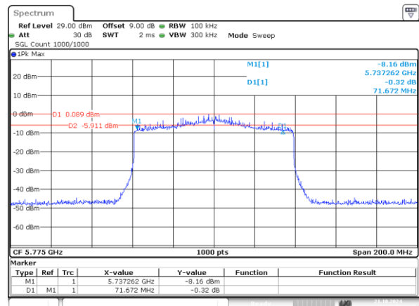
802.11ax80_5775MHz_RU_996/67_Chain 1 71.672MHz
