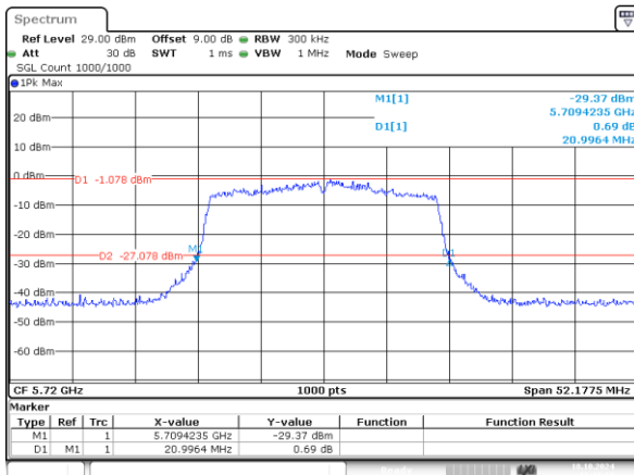
802.11ax20_5720MHz_RU_242/61_Chain 0 20.996MHz
