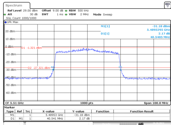
802.11ax40_5510MHz_RU_484/65_Chain 1 40.541MHz
