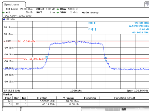
802.11n40_5550MHz_Chain 0 40.140MHz
