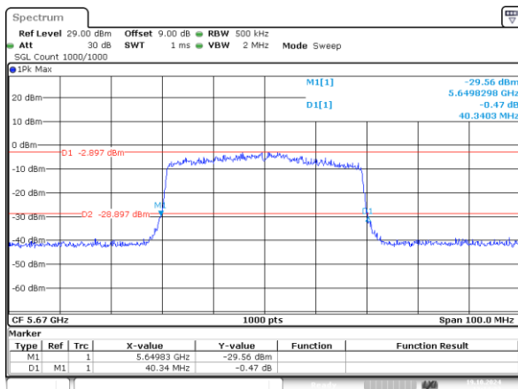
802.11ax40_5670MHz_RU_484/65_Chain 0 40.340MHz
