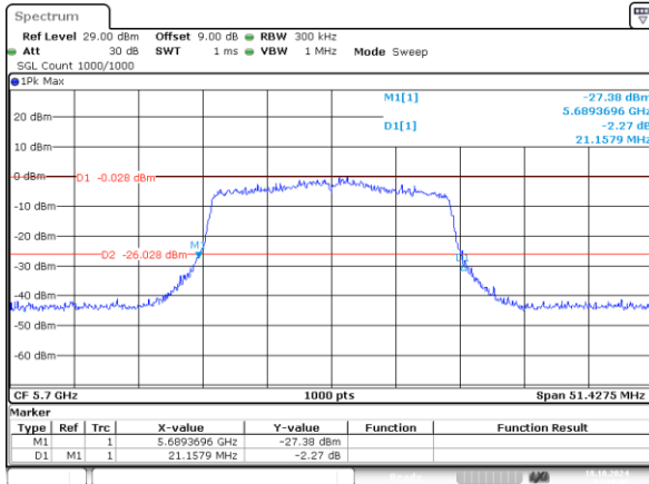
802.11ax20_5700MHz_RU_242/61_Chain 0 21.158MHz
