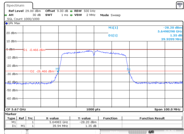
802.11n40_5670MHz_Chain 1 39.940MHz
