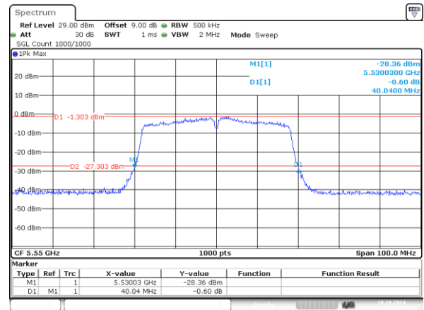
802.11n40_5550MHz_Chain 1 40.040MHz
