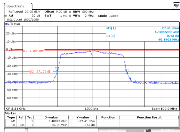
802.11n40_5510MHz_Chain 1 40.140MHz
