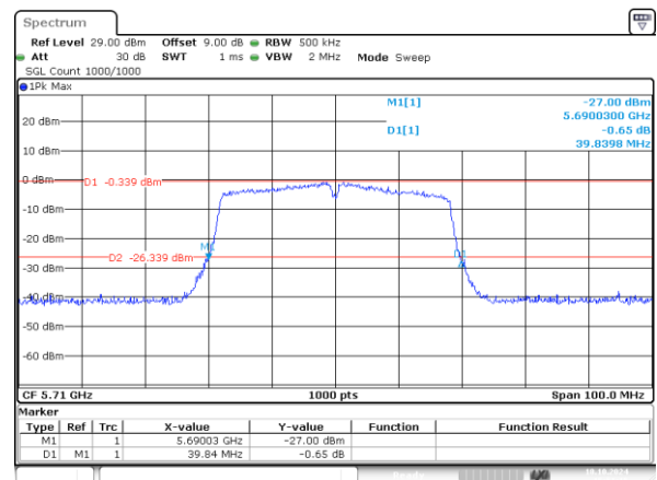
802.11n40_5710MHz_Chain 1 39.840MHz
