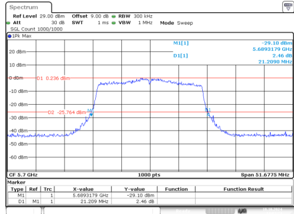
802.11ax20_5700MHz_RU_242/61_Chain 1 21.209MHz
