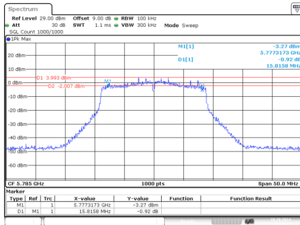
802.11n20_5785MHz_Chain 0 15.816MHz
