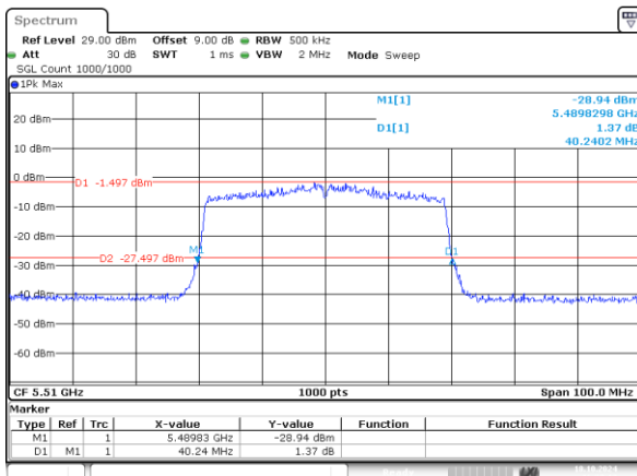
802.11ax40_5510MHz_RU_484/65_Chain 0 40.240MHz
