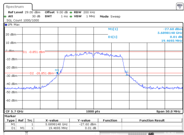
802.11a_5700MHz_Chain 1 19.469MHz
