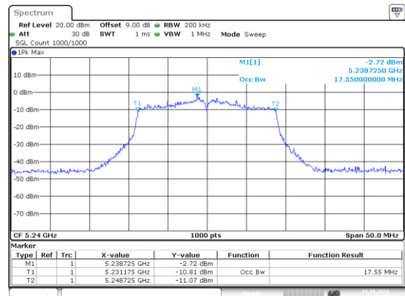
802.11n20_5240MHz_Chain 1 17.550MHz
