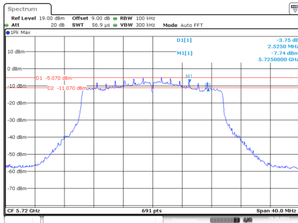
802.11ax20_5720MHz_RU_242/61_Chain 0 2.525MHz
