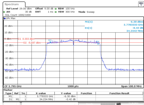
802.11ax40_5795MHz_RU_484/65_Chain 1 34.234MHz
