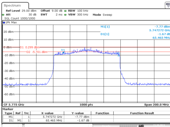
802.11ax80_5775MHz_RU_996/67_Chain 0 65.465MHz
