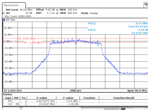
802.11n20_5825MHz_Chain 0 15.215MHz
