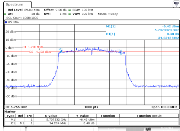
802.11ax40_5755MHz_RU_484/65_Chain 1 34.234MHz
