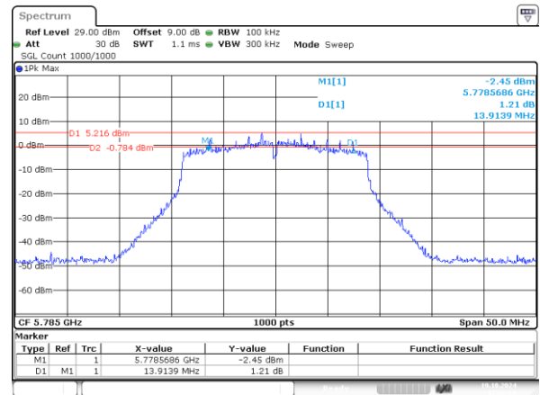
802.11n20_5785MHz_Chain 1 13.914MHz
