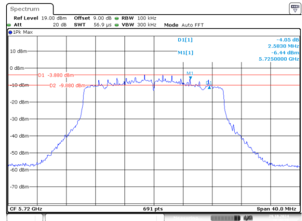
802.11ax20_5720MHz_RU_242/61_Chain 1 2.583MHz
