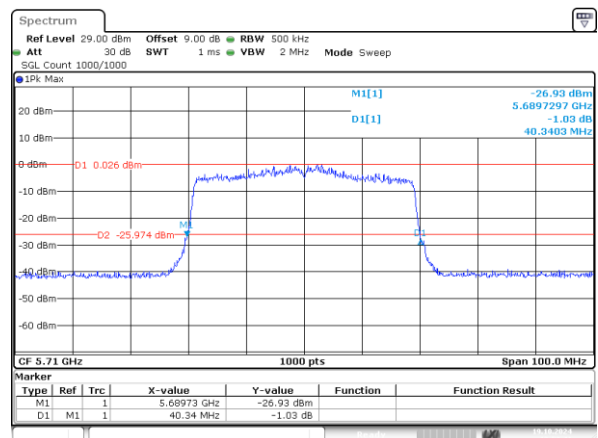
802.11ax40_5710MHz_RU_484/65_Chain 1 40.340MHz
