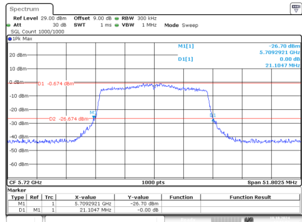
802.11ax20_5720MHz_RU_242/61_Chain 1 21.105MHz
