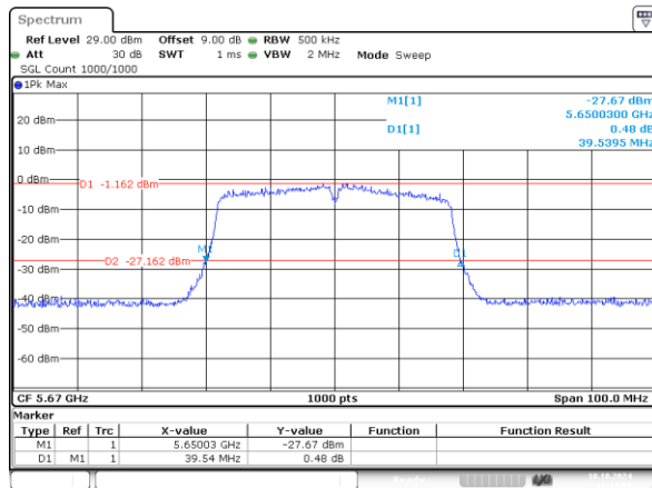
802.11n40_5670MHz_Chain 0 39.540MHz
