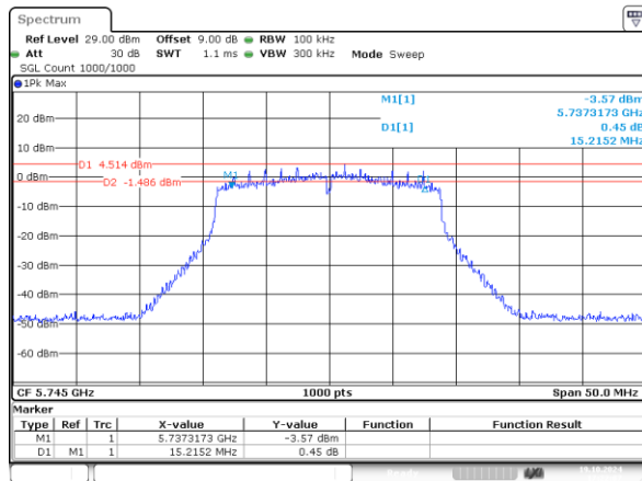
802.11n20_5745MHz_Chain 0 15.215MHz
