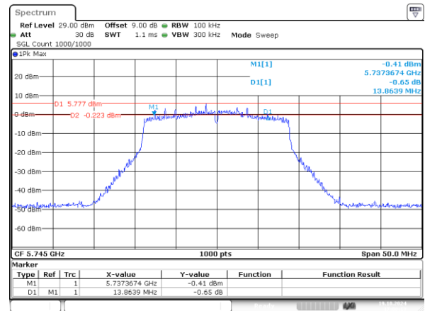
802.11n20_5745MHz_Chain 1 13.864MHz
