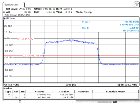
802.11ax40_5670MHz_RU_484/65_Chain 1 40.841MHz
