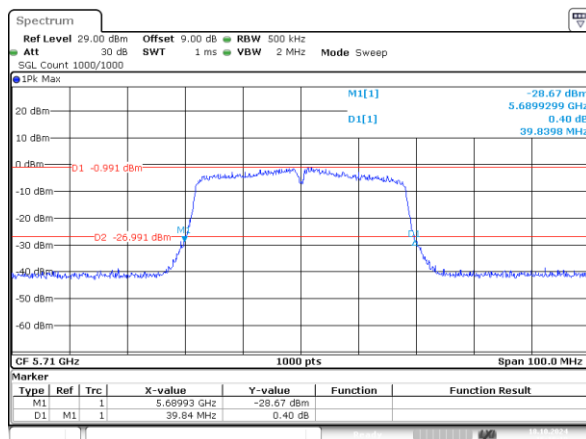
802.11n40_5710MHz_Chain 0 39.840MHz
