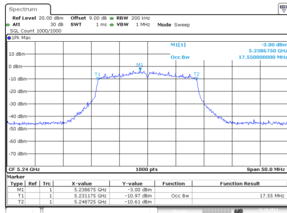
802.11n20_5240MHz_Chain 0 17.550MHz
