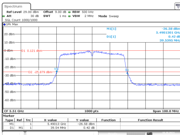
802.11n40_5510MHz_Chain 0 39.540MHz
