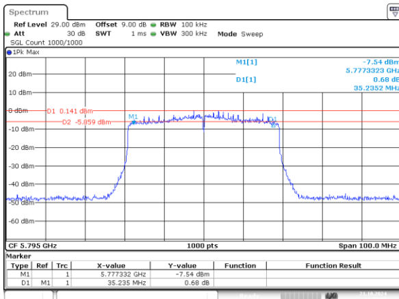
802.11ax40_5795MHz_RU_484/65_Chain 0 35.235MHz
