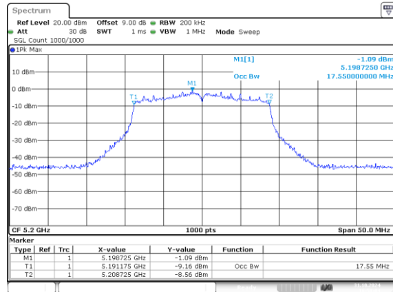
802.11n20_5200MHz_Chain 0 17.550MHz
