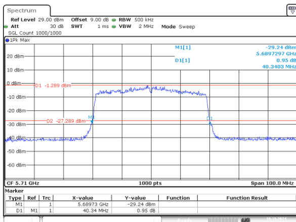
802.11ax40_5710MHz_RU_484/65_Chain 0 40.340MHz
