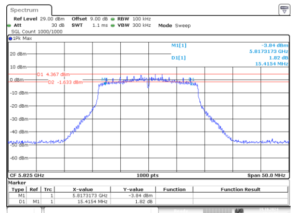
802.11n20_5825MHz_Chain 1 15.415MHz
