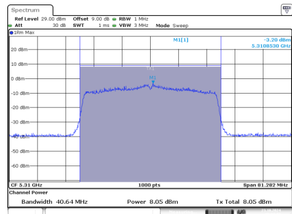
802.11ax40_5310MHz_RU_484/65_Chain 1
