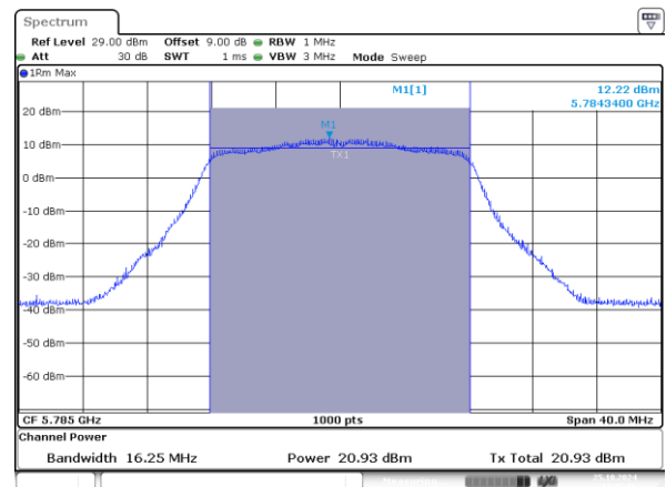
802.11a_5785MHz_Chain 1
