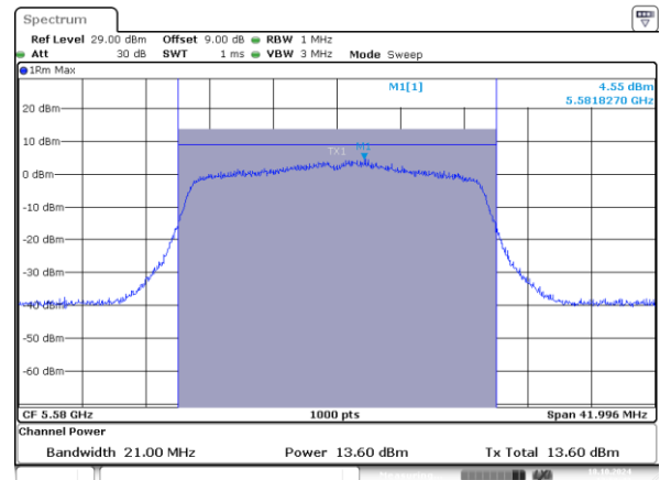
802.11ax20_5580MHz_RU_242/61_Chain 1
