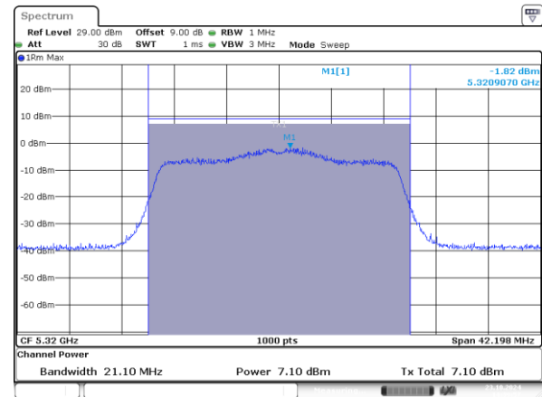
802.11ax20_5320MHz_RU_242/61_Chain 1
