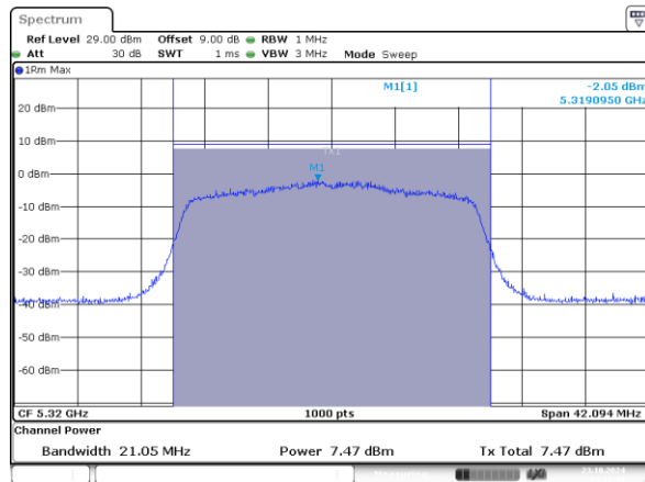
802.11ax20_5320MHz_RU_242/61_Chain 0
