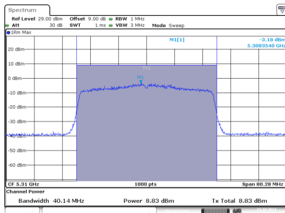
802.11ax40_5310MHz_RU_484/65_Chain 0
