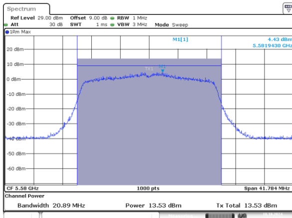
802.11ax20_5580MHz_RU_242/61_Chain 0
