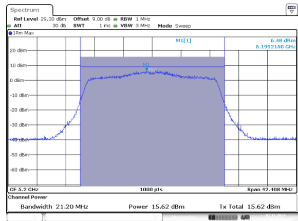
802.11ax20_5200MHz_RU_242/61_Chain 1
