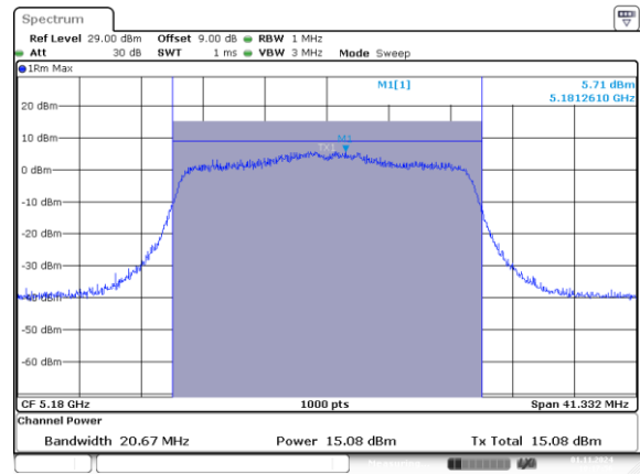
802.11ax20_5180MHz_RU_242/61_Chain 1
