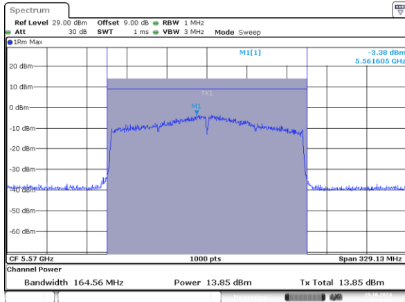
802.11ax160_5570MHz_RU_2*996_Chain 0
