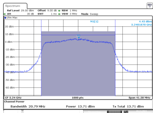
802.11ax20_5240MHz_RU_242/61_Chain 1
