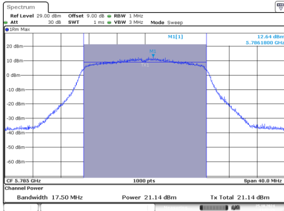
802.11n20_5785MHz_Chain 0
