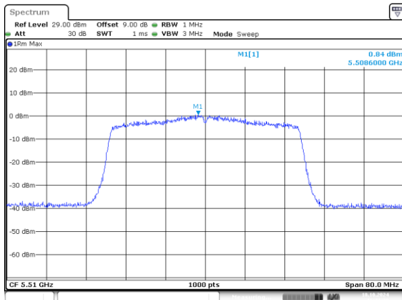
802.11ax40_5510MHz_RU_484/65_Chain 0
