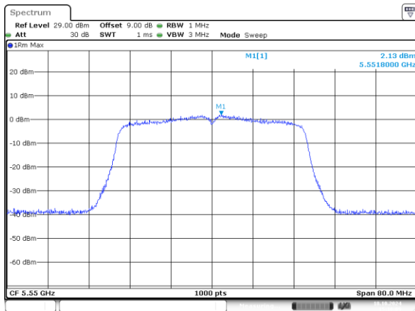
802.11n40_5550MHz_Chain 0
