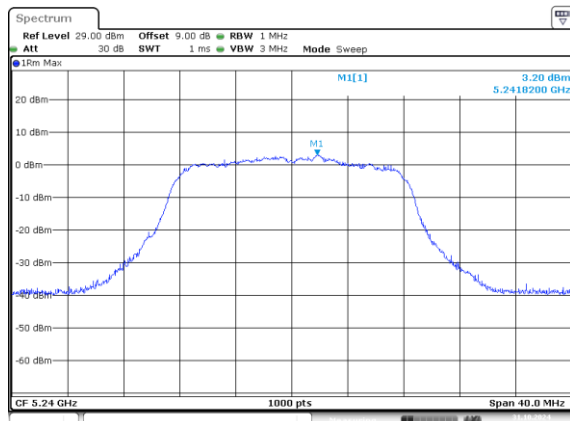
802.11a_5240MHz_Chain 0
