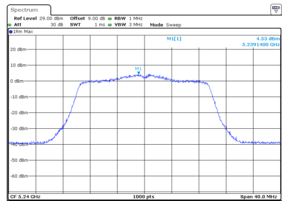
802.11ax20_5240MHz_RU_242/61_Chain 1
