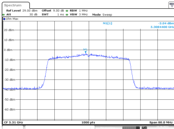
802.11ax40_5310MHz_RU_484/65_Chain 0
