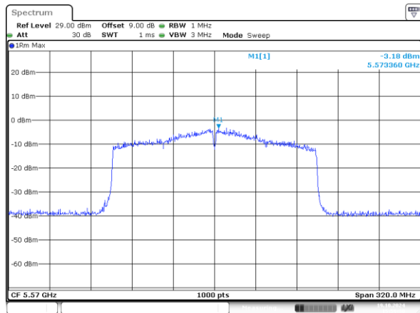
802.11ax160_5570MHz_RU_2*996_Chain 0
