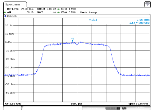
802.11n40_5550MHz_Chain 1
