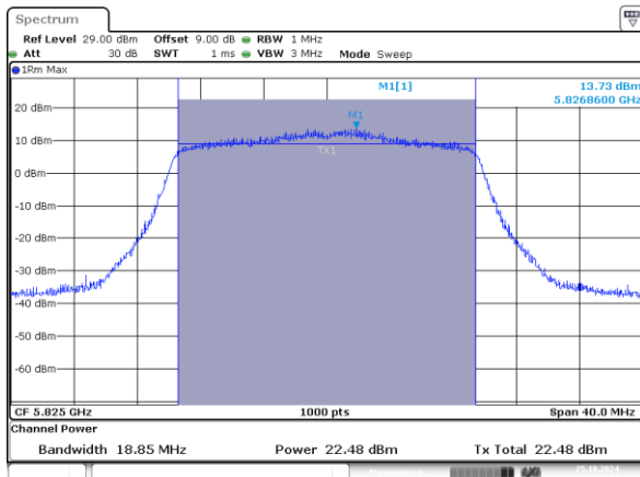
802.11ax20_5825MHz_RU_242/61_Chain 0
