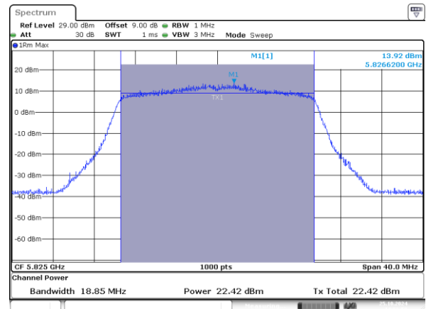
802.11ax20_5825MHz_RU_242/61_Chain 1
