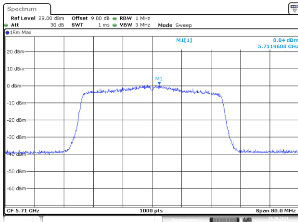
802.11ax40_5710MHz_RU_484/65_Chain 0
