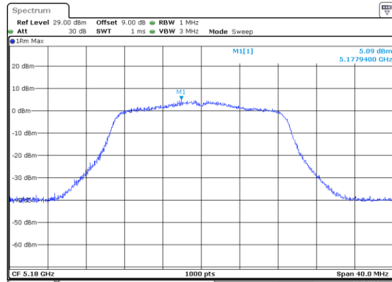
802.11n20_5180MHz_Chain 0
