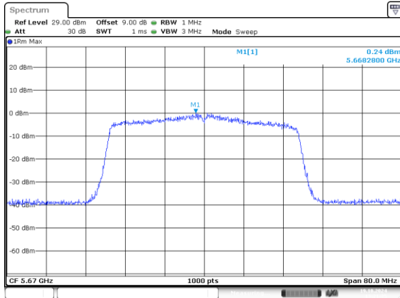
802.11ax40_5670MHz_RU_484/65_Chain 0
