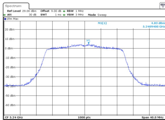
802.11ax20_5240MHz_RU_242/61_Chain 0
