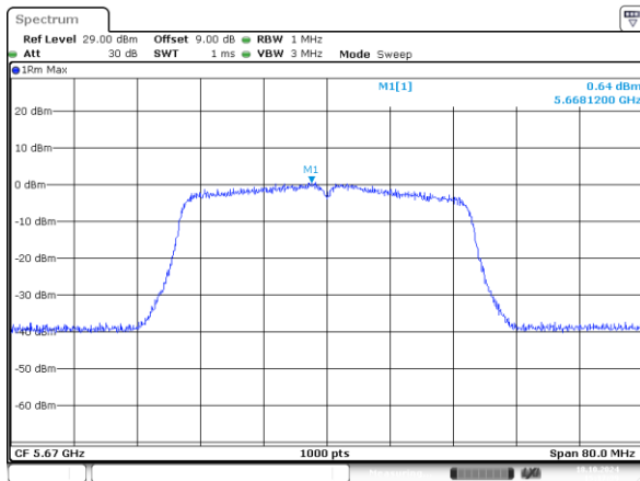
802.11n40_5670MHz_Chain 0
