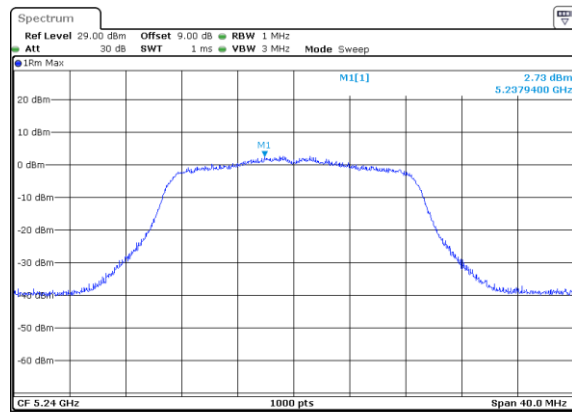
802.11n20_5240MHz_Chain 0
