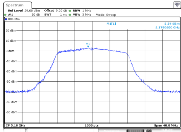
802.11a_5180MHz_Chain 1
