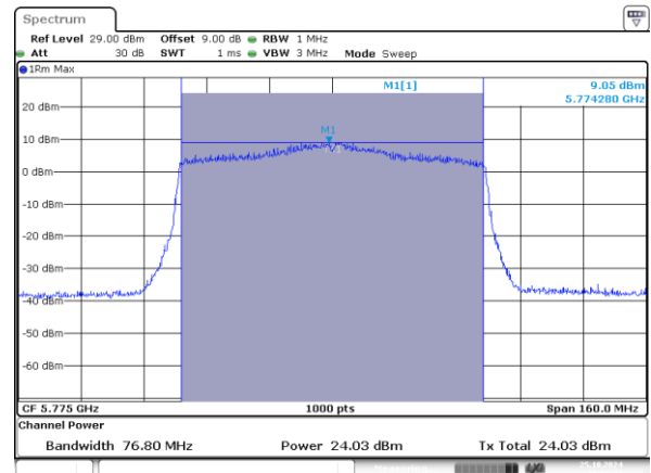
802.11ax80_5775MHz_RU_996/67_Chain 1
