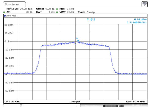
802.11ax40_5510MHz_RU_484/65_Chain 1
