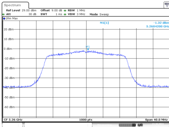
802.11ax20_5260MHz_RU_242/61_Chain 0
