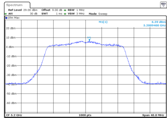
802.11ax20_5200MHz_RU_242/61_Chain 1
