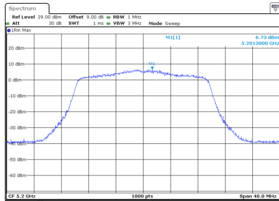
802.11ax20_5200MHz_RU_242/61_Chain 0
