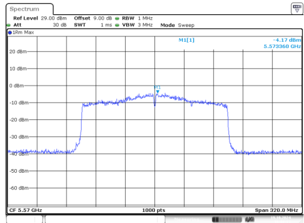
802.11ax160_5570MHz_RU_2*996_Chain 1
