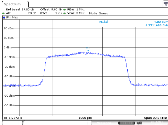
802.11ax40_5270MHz_RU_484/65_Chain 0
