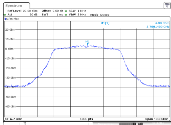
802.11a_5700MHz_Chain 1
