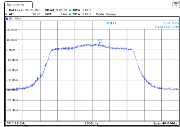
802.11ax20_5180MHz_RU_242/61_Chain 1
