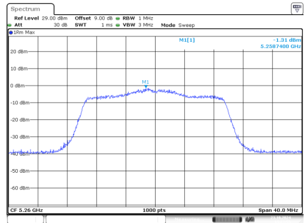
802.11ax20_5260MHz_RU_242/61_Chain 1
