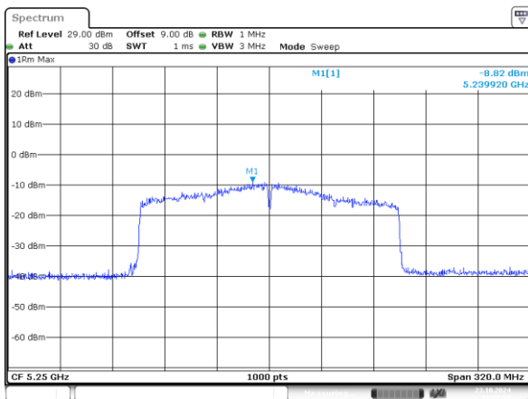
802.11ax160_5250MHz_RU_2*996_Chain 0
