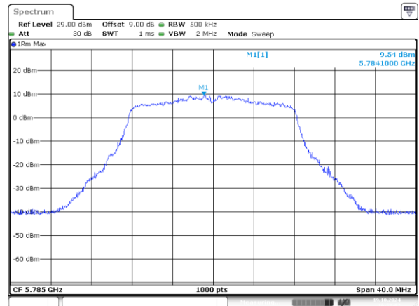
802.11a_5785MHz_Chain 1
