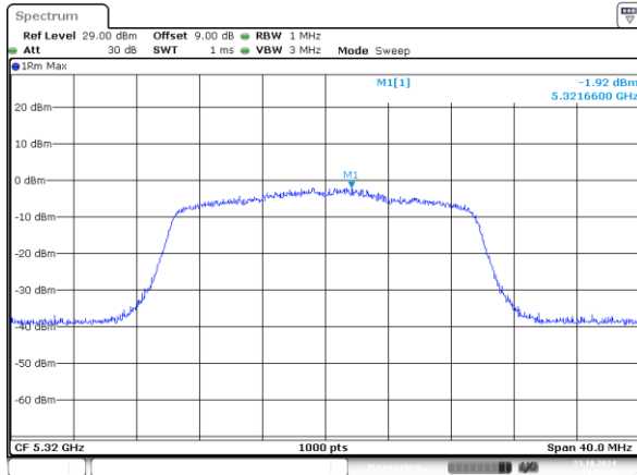
802.11ax20_5320MHz_RU_242/61_Chain 0
