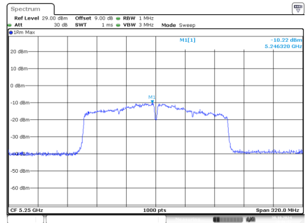
802.11ac160_5250MHz_Chain 1
