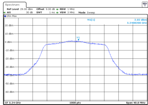
802.11n20_5240MHz_Chain 1
