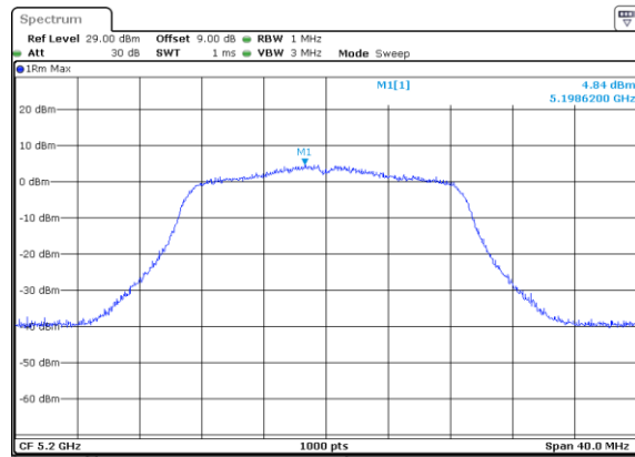
802.11n20_5200MHz_Chain 0
