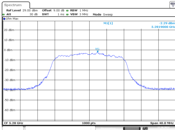
802.11a_5280MHz_Chain 0
