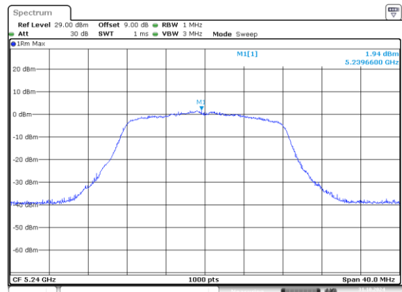
802.11a_5240MHz_Chain 1
