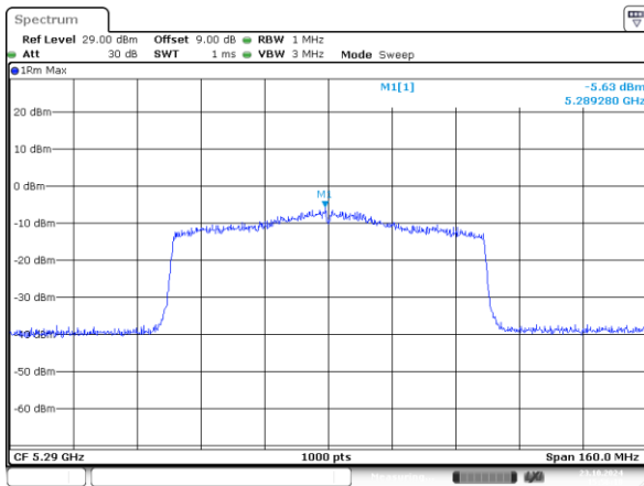
802.11ax80_5290MHz_RU_996/67_Chain 0
