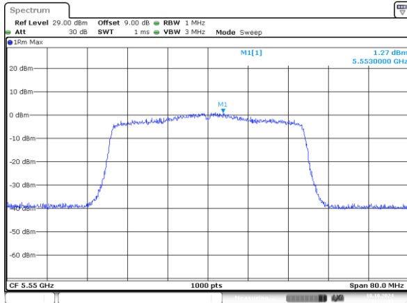
802.11ax40_5550MHz_RU_484/65_Chain 0
