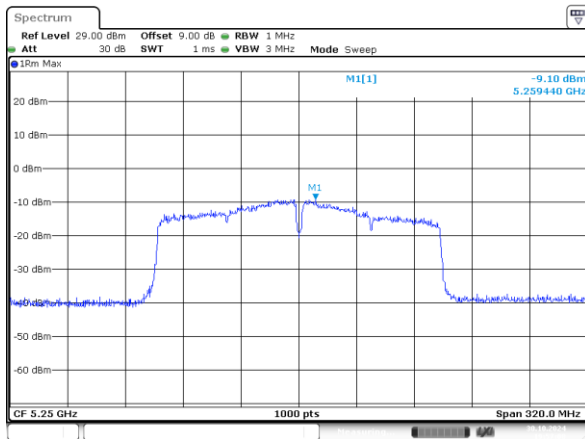
802.11ac160_5250MHz_Chain 0
