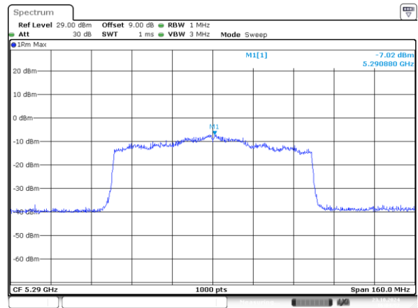
802.11ax80_5290MHz_RU_996/67_Chain 1
