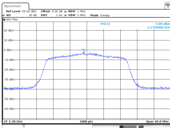
802.11ax20_5280MHz_RU_242/61_Chain 0
