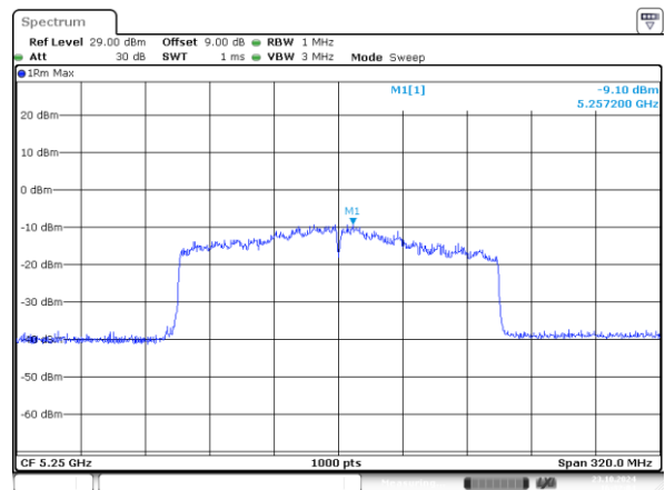
802.11ax160_5250MHz_RU_2*996_Chain 1
