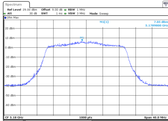
802.11ax20_5180MHz_RU_242/61_Chain 0
