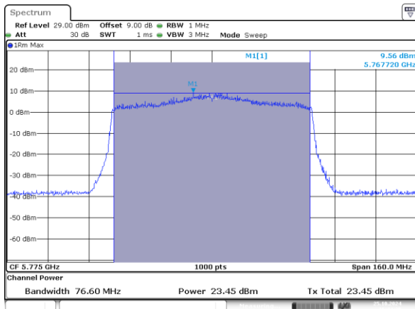
802.11ax80_5775MHz_RU_996/67_Chain 0
