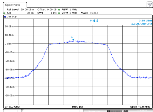
802.11a_5200MHz_Chain 1
