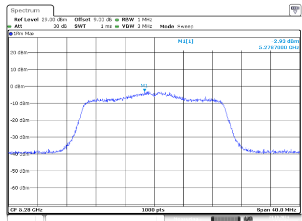
802.11ax20_5280MHz_RU_242/61_Chain 1
