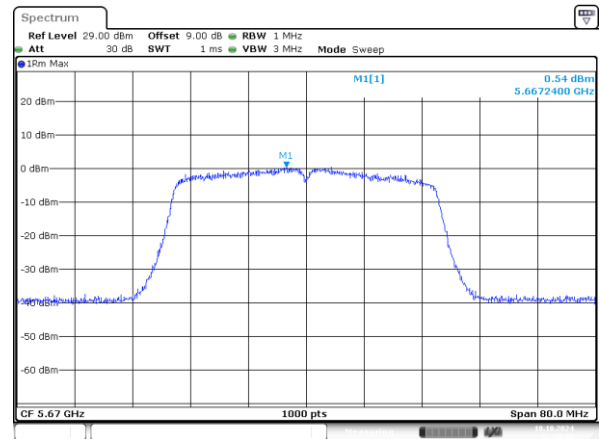
802.11n40_5670MHz_Chain 1
