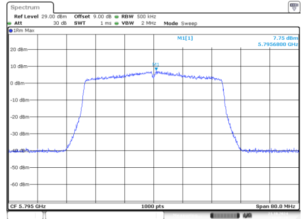
802.11ax40_5795MHz_RU_484/65_Chain 1
