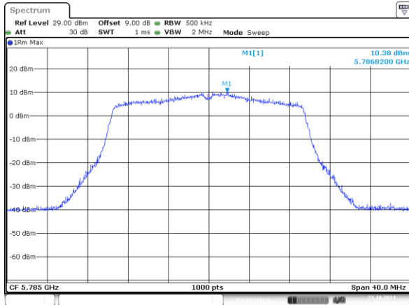
802.11ax20_5785MHz_RU_242/61_Chain 0
