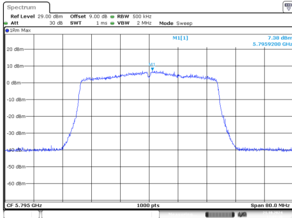
802.11ax40_5795MHz_RU_484/65_Chain 0
