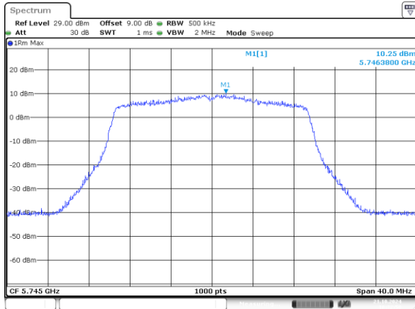
802.11ax20_5745MHz_RU_242/61_Chain 0
