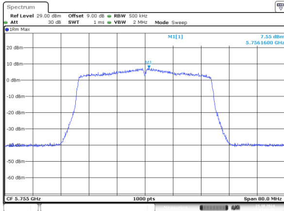
802.11ax40_5755MHz_RU_484/65_Chain 0
