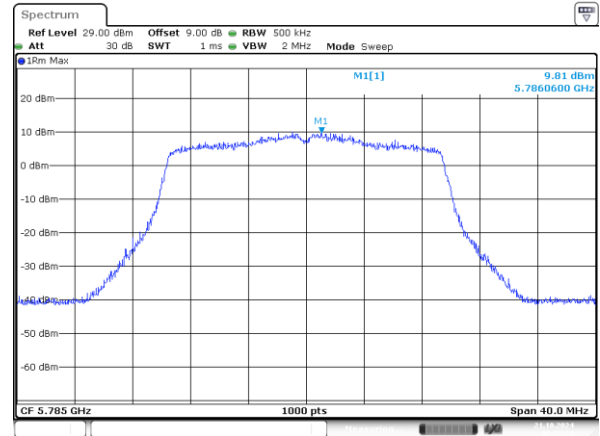
802.11ax20_5785MHz_RU_242/61_Chain 1
