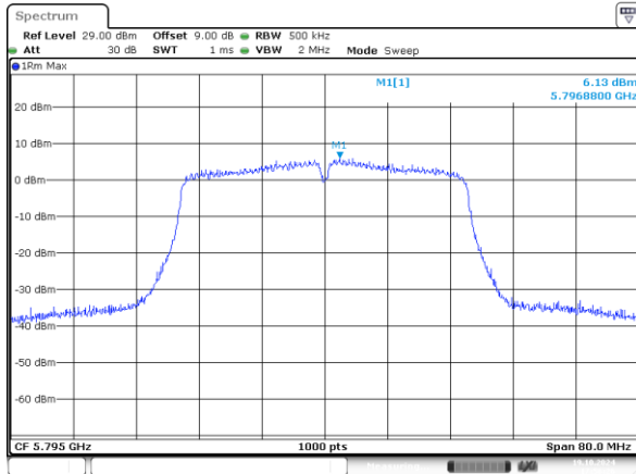
802.11n40_5795MHz_Chain 0
