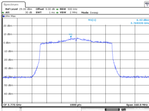
802.11ax80_5775MHz_RU_996/67_Chain 0
