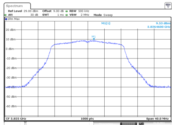
802.11n20_5825MHz_Chain 1
