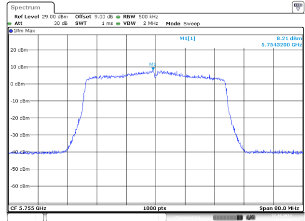
802.11ax40_5755MHz_RU_484/65_Chain 1
