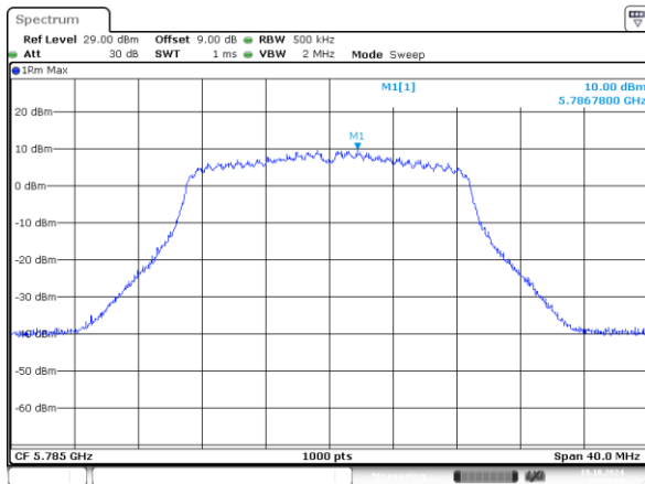
802.11n20_5785MHz_Chain 0
