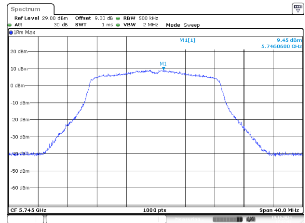
802.11n20_5745MHz_Chain 1
