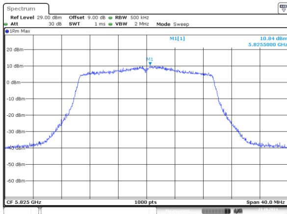
802.11ax20_5825MHz_RU_242/61_Chain 0
