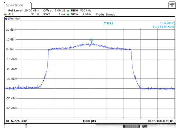
802.11ax80_5775MHz_RU_996/67_Chain 1
