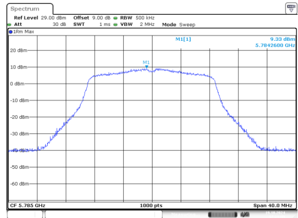
802.11n20_5785MHz_Chain 1
