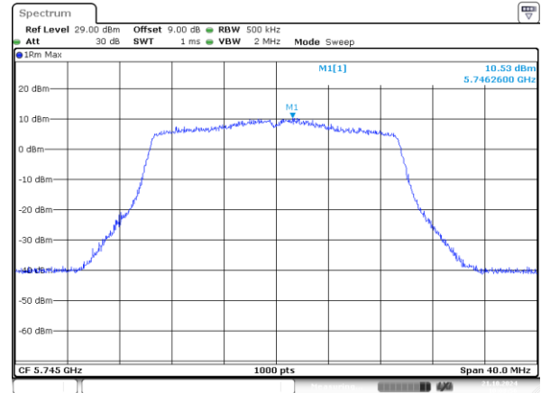
802.11ax20_5745MHz_RU_242/61_Chain 1
