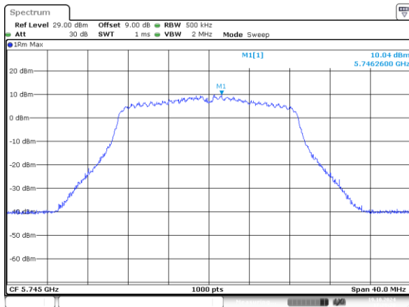
802.11n20_5745MHz_Chain 0
