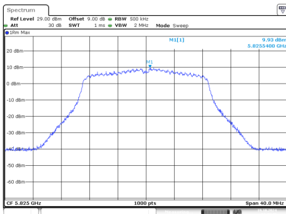
802.11n20_5825MHz_Chain 0
