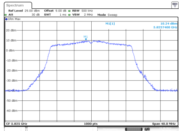
802.11ax20_5825MHz_RU_242/61_Chain 1
