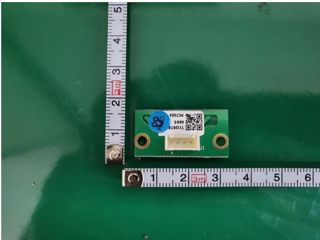
LED board - Rear
