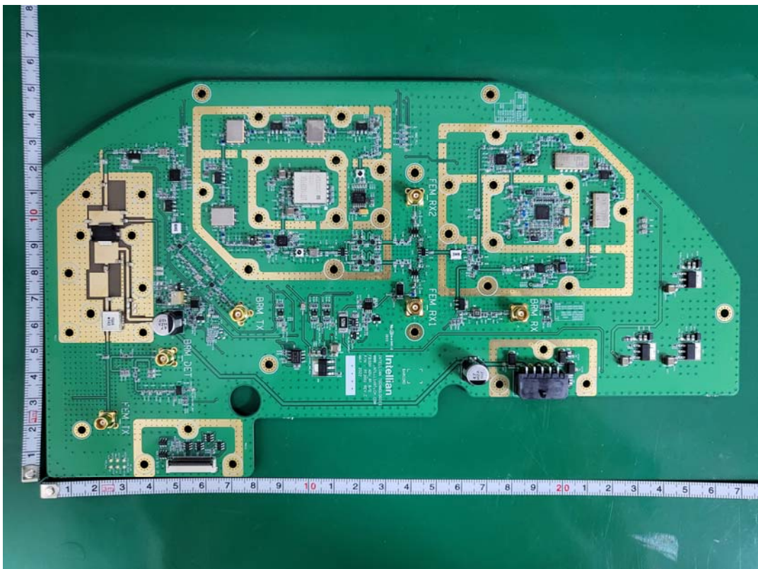
RF board - rear (shielding removed)
