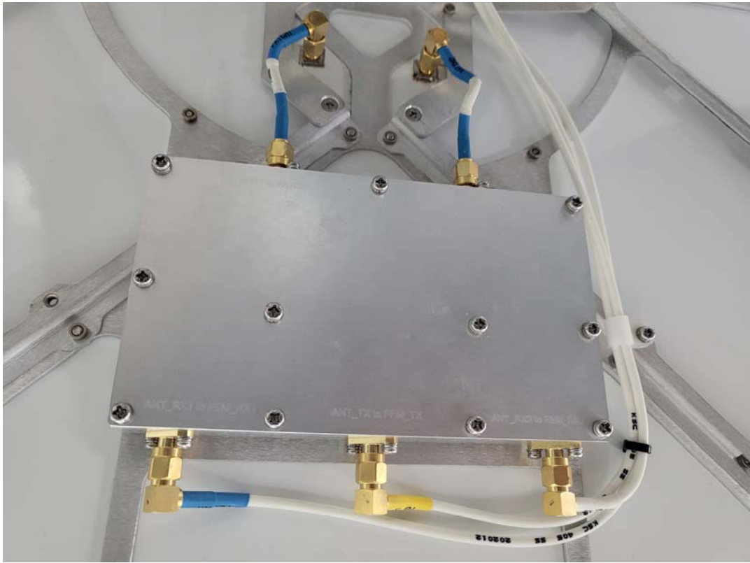
Connection between FEM and Patch antenna
