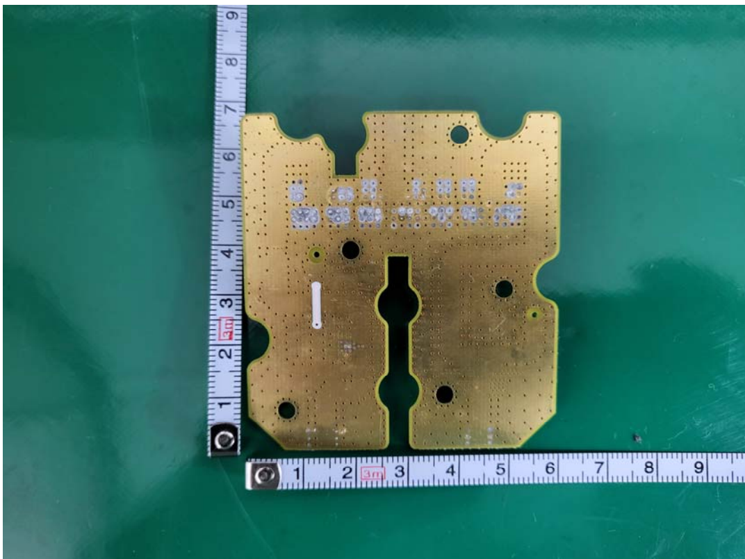
FEM (bottom) - rear
