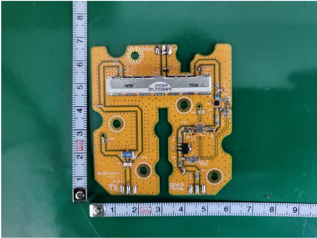
FEM (bottom) - front
