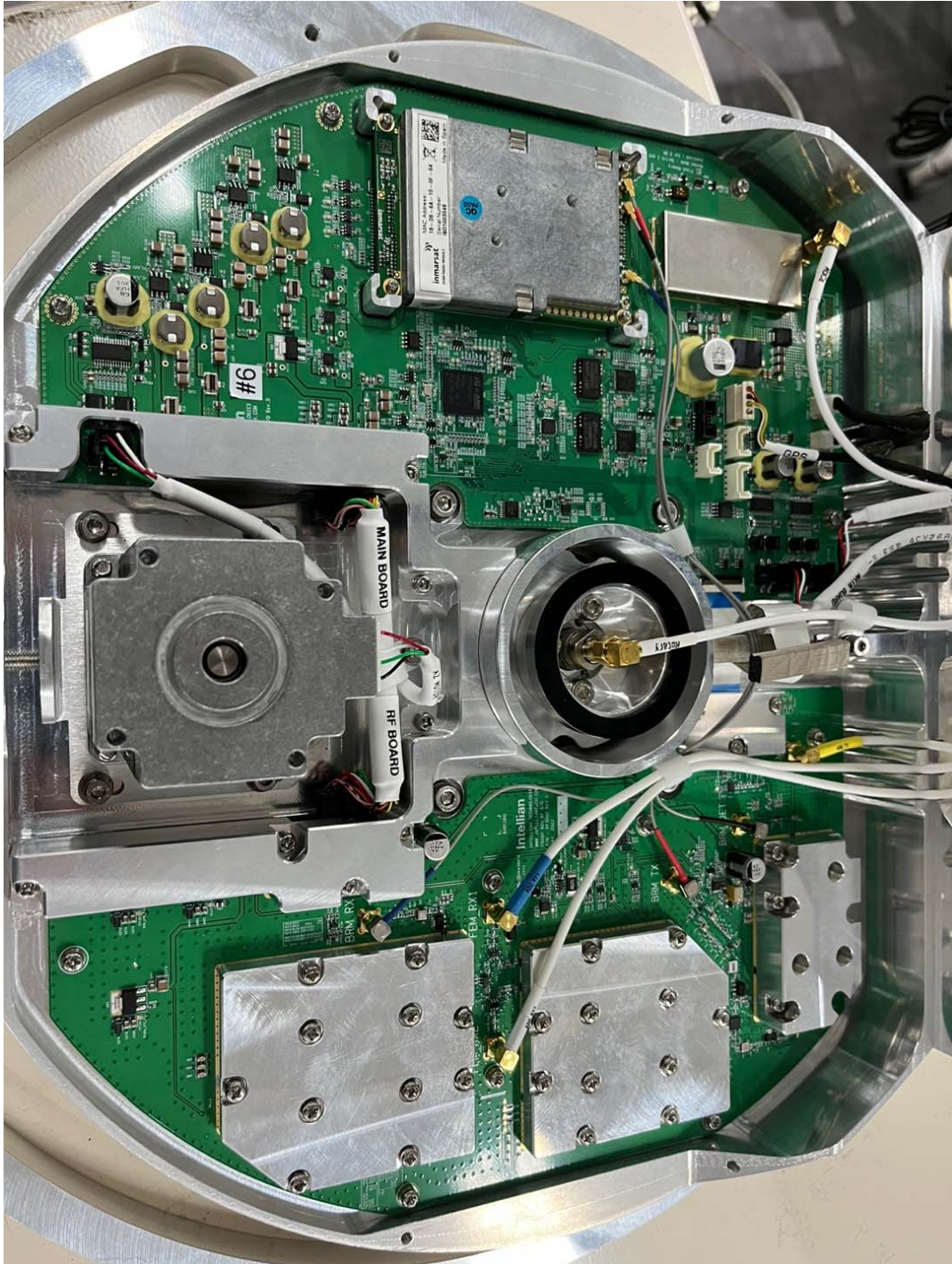
Cover opened (Mainboard, BRM, RF board)
