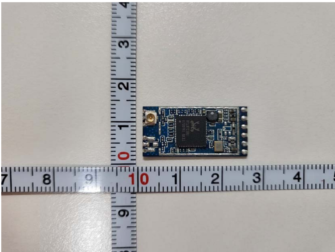
certified WiFi module - Front (shielding removed)
