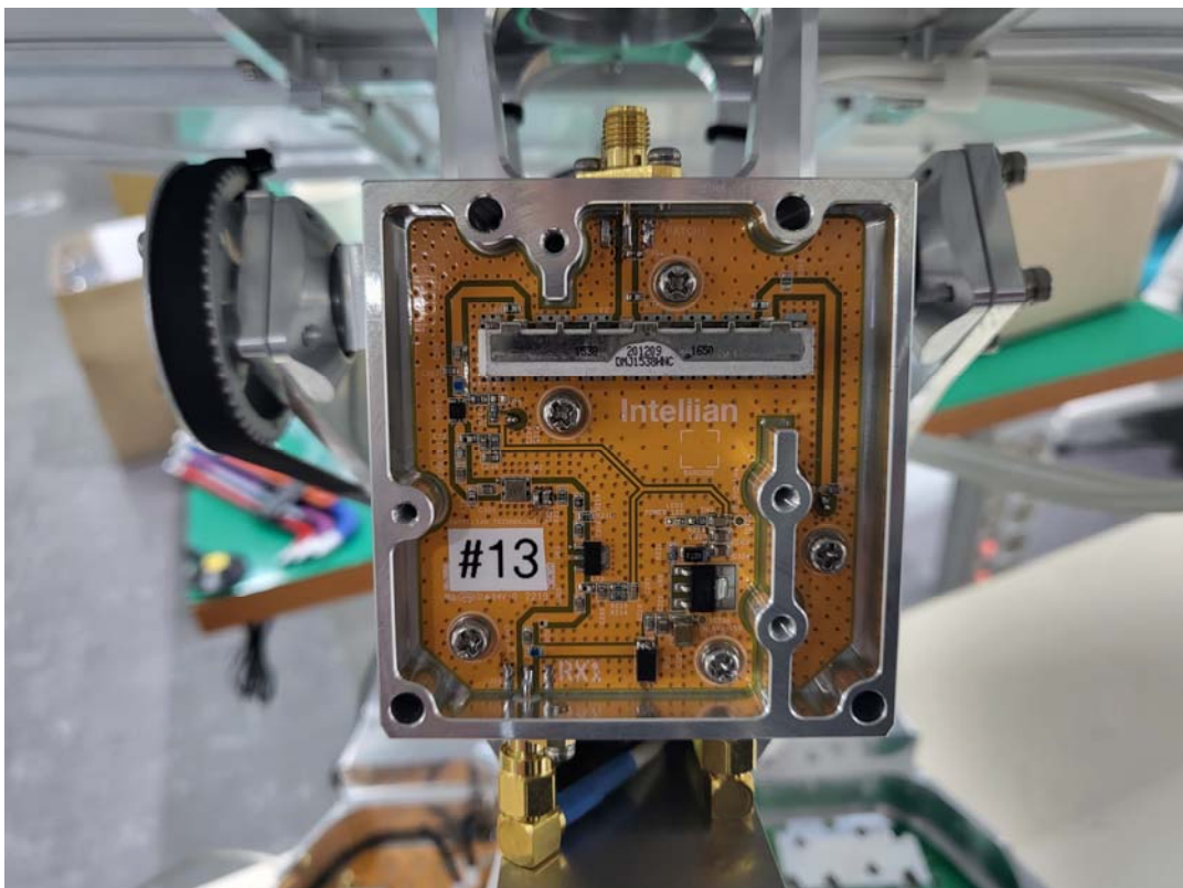
Cover opened (FEM)
