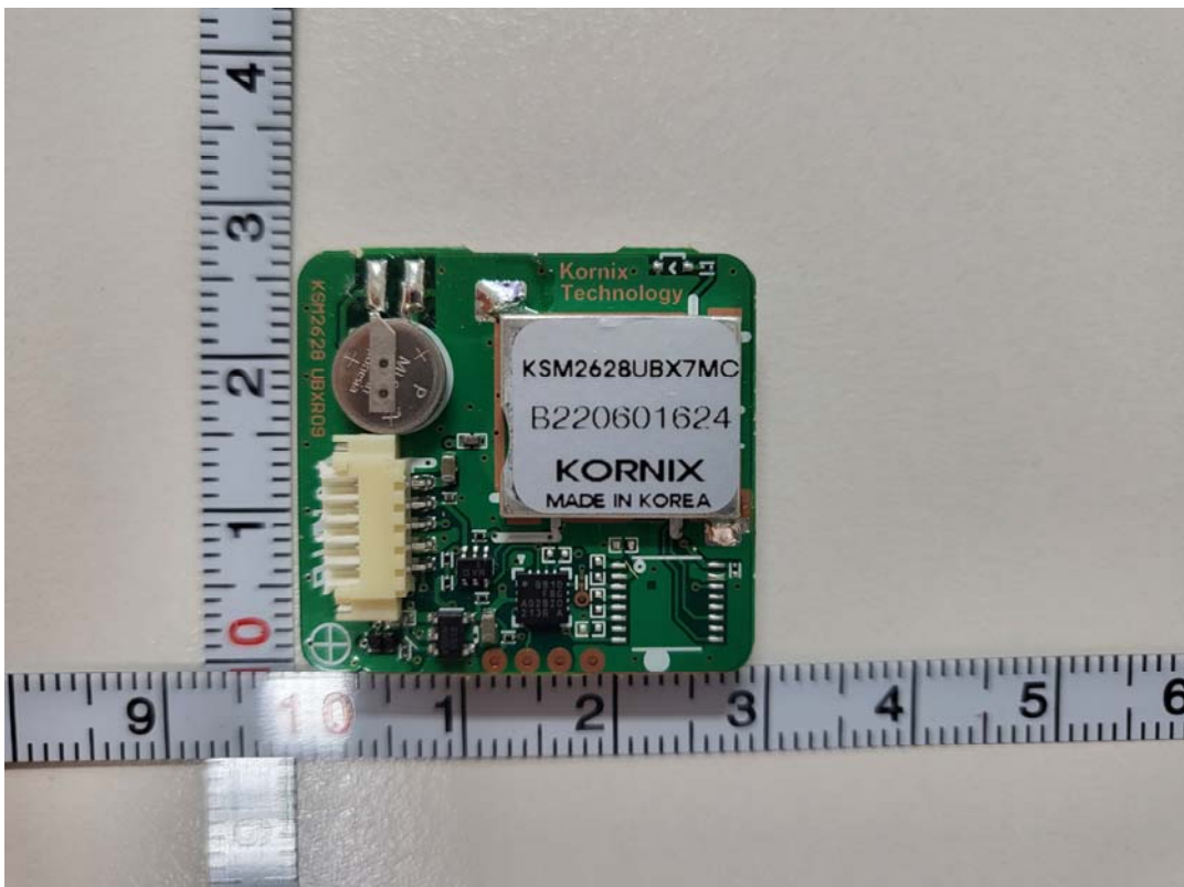
GPS Mainboard front (cover opened)
