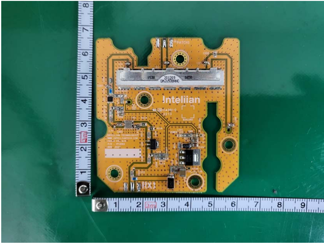
FEM (top) - front
