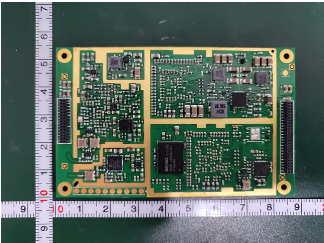
BRM - rear (shielding removed)
