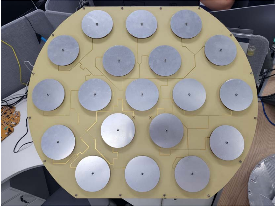
Cover opened (patch antenna)
