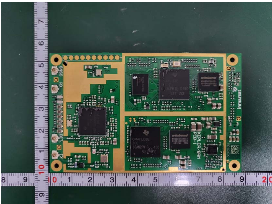
BRM - front (shielding removed)
