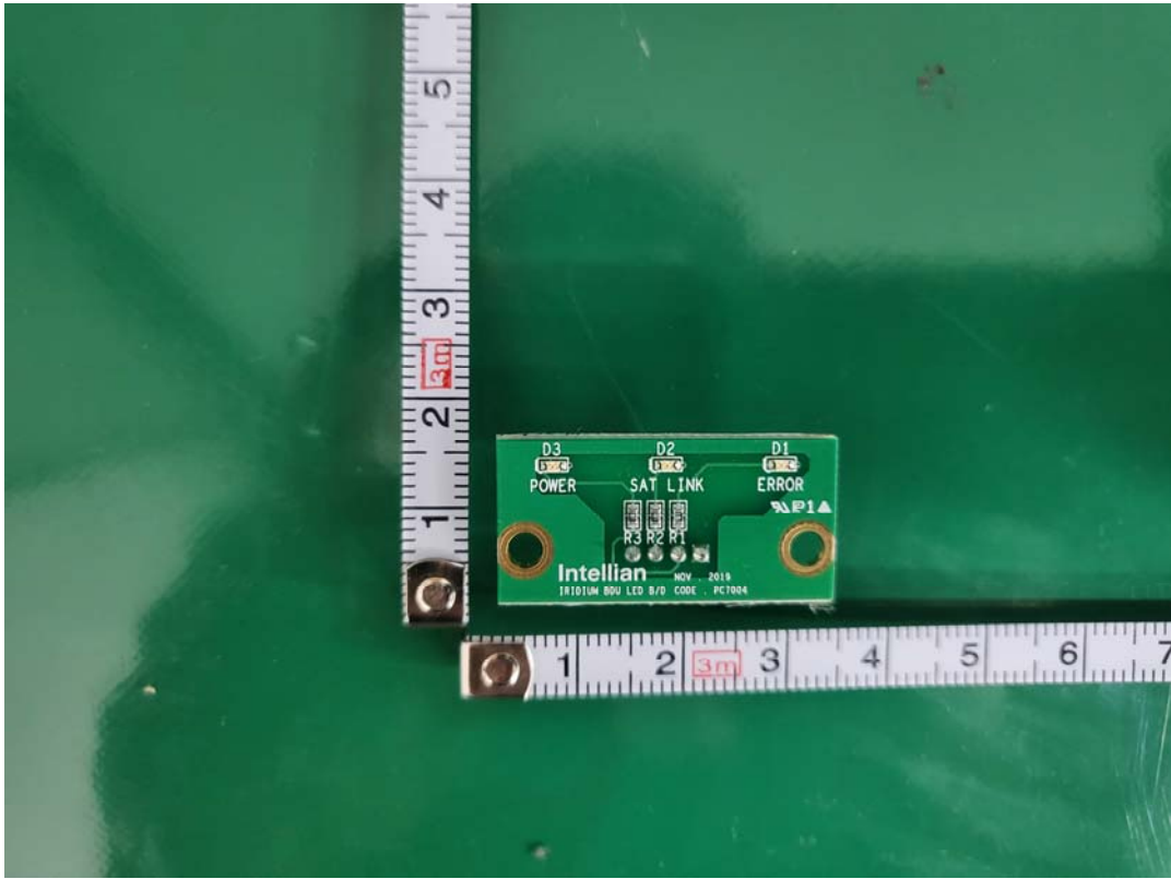
LED board - Front
