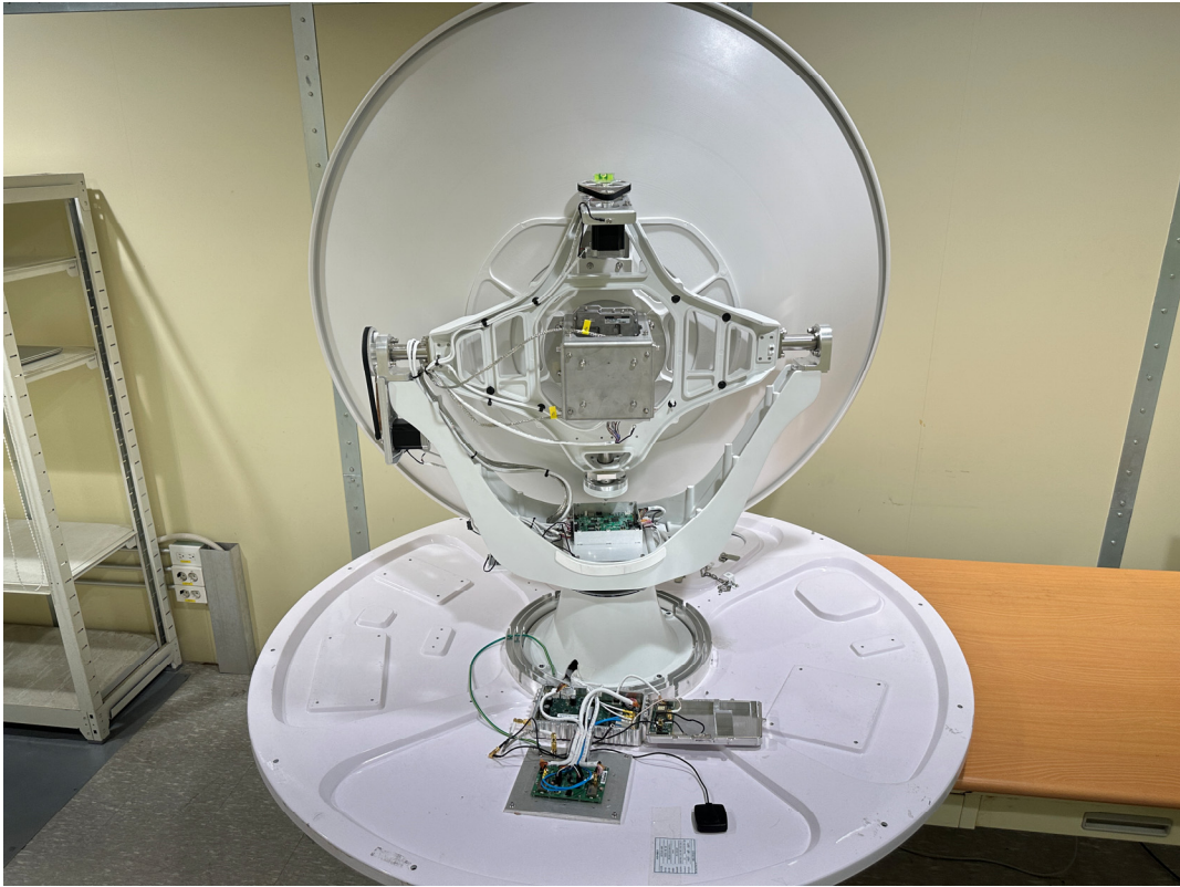
Primary Antenna Unit Cover opened (overall)
