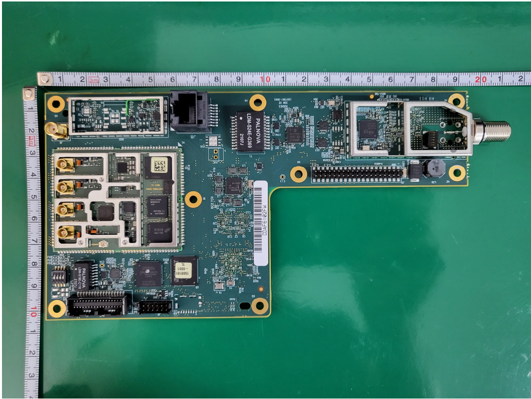
SSM Front(Shielding removed)
