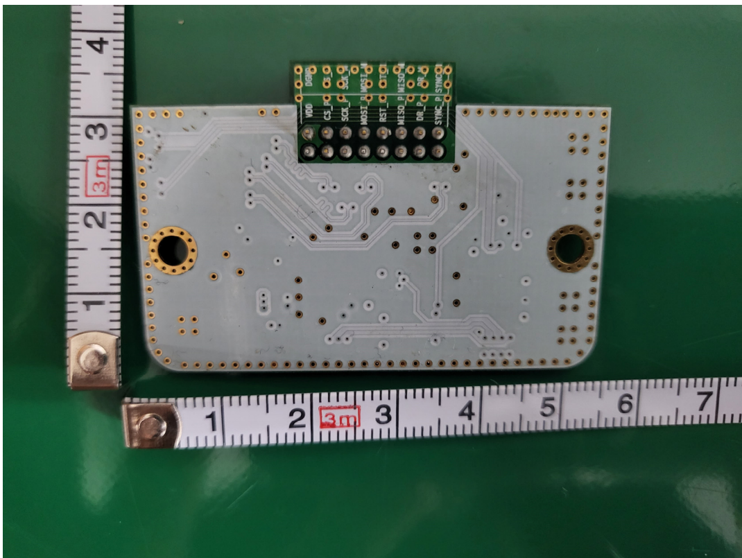
IMU Rear
