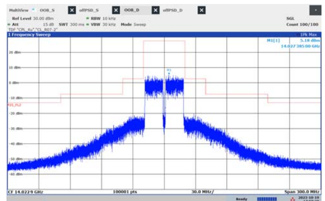
f_{\text{LOW}} (39.6 MHz, 16QAM)
