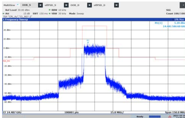
f_{\text{HIGH}} (19.8 MHz, 8PSK)
