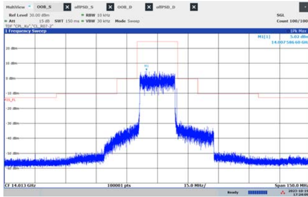
f_{\text{LOW}} (19.8 MHz, QPSK)
