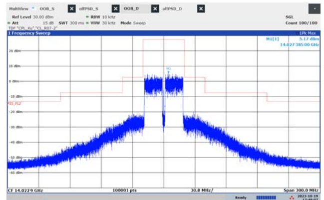
f_{\text{LOW}} (39.6 MHz, 8PSK)
