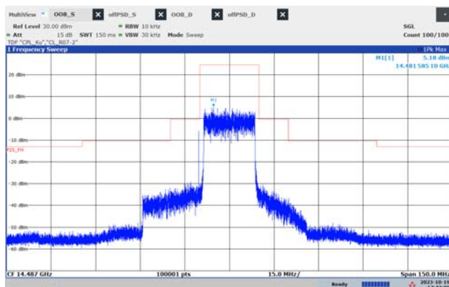
f_{\text{HIGH}} (19.8 MHz, 16QAM)
