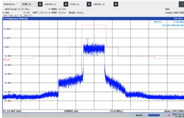
f_{\text{HIGH}} (19.8 MHz, QPSK)
