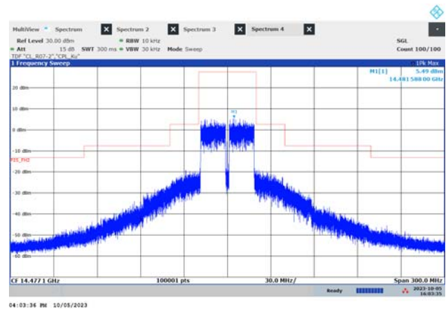
f_{\text{HIGH}} (39.6 MHz, 8PSK)
