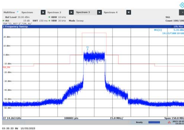
f_{\text{MID}} (19.8 MHz, 8PSK)
