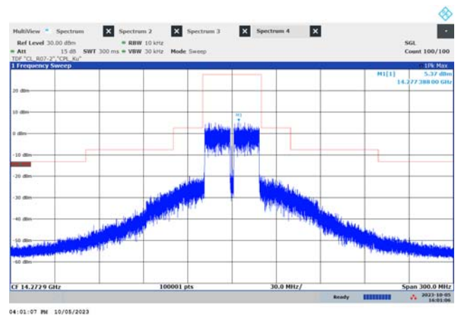
f_{\text{MID}} (39.6 MHz, 16QAM)
