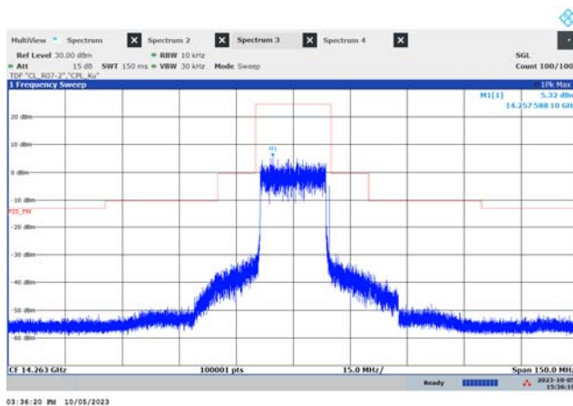
f_{\text{MID}} (19.8 MHz, 16QAM)
