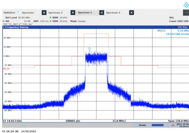
f_{\text{LOW}} (19.8 MHz, 8PSK)
