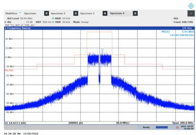
f_{\text{HIGH}} (39.6 MHz, 16QAM)
