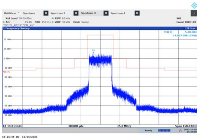
f_{\text{LOW}} (19.8 MHz, 16QAM)
