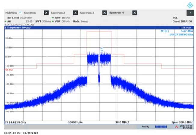
f_{\text{LOW}} (39.6 MHz, 16QAM)
