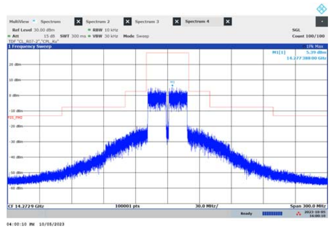
f_{\text{MID}} (39.6 MHz, 8PSK)
