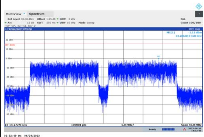
f_{\text{MID}} (39.6 MHz, 16QAM)
