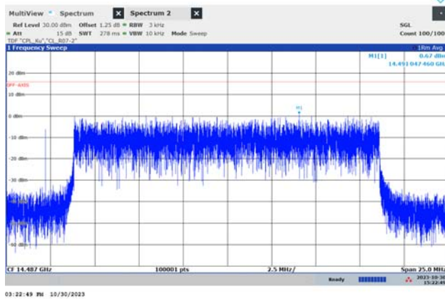
f_{\text{HIGH}} (19.8 MHz, QPSK)
