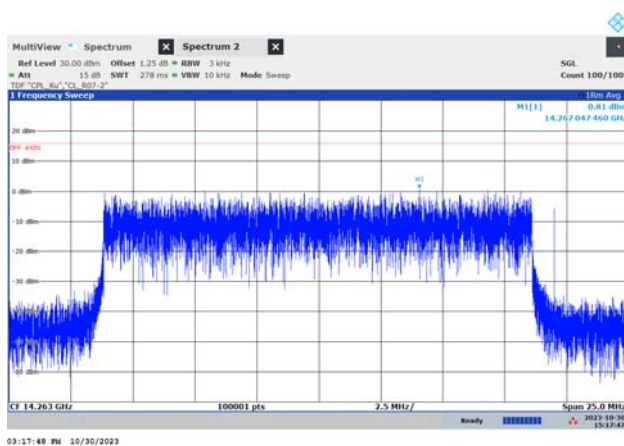
f_{\text{MID}} (19.8 MHz, 16QAM)
