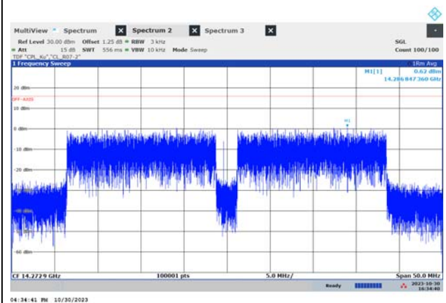
f_{\text{MID}} (39.6 MHz, 8PSK)
