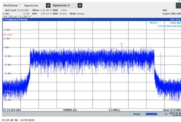
f_{\text{MID}} (19.8 MHz, QPSK)
