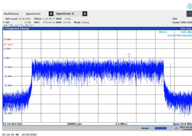
f_{\text{MID}} (19.8 MHz, 8PSK)
