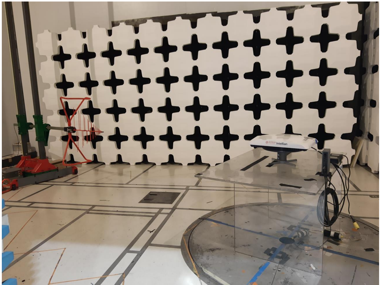
Photograph 3. RE Setup [30 MHz - 1GHz]
