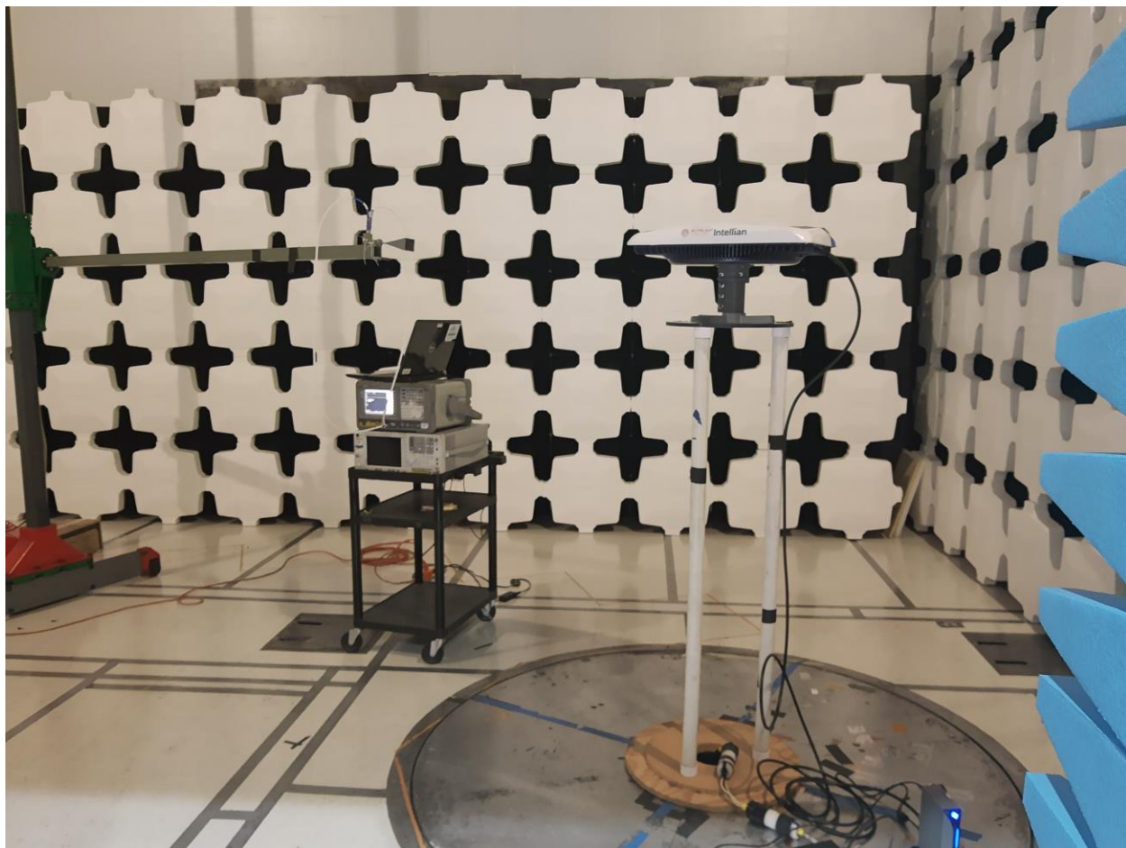
Photograph 6. RE Setup [40 GHz - 50 GHz]
