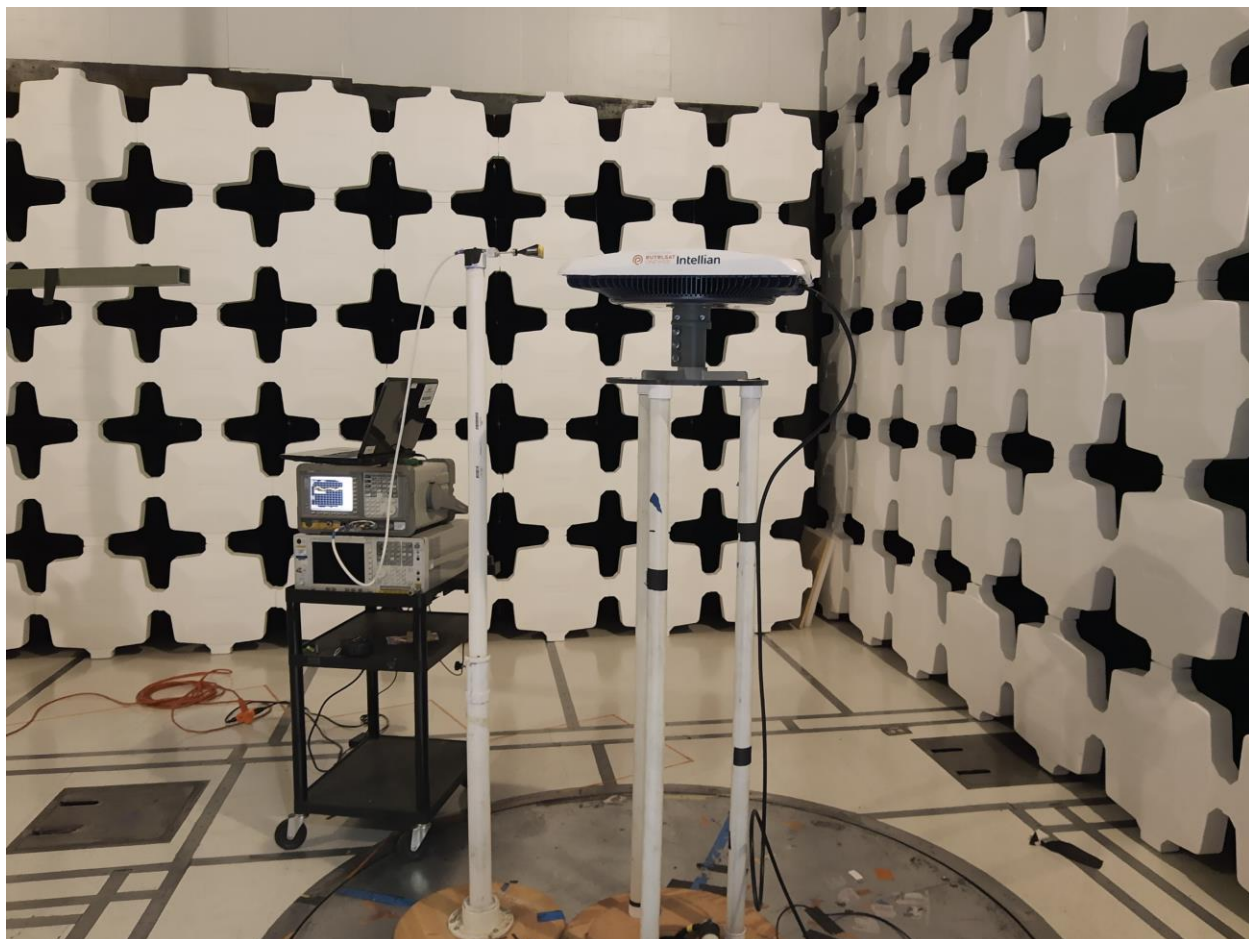
Photograph 7. RE Setup [50 GHz - 75 GHz]
