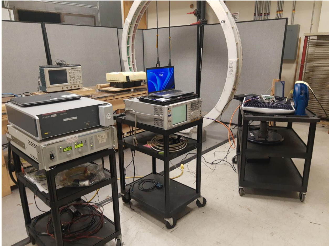
Photograph 2. Voltage Variation Frequency Stability Setup
