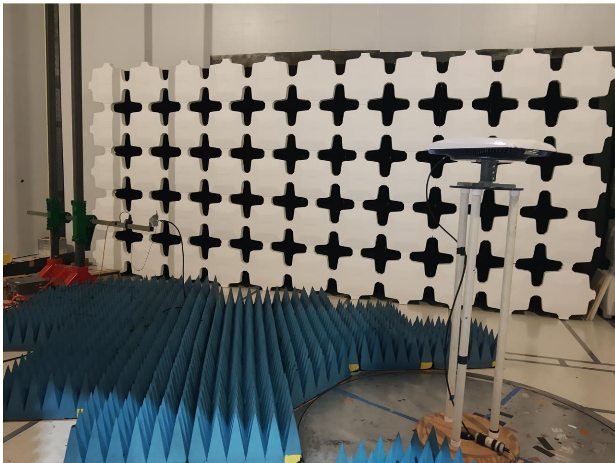
Photograph 5. RE Setup [18 GHz - 40 GHz]
