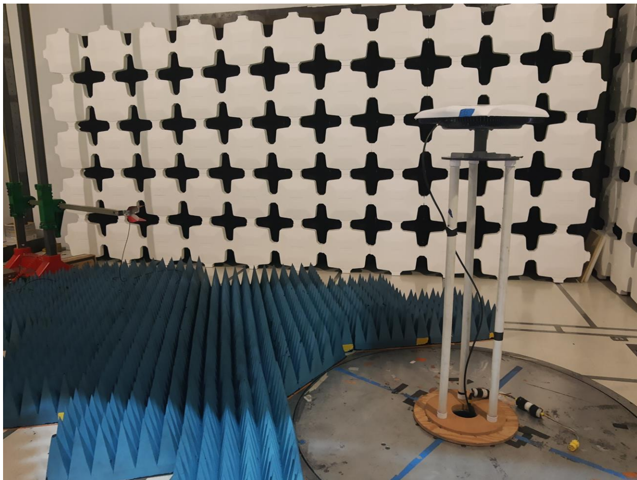
Photograph 4. RE Setup [1 GHz - 18 GHz]
