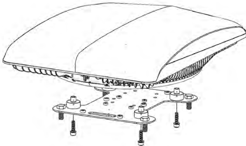
Figure 30: Attach Plate to Antenna
