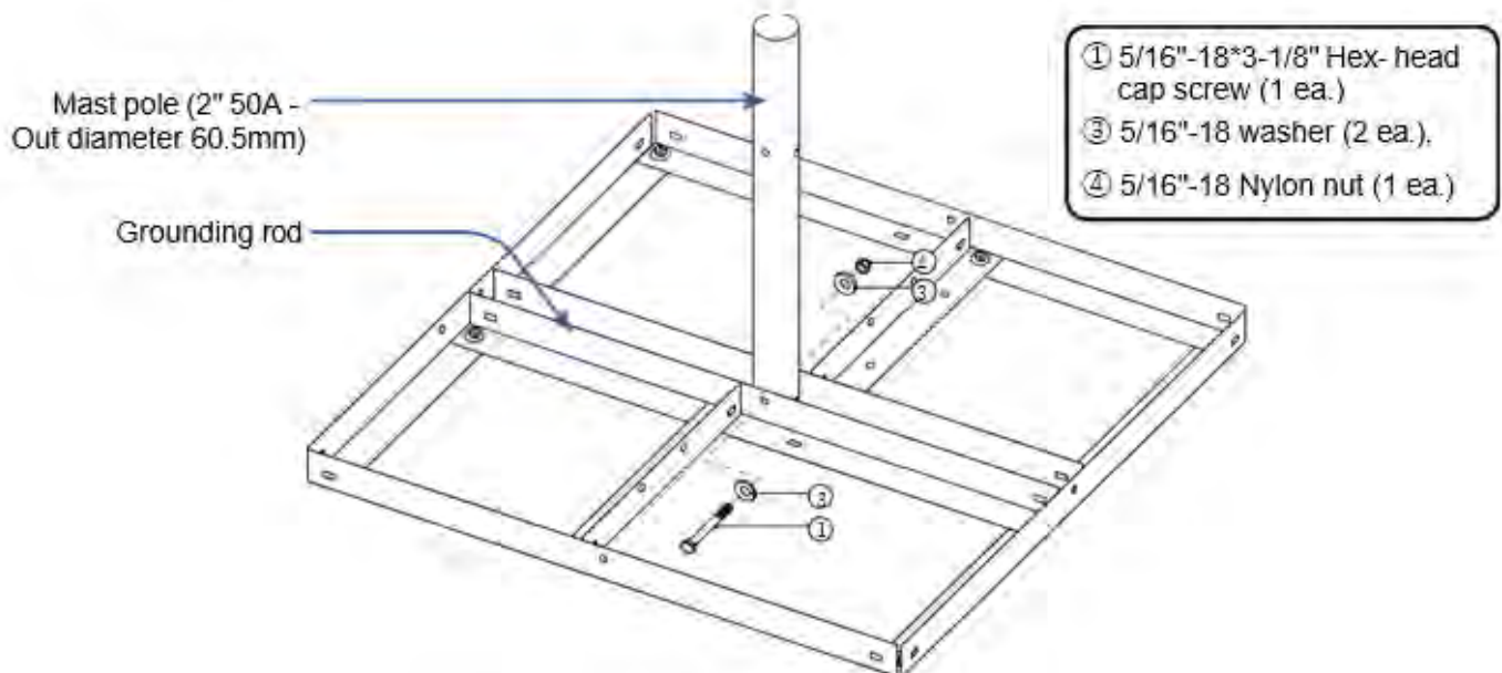
Figure 92: NPM Assemble Mast Pole
