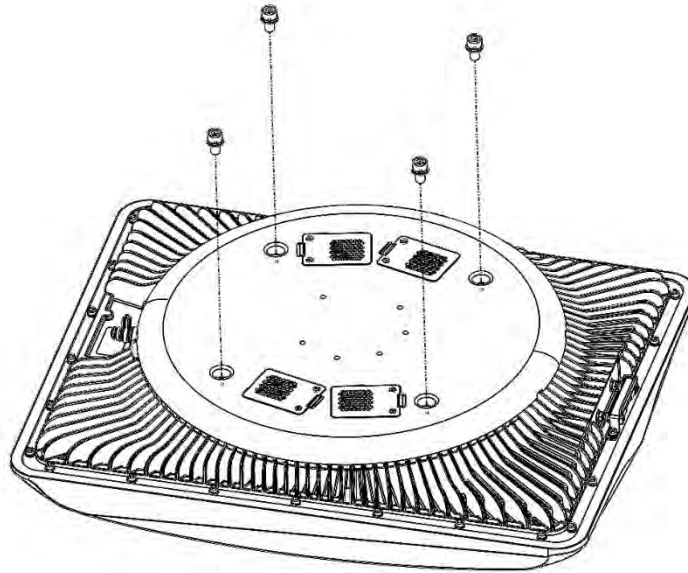
Figure 21: Mount Points
