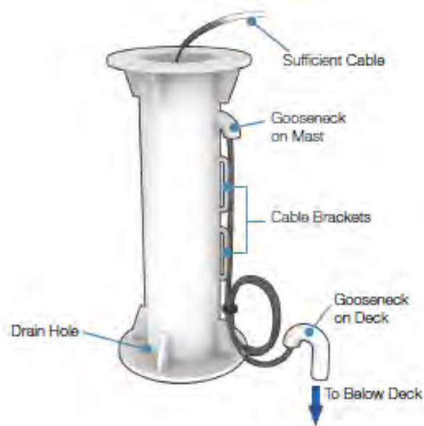
Figure 32: Routing Cable Through Inside of Mast
