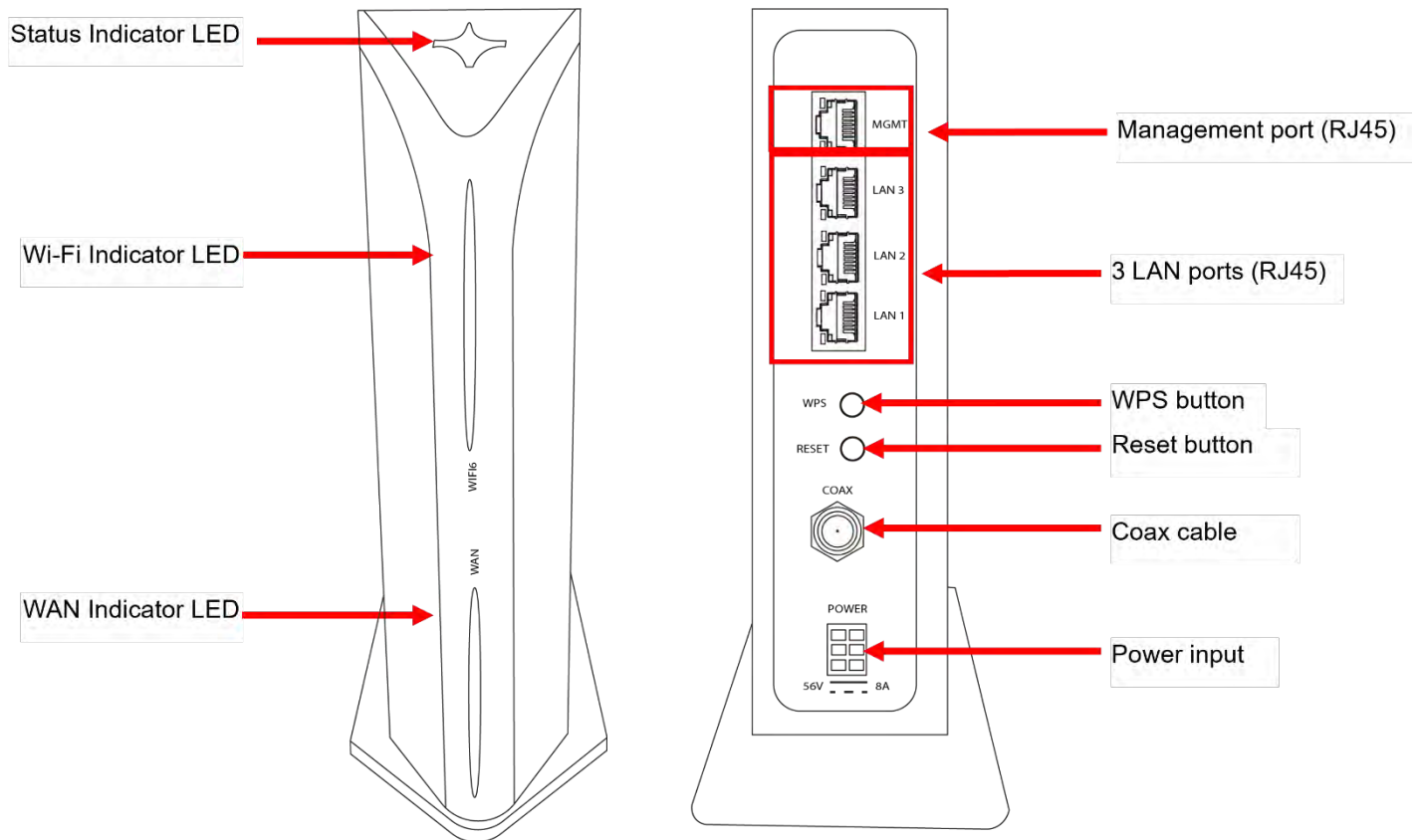
Figure 44: Front and Back Panels of CNX-WIFI
