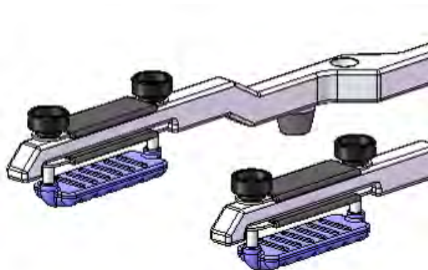
Figure 39: Install U Bolts
