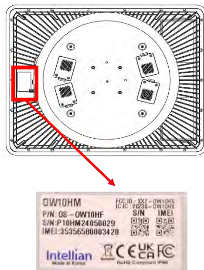
Figure 108:OW10Hx Label
