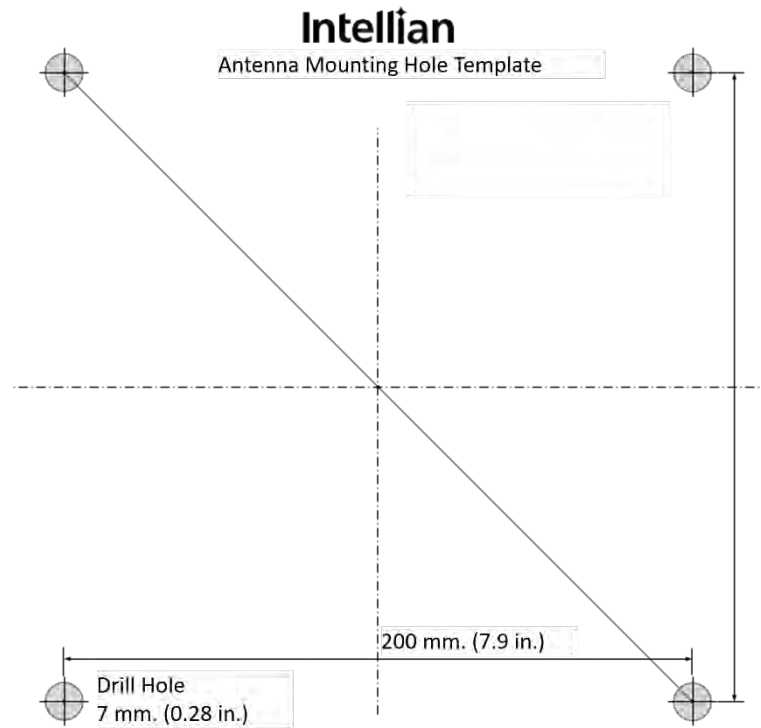
Figure 34: Hole Pattern
