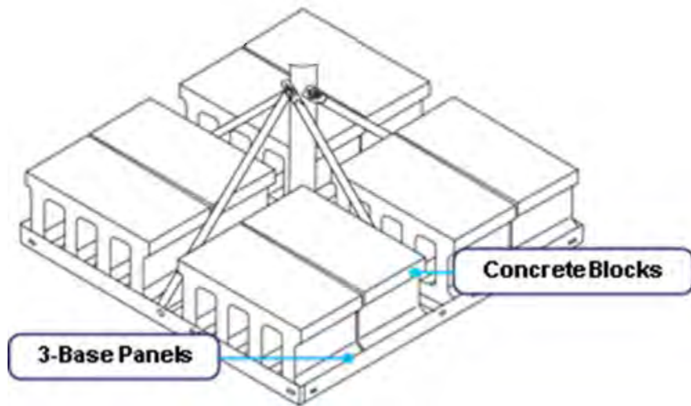
Figure 96: Concrete Blocks Arrangement
