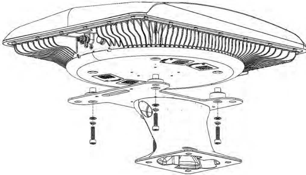
Figure 27: Attach Antenna to Plate
