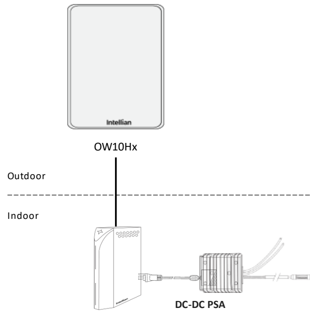
Figure 4: DC Power with CNX-WIFI
