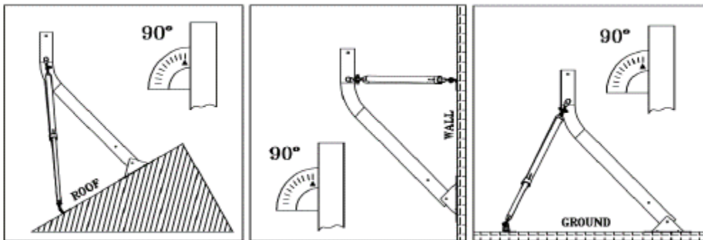
Figure 99: Completed Installation Positions
