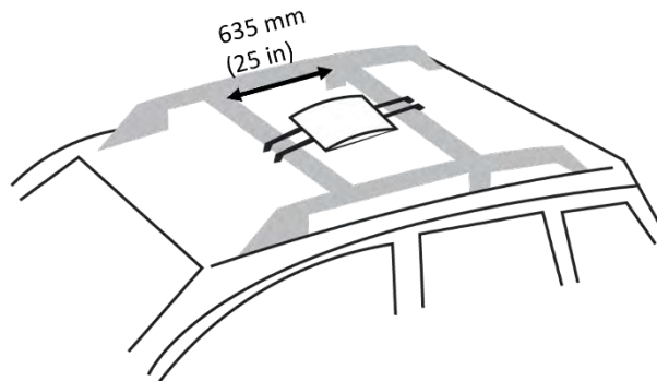
Figure 38: Antenna on Crossbars
