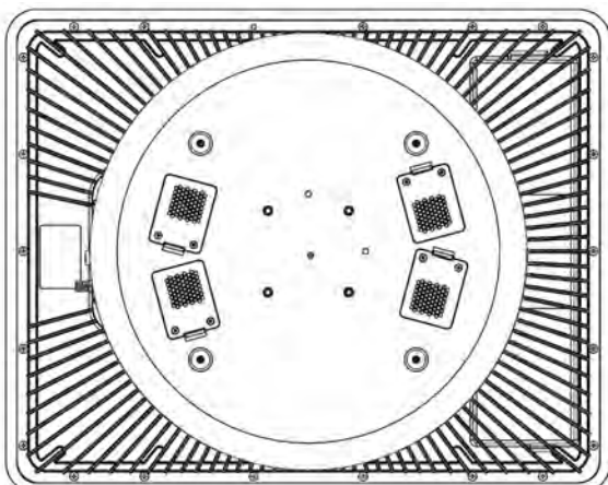
Figure 113: Fans Location
