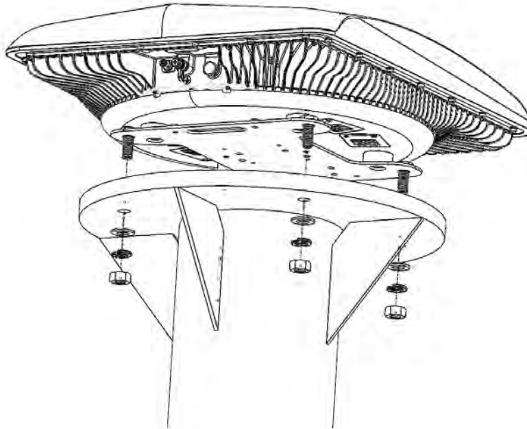
Figure 31: Attach Antenna to Mast
