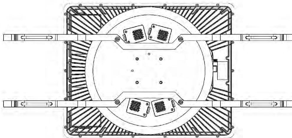
Figure 37: Attach Antenna to Mount Adapter
