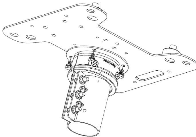
Figure 22: Attach Adjustable Mount Adapter to Maritime Mount Adapter Plate
