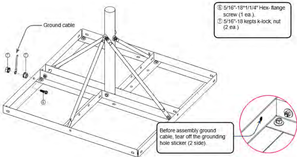
Figure 95: NPM Ground Cable
