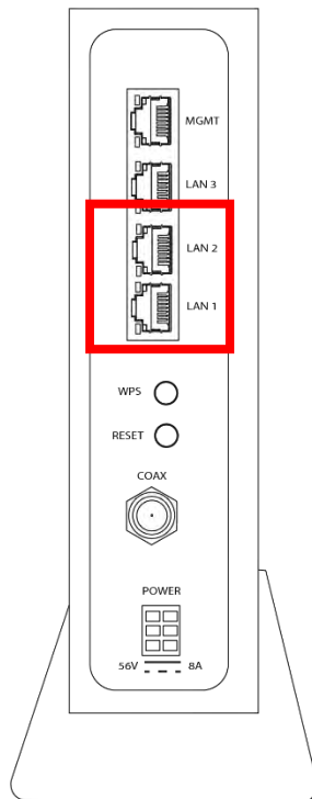
Figure 55: LAN1 and LAN2 ports
