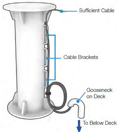
Figure 33: Routing Cable Through Outside of Mast
