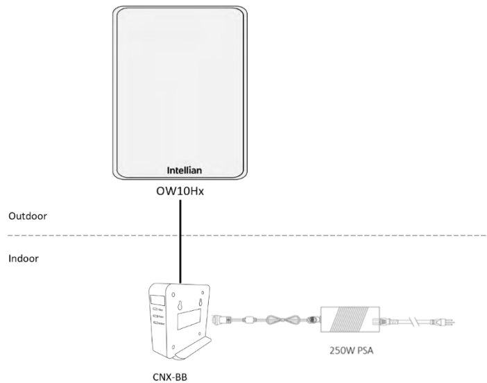
Figure 3: AC Power with CNX-BB
