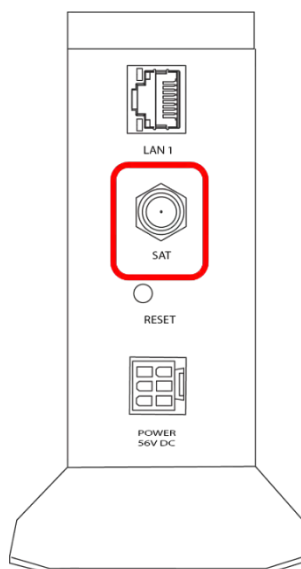
Figure 58: Connect Coax Cable
