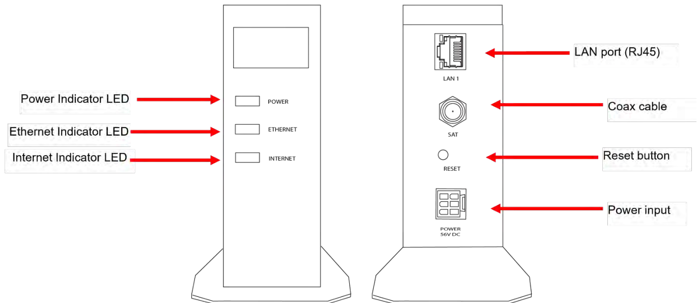
Figure 60: Front and Back Panels of CNX-BB
