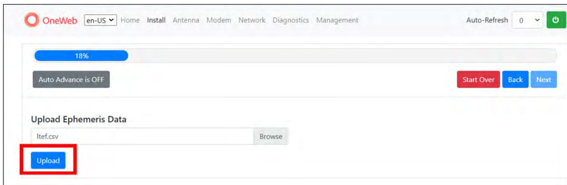
Figure 74: Upload Ephemeris File
