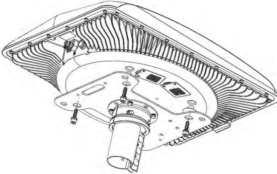
Figure 23: Attach Antenna to Mount
