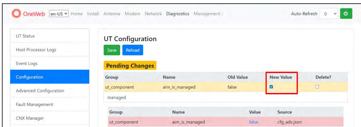
Figure 80: Pending Changes Updates
