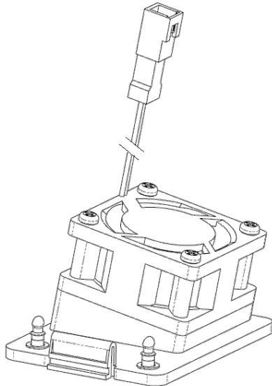
Figure 115: Disconnect Fan
