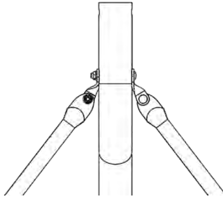
Figure 98: Attach Mast and Adjustment Struts
