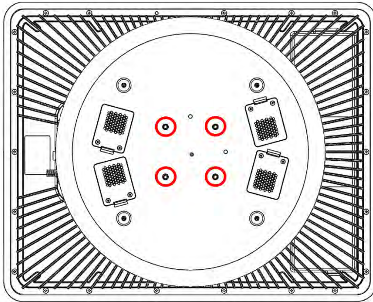
Figure 15: Attach Adjustable Mount Adapter
