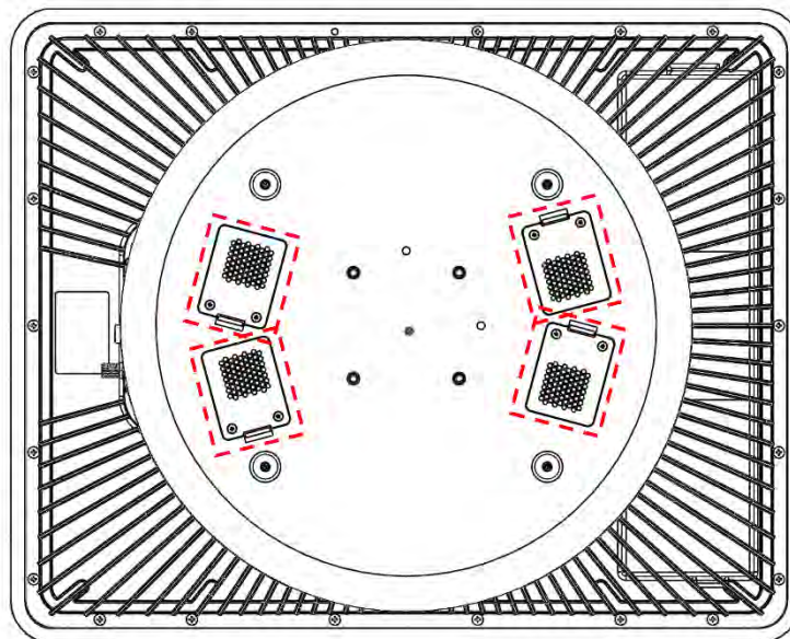
Figure 24: Antenna Fans
