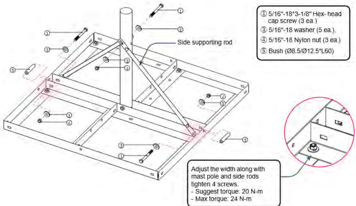
Figure 93: NPM Supporting Rods and Bolts
