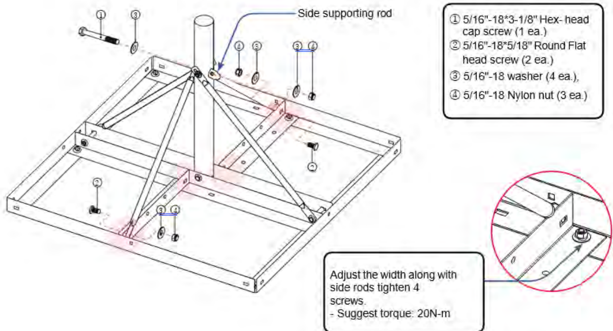
Figure 94: NPM Supporting Rods
