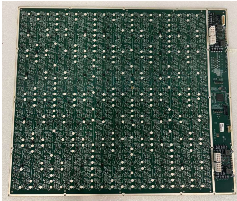
ACU2P4: (Fron and Back Side):
