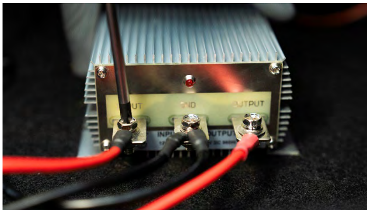
Figure 57: DC-DC PSA
