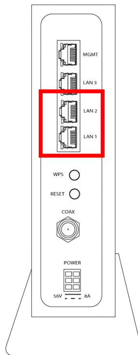
Figure 53: LAN1 and LAN2 ports
