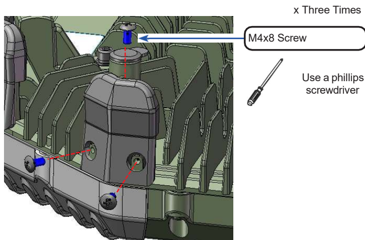
Figure 32: Attaching the Side Bumpers
