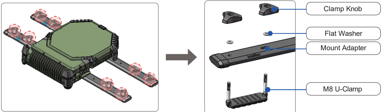
Figure 20: Loosening Clamp Knobs of the Mount Adapter
