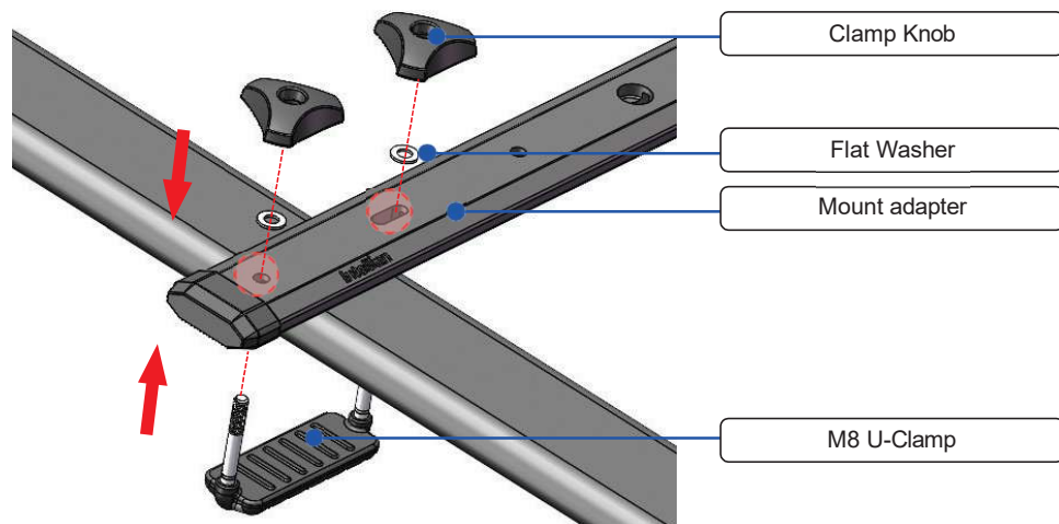
Figure 21: Assembling the M8 U-Clamp
