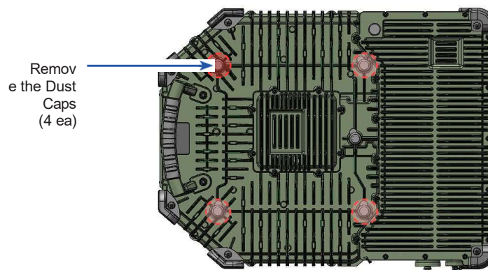
Figure 17: Removing the Dust Caps
