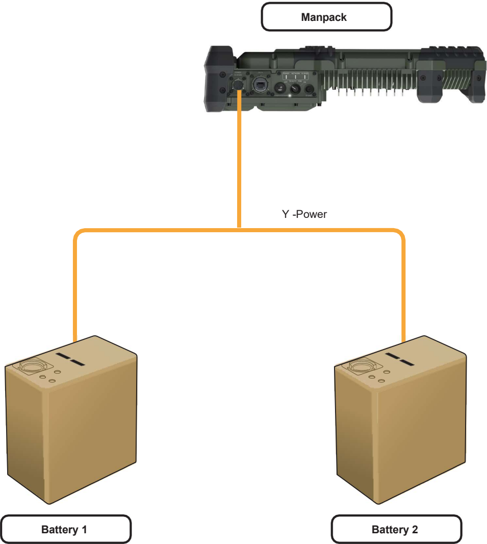
Figure 24: Connecting Battery Y Power Cable
