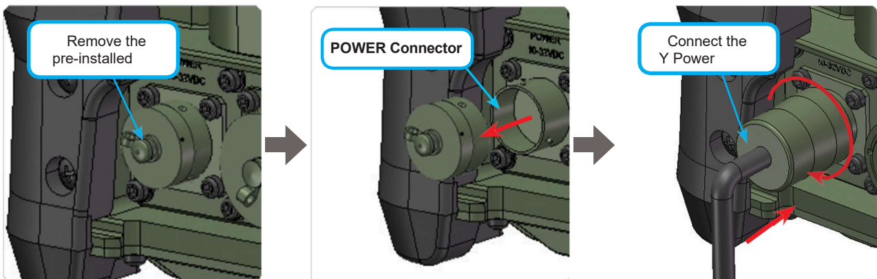
Figure 25: Connecting PSA Cable
