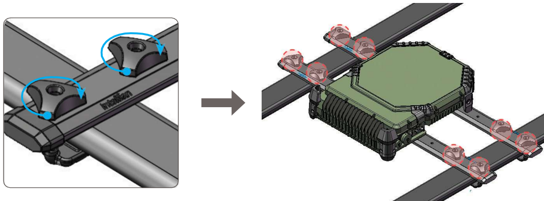
Figure 22: Fixing the Mount Adapter on the Cross Bar
