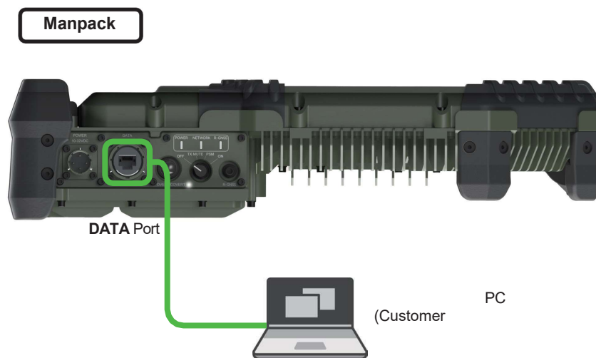
Figure 29: DATA Port Connection
