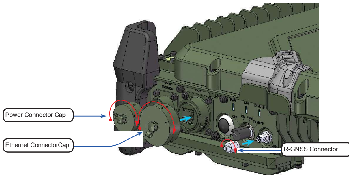
Figure 35: Installing the Connector Caps on the Connectors
