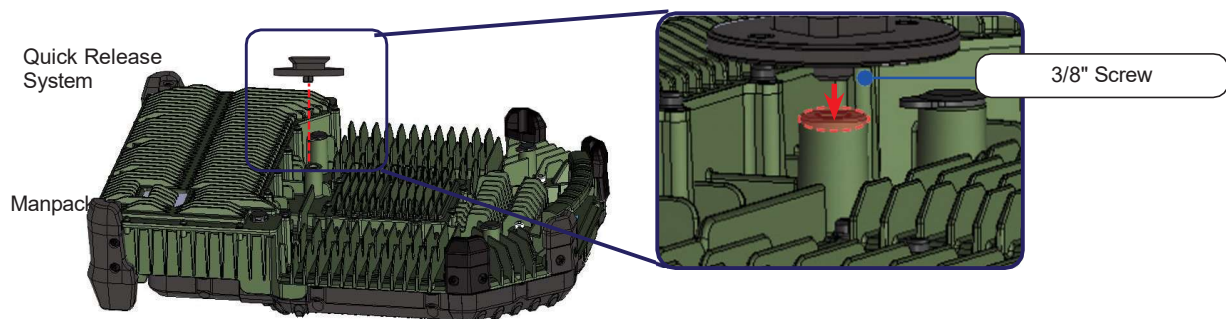
Figure 8: Inserting the 3/8" Screw of the Quick Release System
