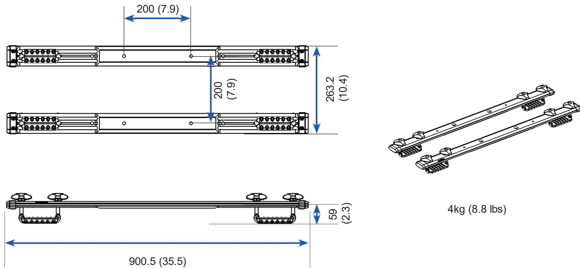
Figure 16: Land Mobile Mount Adapter Dimension
