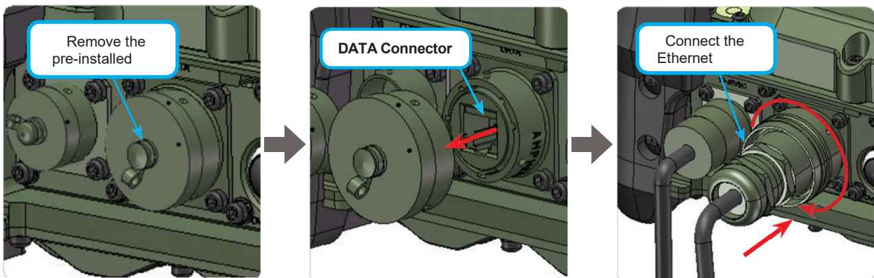
Figure 27: Connecting Ethernet Cable
