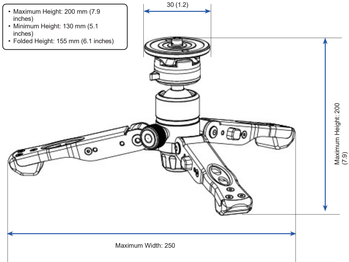
Figure 4: Mini-Tripod Dimensions
