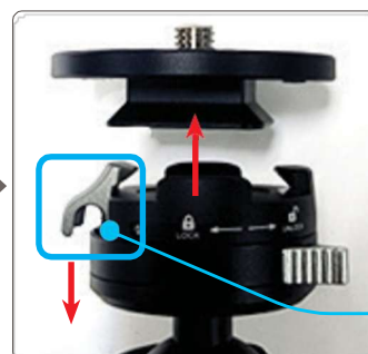
Figure 6: Detaching the Quick Release System
