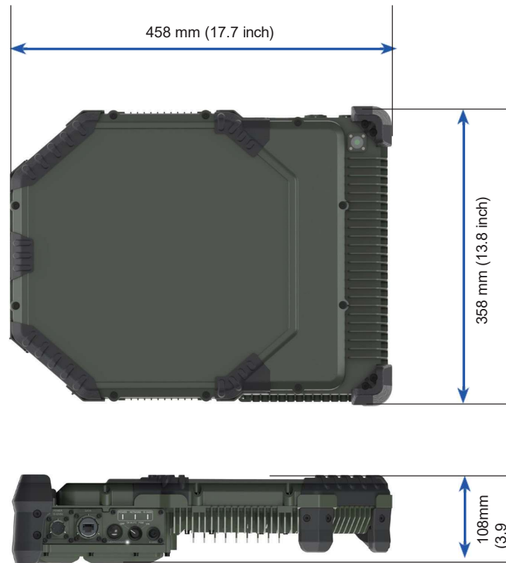
Figure 3: Manpack Dimension
