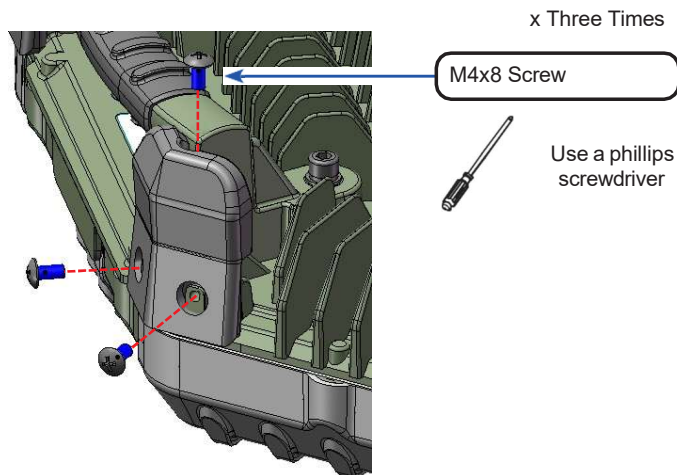
Figure 31: Attaching the Front Bumpers
