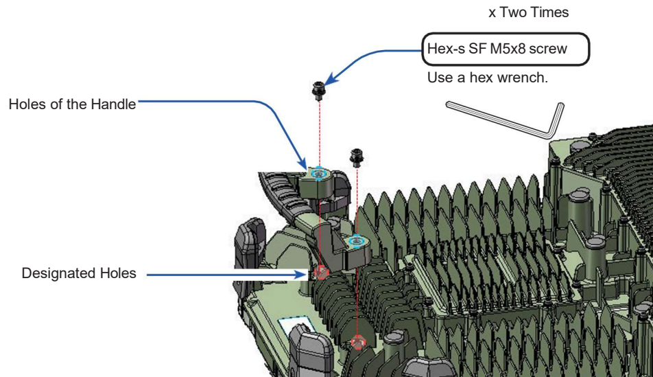
Figure 34: Installing the Handles on the Manpack
