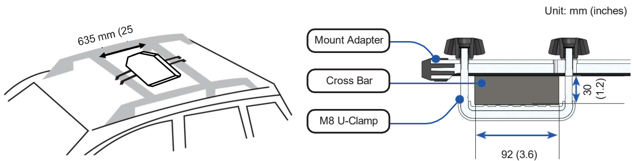
Figure 19: Conditions for crossbars suitable for land mobile mount installation
