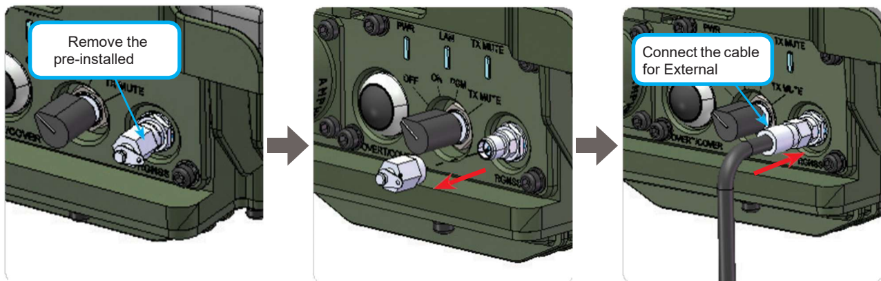
Figure 28: Connecting the SMA connector of the external GNSS cable to the GNSS connector
