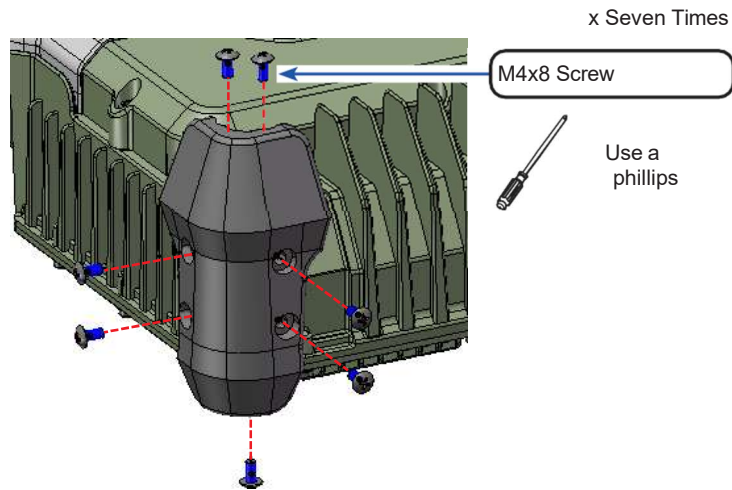
Figure 33: Attaching the Rear Bumpers
