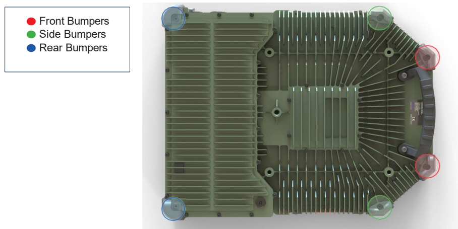
Figure 30: Positions of Bumpers
