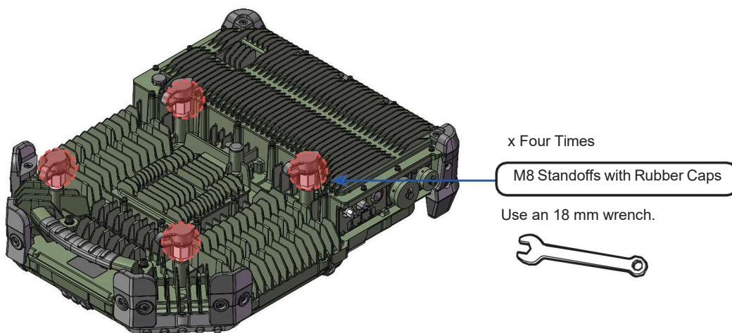
Figure 18: Attaching the M8 Rubber Feet Plugs
