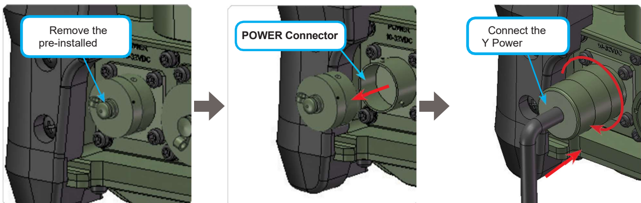
Figure 23: Connecting Power Cable
