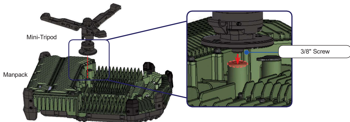
Figure 12: Inserting the 3/8" Screw of the Mini-Tripod
