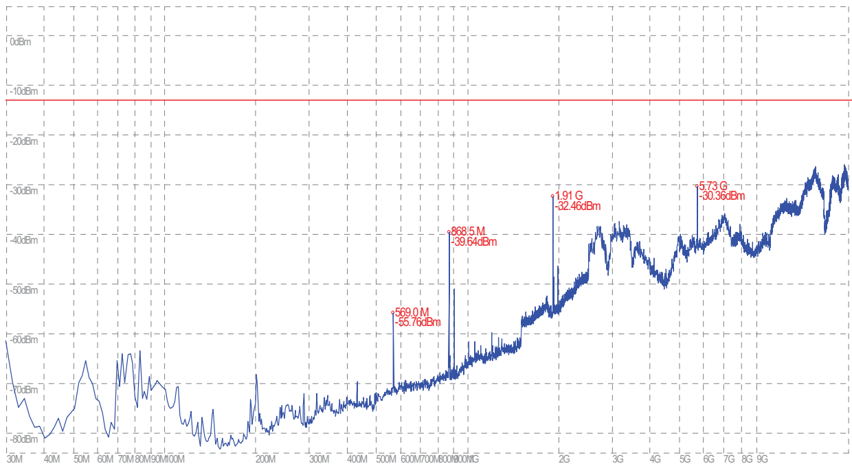
(Plot F.2: GSM 1900MHz Channel = 810, Test Antenna Vertical)
